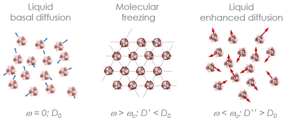
Fig. 4. Phase behaviour of rotating ATP synthases in lipid membranes. In the absence of rotation, \omega = 0 , ATP synthases freely diffuse within the membrane with a diffusion coefficient D_0 . At high rotational velocities ( \omega > \omega_c ) proteins are kinetically arrested ( D' \approx 0 ). At low spin velocities, protein diffusion is enhanced ( D'' > D_0 ). The spin velocity can be tuned with the ATP concentration and the critical angular velocity can be modified by changing the viscoelastic properties of the embedding lipid membrane and the protein packing.
