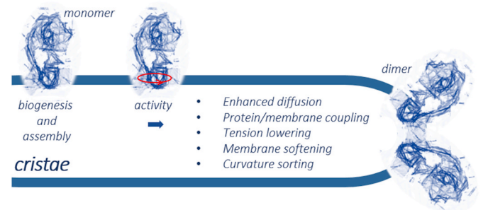
Fig. 5. Monomeric ATP synthases are synthesized and assembled within cristae [124]. Protein activity triggers membrane softening and tension lowering [91]. The mechanical adaptation might facilitate membrane tubulation. In addition, membrane softening might be also responsible for an enhanced protein-to-curvature coupling thus results into curvature sorting. The transport properties of ATP synthase can be regulated in a framework containing a set of rotating ATP synthases.
