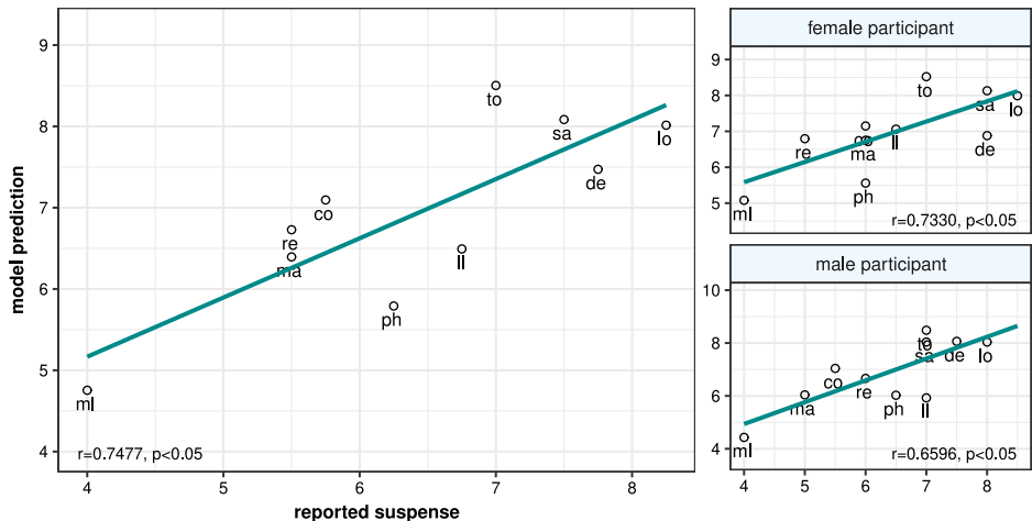
Fig. 5. Correlation between reported suspense for the last slides and the return value of the predictive model.
