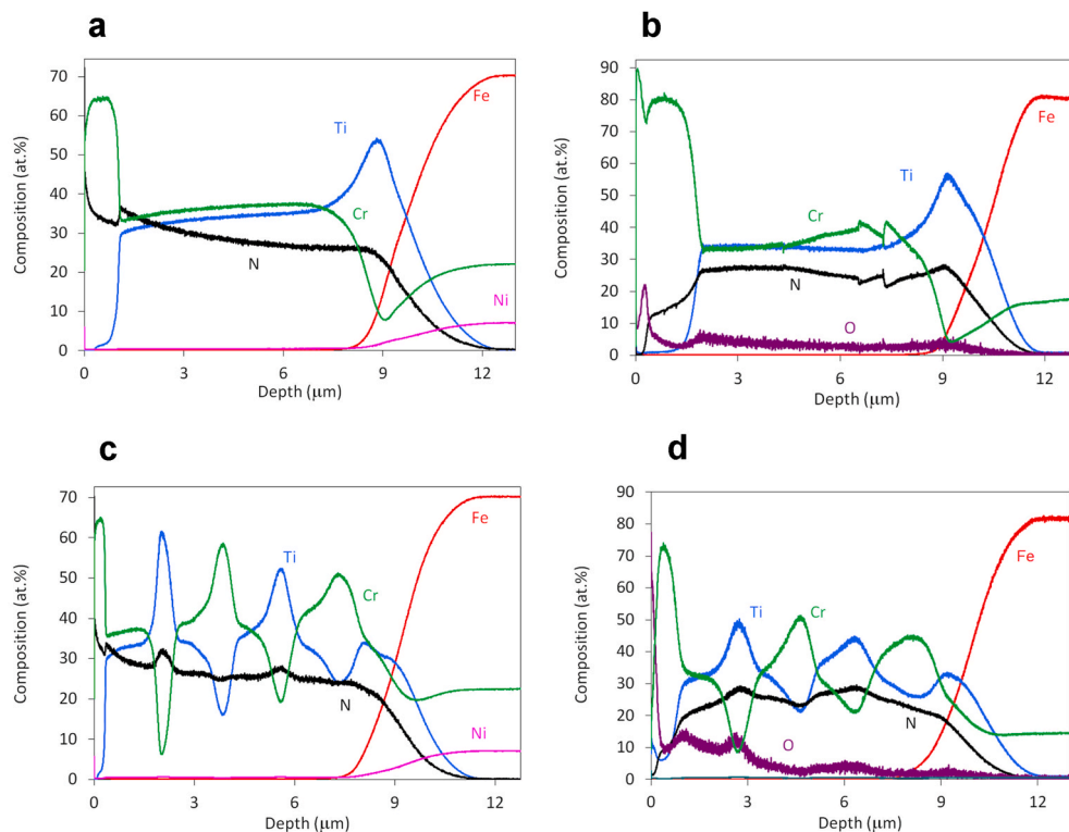
Fig. 9. Compositional depth profiles by GDOES of as-deposited and oxidized at 650 °C to 2000 h in 100% steam atmosphere: a) and b) CrN/CrTiN/TiN three-layer coating, c) and d) CrN/CrTiN/TiN multi-layer coating.
