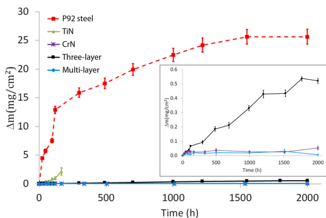
Fig. 4. Mass change per unit area versus time of the substrate P92 and the coatings under study up to 2000 h at 650 °C in 100% steam atmosphere. The inset shows an enlargement of the part of the graph corresponding to the three coatings which have shown the lowest mass change.
