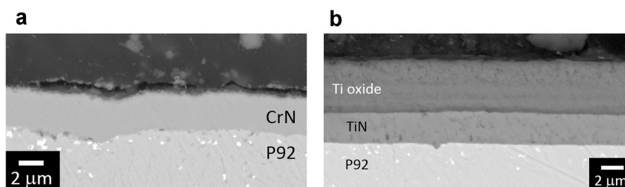
Fig. 6. SEM micrographs, in cross section view, a) of the CrN monolithic coating oxidized up to 2000 h, and b) the TiN monolithic coating oxidized up to 96 h. In both cases oxidation took place at 650 °C in 100% steam atmosphere.
