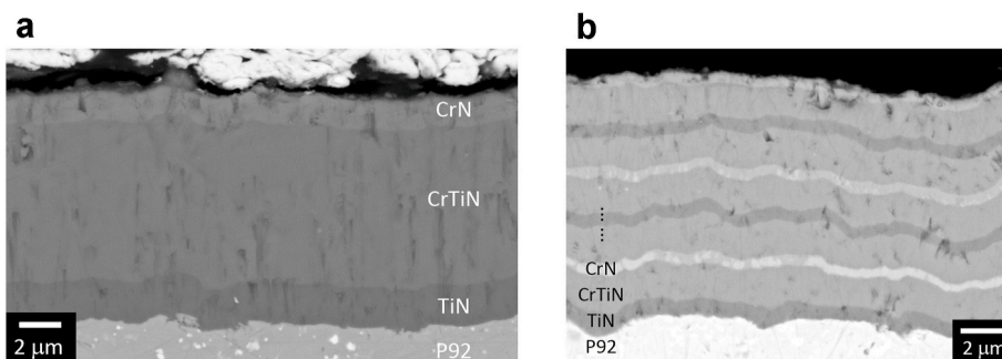
Fig. 5. SEM micrographs, in cross section view, of the oxidized layered coatings up to 2000 h at 650 °C in 100% steam atmosphere. a) CrN/CrTiN/TiN three-layer coating, and b) CrN/CrTiN/TiN multi-layered coating.
