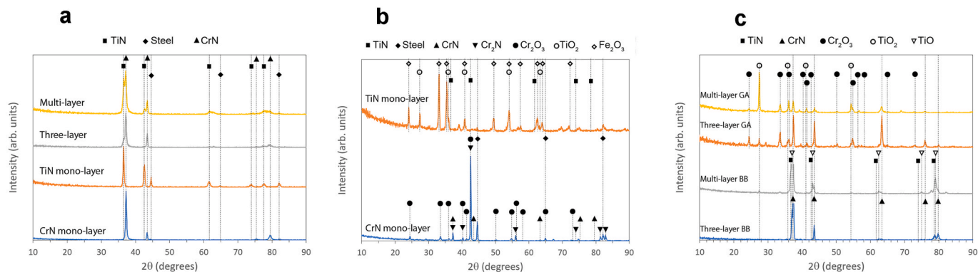
Fig. 10. XRD diffractograms of the a) as-deposited coatings with Bragg-Brentano geometry, b) oxidized monolithic coatings with Bragg-Brentano geometry, and c) oxidized layered coatings with Bragg-Brentano (BB) and grazing angle (GA) geometries.
