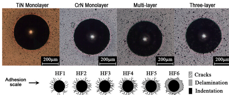
Fig. 3. Optical micrographs of the residual mark produced after Daimler-Benz Rockwell C indentation adhesion tests on the four studied coatings, and adhesion scale employed (VDI 3198).
