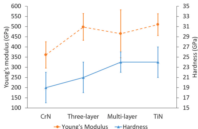
Fig. 2. Young's modulus and hardness of the studied coatings.
