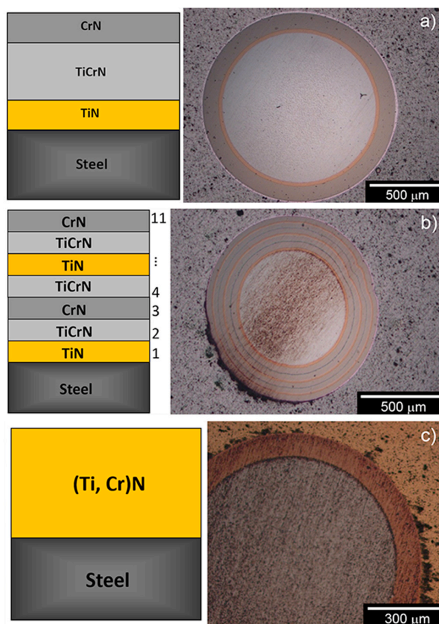
Fig. 1. Schematic layer architecture designs of the coatings and images of craters grinded by ball crater micro-abrasion method (Calotest) of a) three-layered CrN/CrTiN/TiN coating, b) multi-layered CrN/CrTiN/TiN coating and c) monolithic TiN or CrN coating: (Ti,Cr)N.
