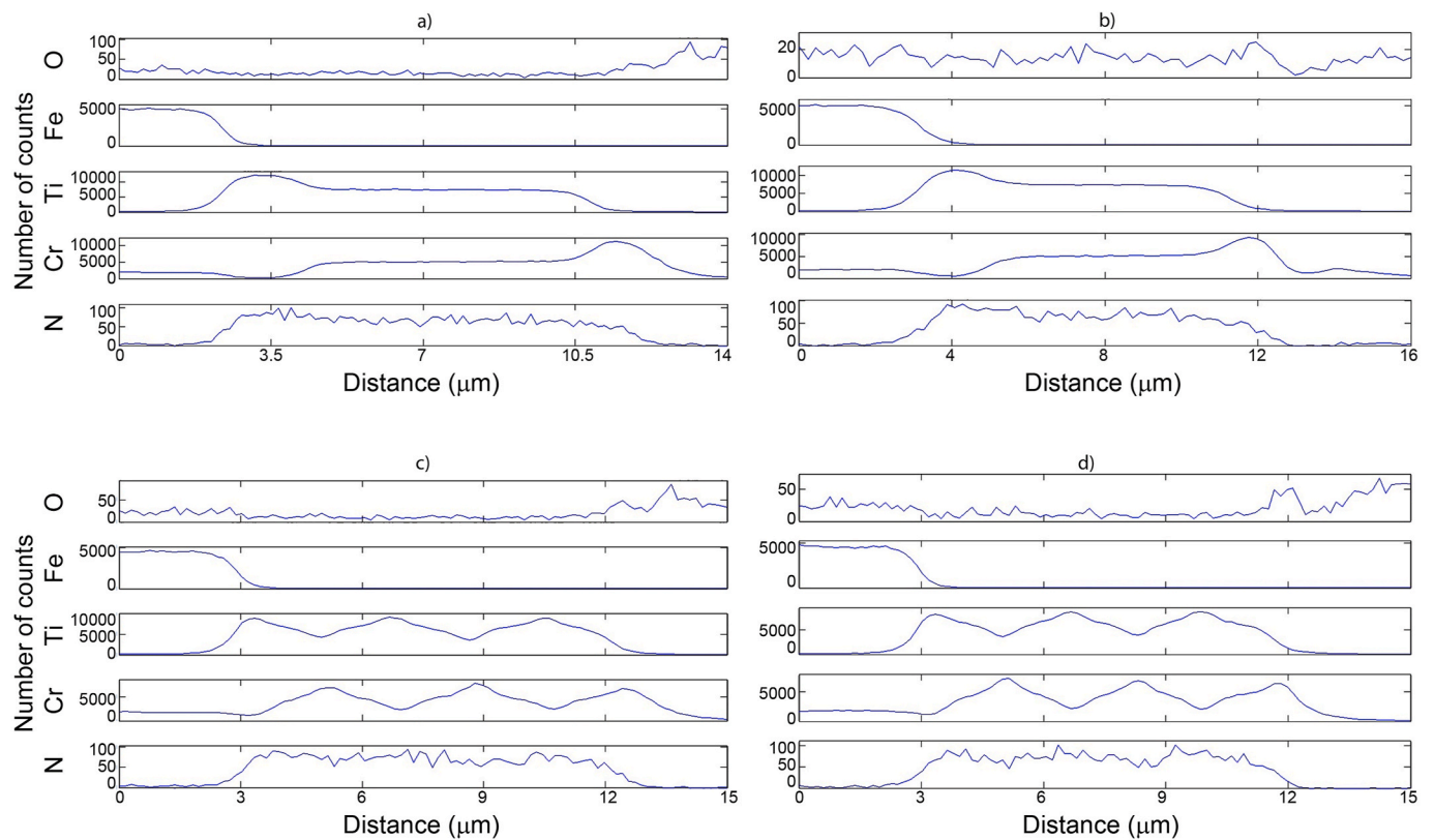
Fig. 8. Compositional depth profiles by EPMA of as-deposited and oxidized at 650 °C to 2000 h in 100% steam atmosphere: a) and b) CrN/CrTiN/TiN three-layer coating, c) and d) CrN/CrTiN/TiN multi-layer coating.
