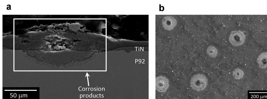
Fig. 7. SEM micrographs of the TiN monolithic coating oxidized up to 96 h at 650 °C in 100% steam atmosphere a) in a cross section view showing coating failure, and b) in a planar top view.
