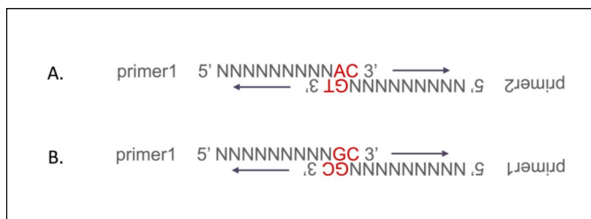
Fig. 1. Formation of primer-dimer through complementarity between the 3' ends of two primers (5A) or self-complementarity of the 3' end of a single primer (5B).
