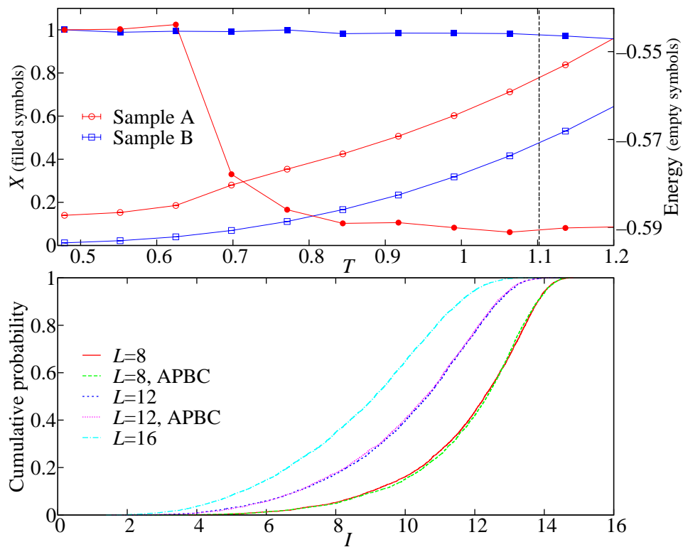
Figure 1. Signatures of temperature chaos. Top: for a strongly chaotic (A, circles) and a non-chaotic (B, squares) sample, we show the chaos parameter X_{T_{\min}=0.479, T} (solid symbols) and the energy per bond \langle H/(3L^3) \rangle_J (empty symbols) as a function of temperature. The dotted vertical line marks the critical temperature. A chaotic event for sample A at T \approx 0.65 is signalled by the strong drop of X . On the other hand, the effect in the energy is very subtle. Bottom: Probability distribution of the chaos integral I_J , as computed for lattices L = 8, 12 and 16 , with T_{\min} = 0.479 and T_{\max} = 1.6 (for all L , the same set of temperatures was used in the parallel tempering simulations). The distributions obtained with PBC and APBC are, of course, identical. The fraction of chaotic samples (i.e., small I ) increases with system size. L = 16 data from Ref. [40].
