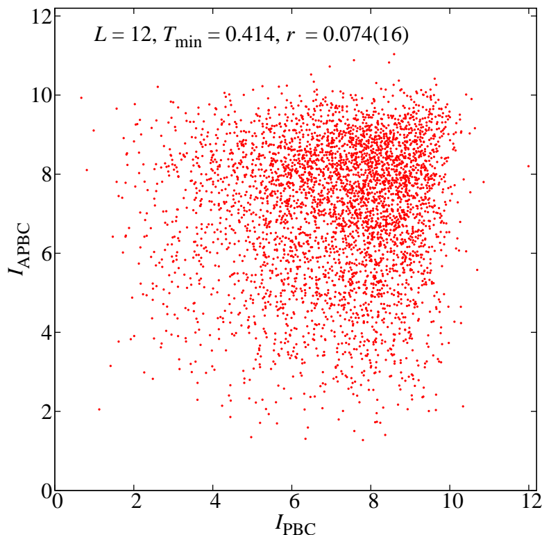
Figure 2. The non-local nature of chaos. Scatter plot of the chaos integral ( I_{\text{PBC}}, I_{\text{APBC}} ) as computed for each of our 4000 pairs of samples with L = 12 and T_{\text{min}} = 0.414 . Hereafter we shall only show data from this simulation (the qualitatively identical results for other values of L and T_{\text{min}} can be found in Appendix C).
