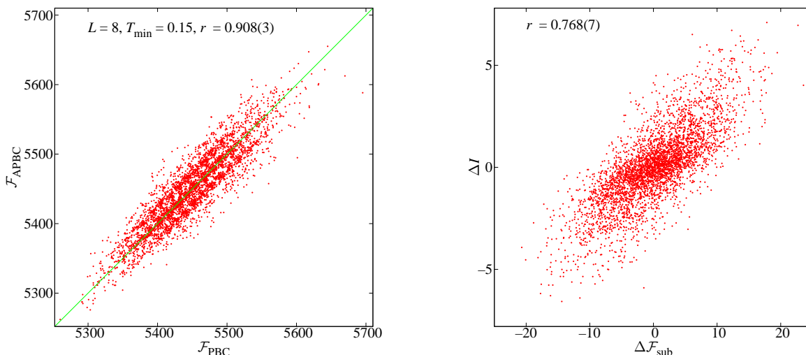
Figure C3. We show two scatter plots for our L = 8 and T_{\min} = 0.15 data (this figure is the analogous of Fig 4, as obtained for these L and T_{\min} ). Left: For the free-energy (6) we plot (\mathcal{F}_{\text{PBC}}, \mathcal{F}_{\text{APBC}}) for each of our 4000 sample pairs. The green straight line is y = x . Right: we plot (\mathcal{F}_{\text{sub,PBC}} - \mathcal{F}_{\text{sub,APBC}}, I_{\text{PBC}} - I_{\text{APBC}}) .
