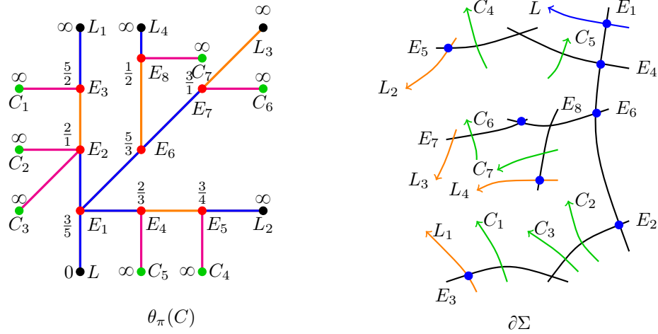
FIGURE 21. The fan tree \theta_\pi(C) is isomorphic to the dual graph of the toroidal boundary \partial\Sigma
