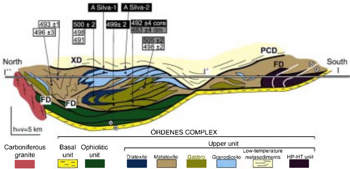
Fig. 2. Synthetic cross-section, approximately parallel to the inferred tectonic transport direction, showing the relationships between the main extensional detachments and the antiformal stack developed in the gabbroic and granodioritic plutonic complex. Abbreviations as in Fig. 1. Zircon U-Pb protolith ages are shown in black boxes, zircon U-Pb metamorphic ages in grey boxes and U-Pb monazite ages in white boxes. Hornblende ^{40}\text{Ar}/^{39}\text{Ar} ages underlined.
