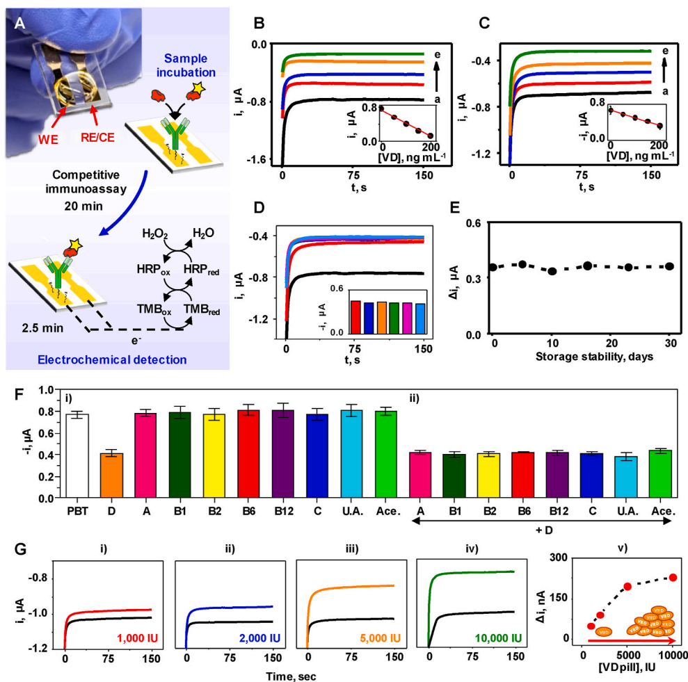
Fig. 2. VD electrochemical immunostrip characterization. A) Homemade sputtered sensor platform for single determination consisting of two Au-sputtered electrodes, employed as working (WE) and reference/counter (RE/CE) electrodes, respectively, along with the immunoreaction and transduction processes involved in the VD sensing. Chronoamperometric responses of the immunosensor to increasing VD concentrations from 0 (a) to 200 ng mL -1 (e) in 50 ng mL -1 increments in buffer B ) or saliva C ). D ) Reproducibility of the immunoassay for 100 ng mL -1 VD standards. E ) Storage stability at 4 °C of the VD Immunostrip: monitoring of the resulting variation of intensity between the electrochemical responses obtained for 0 and 100 ng mL -1 of VD over a 30-day period after its fabrication. F ) Immunosensor responses in the analysis of PBT (white bar), 100 ng mL -1 VD (orange bar), and 500 μM of each interferent in the absence (i) or presence of 100 ng mL -1 VD (ii): vitamins A (pink bars), B1 (dark green bars), B2 (yellow bars), B6 (red bars), B12 (purple bars), uric acid (U.A.) (light blue bars) and acetaminophen (Ace.) (light green bars). G ) Amperometric responses of the VD immunoplatfrom in the analysis of saliva samples collected before (black lines) and 30 min after taking i) 1000 (red line); ii) 2000 (blue line); iii) 5000 (orange line) or iv) 10,000 IU (green line) of VD pill (as 25-Hydroxyvitamin D3) and v) the corresponding variations of intensity. Dots and bars represent the mean and the error bars represent the standard deviation of the measurements performed with three different chips in B, C and F. (For interpretation of the references to colour in this figure legend, the reader is referred to the Web version of this article.)
