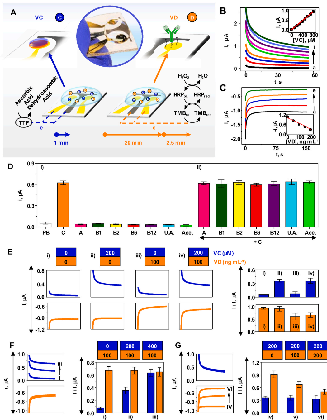
Fig. 4. VC-D Dual Chip characterization. A) Homemade sputtered dual sensor chip and schematic diagram of the localized VC and VD measurements on a single chip. Chronoamperometric responses of the dual chip to increasing B) VC concentrations from 0 (a) to 800 μM (i) in 100 μM increments or C) VD concentrations from 0 (a) to 200 ng mL -1 (e) in 50 ng mL -1 increments in buffer. D) Chronoamperometric responses of the VC sensor in the measurement of PB (white bar), 500 μM VC (blue bar), and 500 μM of each interferent in the absence (i) or presence of 500 μM VC (ii): vitamins A (pink bars), B1 (dark green bars), B2 (yellow bars), B6 (red bars), B12 (purple bars), uric acid (U.A.) (light blue bars) and acetaminophen (Ace.) (light green bars). E) Cross-talk evaluation of the dual chips in the analysis of VC-D mixture solutions. Chronoamperometric responses to various combinations of VC-D concentrations: i) absence of both markers; ii) 200 μM VC; iii) 100 ng mL -1 VD; and iv) 200 μM VC and 100 ng mL -1 VD. Evaluation of the dual chips by measuring F) increasing VC concentrations in the presence of a fixed VD level (i–iii) or G) increasing VD concentrations in the presence of a fixed VC level (iv–v). Dots and bars represent the mean and the error bars represent the standard deviation of the measurements performed with three different chips. (For interpretation of the references to colour in this figure legend, the reader is referred to the Web version of this article.)
