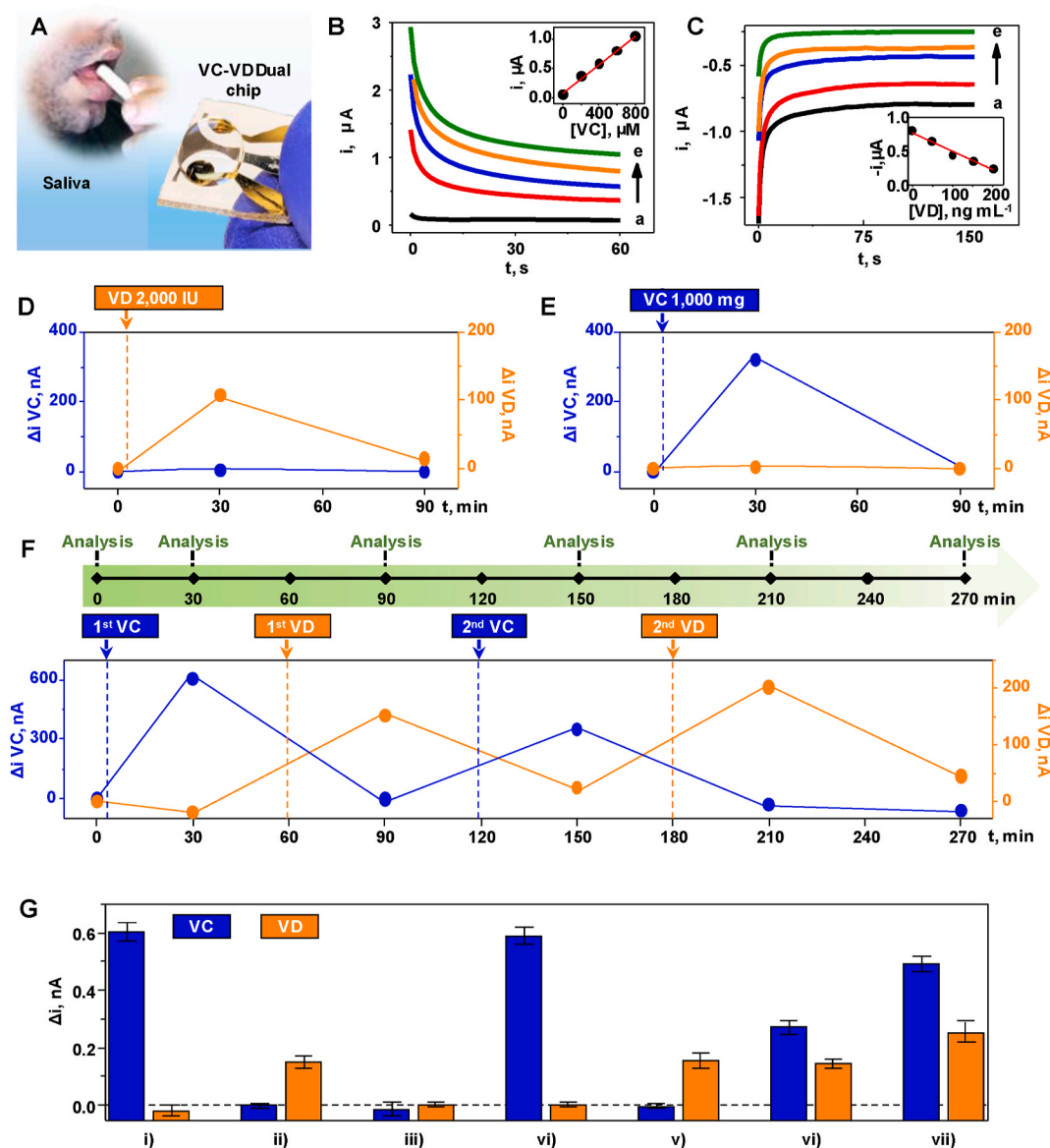
Fig. 5. Application of the VC-VD Dual Chip in saliva for personalized nutrition. A) Schematic diagram of the analysis of saliva samples with the VC-VD Dual Chip. Chronoamperometric responses of the dual chip to increasing B) VC concentrations from 0 (a) to 800 \mu\text{M} (e) in 200 \mu\text{M} increments or C) VD concentrations from 0 (a) to 200 \text{ng mL}^{-1} (e) in 50 \text{ng mL}^{-1} increments in stimulated saliva. Saliva VC & VD temporal profiles obtained using the VC-VD Dual chip developed after taking 2,000 IU VD (as 25-Hydroxyvitamin D3) (D), 1,000 mg VC (as ascorbic acid) (E) or both sequentially at 1-h time intervals (F). Dots connected by lines represent the \Delta i obtained for each analysis time. G) Variation of electrochemical responses of the VC-VD Dual chip in the analysis of saliva 30 min after intake of: i) 1,000 mg VC pill, ii) 2,000 IU VD pill, iii) vitamin B complex pill, iv) vitamin B complex and 1,000 mg VC pills, v) vitamin B complex and 2,000 IU VD pills, vi) multivitamin pill 1 (500 mg VC and 2,000 IU VD) or vii) multivitamin pill 2 (1,000 mg VC and 5,000 IU VD). Dots or bars represent the mean and the error bars represent the standard deviation of the measurements performed with three different chips in B, C and G.
