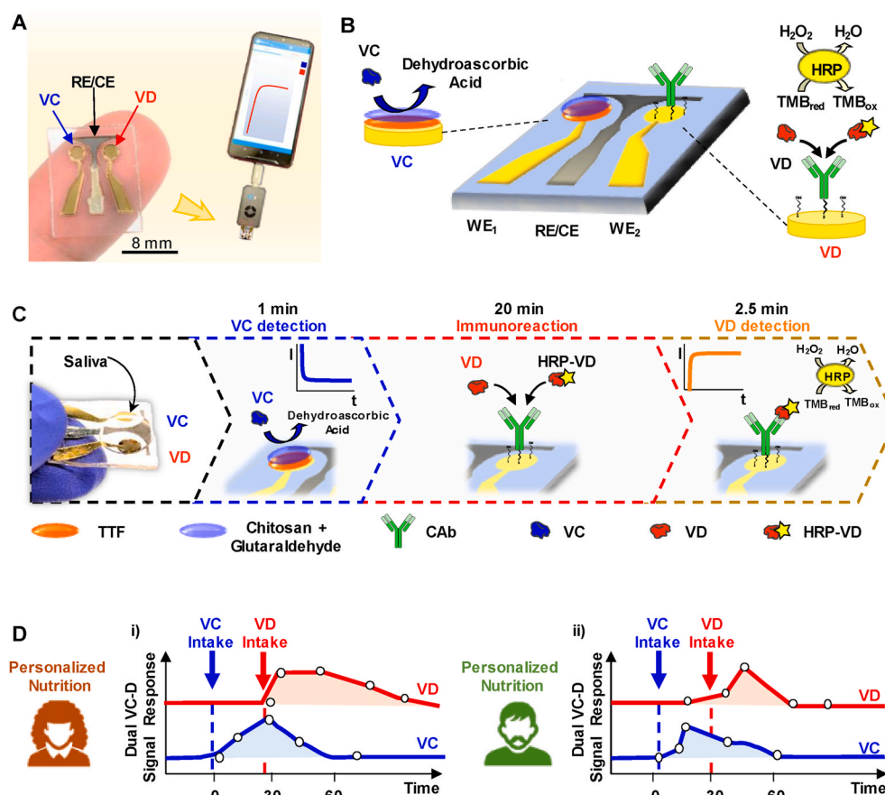
Fig. 1. The concept of VC-VD Dual Chip for personalized nutrition monitoring. A) Images of the lab made sputtered chip consisting of two Au-sputtered electrodes, employed as working electrodes (WE), and an Ag/AgCl electrode acting as a joint reference/counter (RE/CE), along with the digital monitoring. B) Schematic diagram of the localized VC and VD detection on a single sensor chip, showing the immobilized TTF and anti-VD antibody for direct competitive immunoassay allowing selective VC and VD detection, respectively. C) Analysis protocol: VC is first measured (+0.1 V, 60 s), followed by 20 min incubation of the sample supplemented with the HRP-labeled VD and electrochemical detection by chronoamperometry (-0.1 V, 2.5 min) using the H_2O_2 /HRP/TMB redox probe. D) The conceptual idea of interindividual variability in responding to VC and VD micronutrients administration: distinct VC and VD temporal variation profiles for two different subjects (i, ii).
