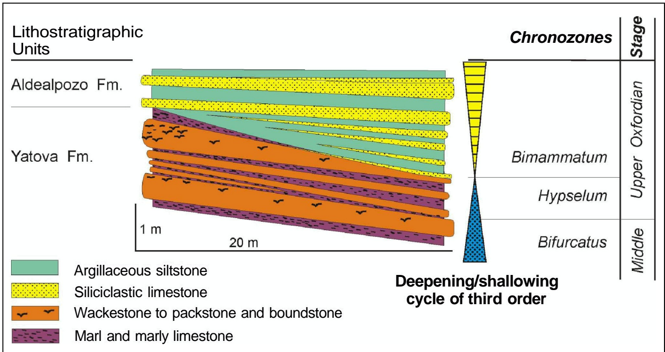
Fig. 2 - Sketch of the stratigraphic succession along a lateral extension of 20 m, as observed in one of the studied outcrops and shown in Fig. 3. This stratigraphic succession comprises a 3 m thick interval, from which the first 2 m correspond to the upper part of Yátova Formation and the uppermost metre belongs to the lower part of Aldealpozo Formation. This succession corresponds to the Bifurcatus (upper part of Middle Oxfordian), Hypselum and Bimammatum (Upper Oxfordian) chronozones. The boundary between these successive formations represents a gradual or a sudden facies change, associated with syndepositional palaeoreliefs developed during the Late Oxfordian. The highest stratigraphic interval of the Yátova Formation developed during the Hypselum Chronozone is composed of marly condensed deposits and represents a condensed section, according to the results of the present work. Upper Oxfordian deposits in this area belong to a single third order deepening/ shallowing environmental cycle. Deposits of the Yátova Formation represent the last phase, of advanced deepening conditions, within a deepening half-cycle. In contrast, deposits of the Aldealpozo Formation represent the first phase, of incipient shallowing conditions, within a shallowing half-cycle.
