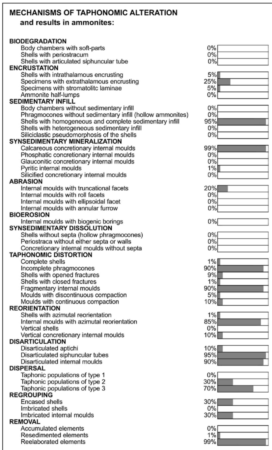
Fig. 6 - Mechanisms of taphonomic alteration and results leading to the development of the ammonites included in condensed deposits from the Hypselum Chronozone in Ricla area.
