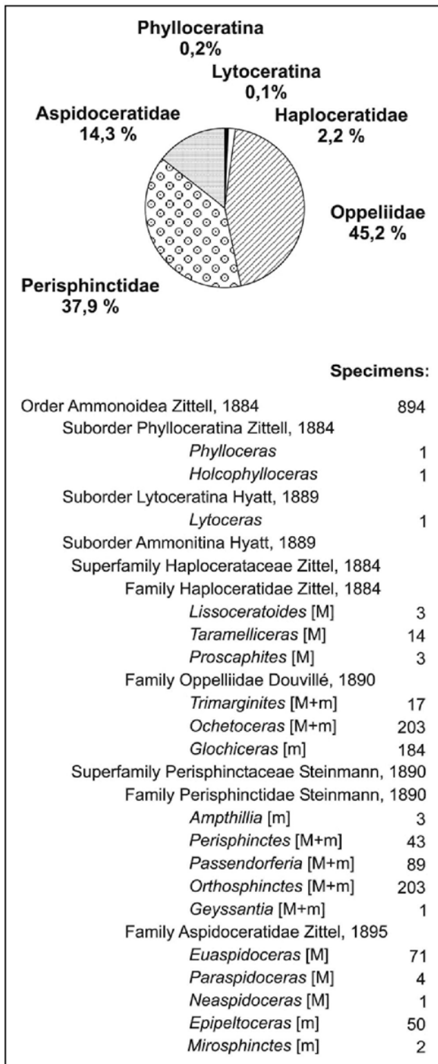
Fig. 5 - Relative abundance of different ammonoid groups from the Hypselum condensed section in Ricla area.
