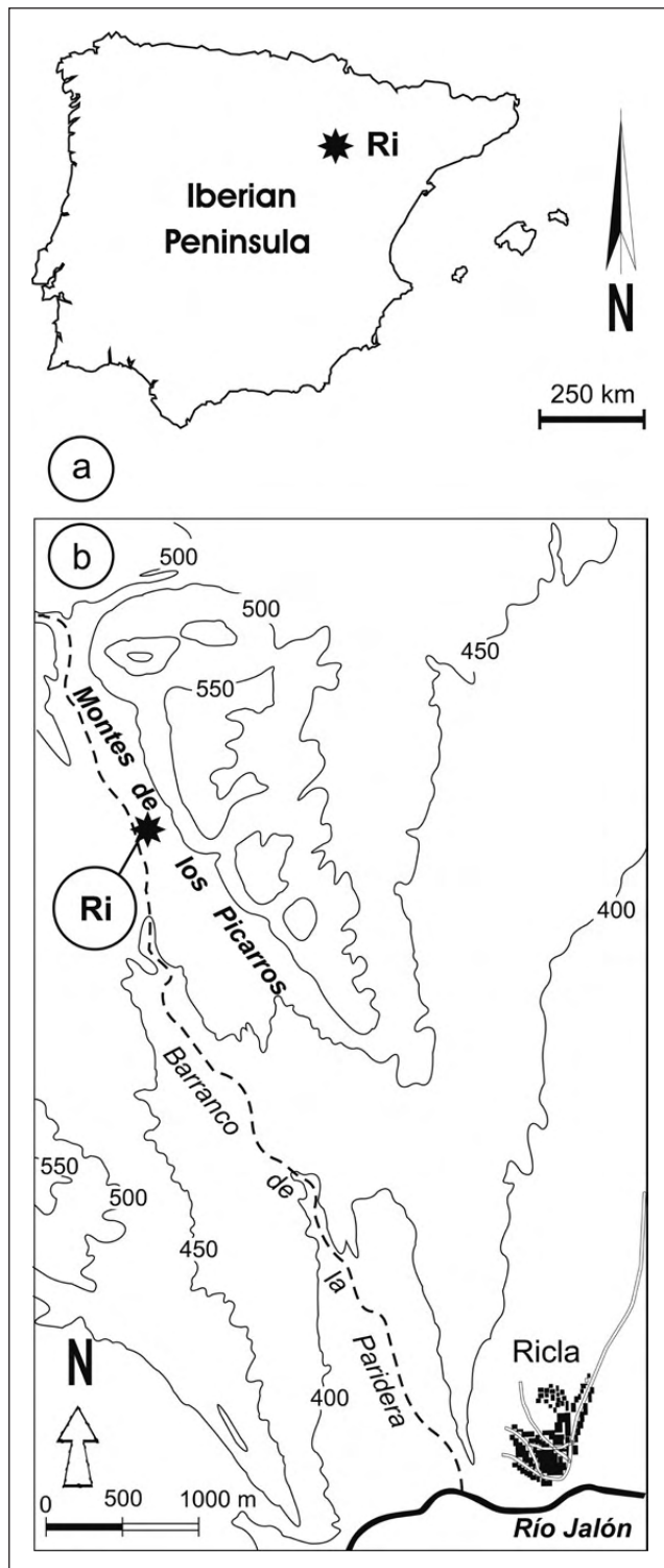
Fig. 1 - Geographical location of the study area, north of the locality of Ricla (Zaragoza province, north-eastern Iberian Peninsula), showing the point of the sampled outcrops (Ri).
