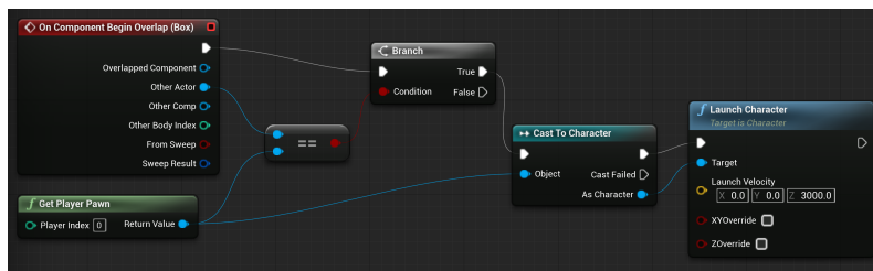
Figura 2.8: Blueprints en Unreal Engine
