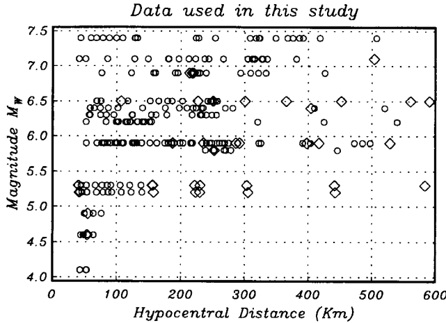
Figure 2. Magnitude versus distance plot summarizing the data used in this study. Symbols indicate the type of data available: open circles, accelerograms; diamonds, broadband velocity data. Stations located in the Valley of Mexico, known to suffer large amplification of seismic waves, are not plotted. Note that the data set includes four events that have the same magnitude of M_w = 5.9 (Table 1).
