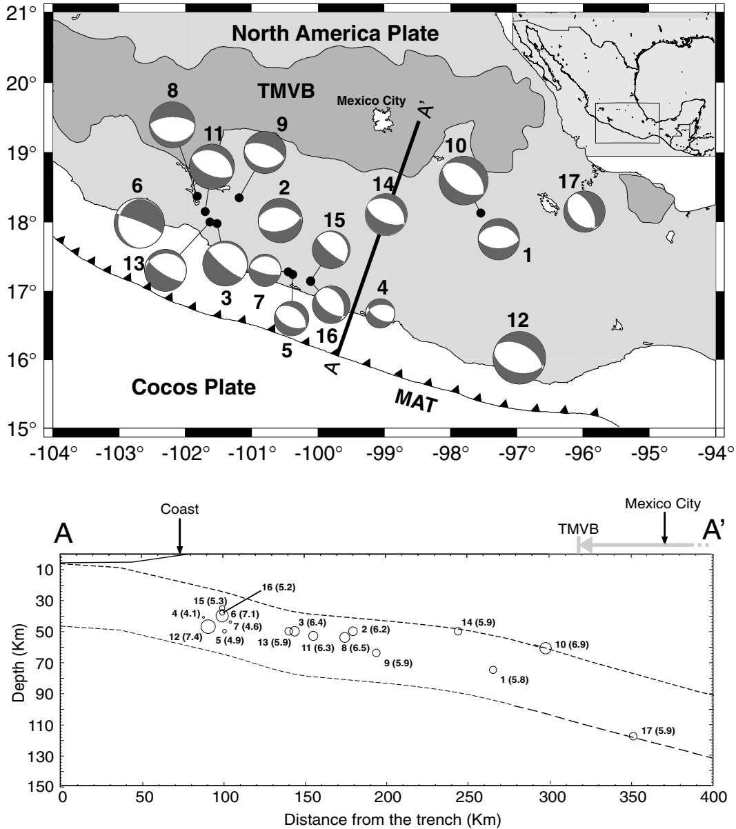
Figure 1. (Top) Map of Mexico showing epicenters and focal mechanisms of normal-faulting, intermediate-depth inslab earthquakes analyzed in this study. Each event is identified by a number, which is keyed to Table 1. TMVB, Trans-Mexican Volcanic Belt; MAT, Middle America Trench. (Bottom) The projection of the hypocenters of the inslab events on a vertical plane AA'. Moment magnitude, M_w , of each event is given in brackets. The dashed lines delineate the subducted Cocos plate.
