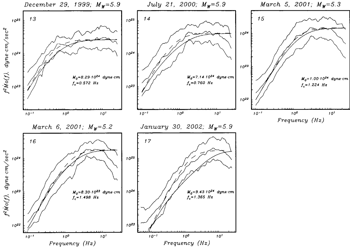
Figure 8. Source acceleration spectra of the in-slab Mexican earthquakes (mean and \pm 1 standard deviation curves). Superimposed on the spectra are predicted curves from an \omega^2 source model (dashed smooth curves) and a two-corner empirical source model (continuous smooth curves). Theoretical curves correspond to the seismic moments of the events, and their stress drops are constrained by the high-frequency spectral level.
