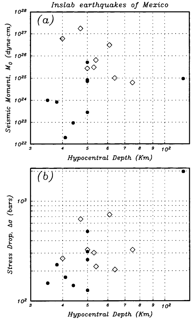
Figure 10. (a) M_0 versus depth. (b) \Delta\sigma versus depth. Filled circles, data from spectra well fitted by an \omega^2 source model; diamonds, data from spectra better matched by the empirical two-corner frequency source model. In the large dispersion of the data, one may discern a slight tendency of both M_0 and \Delta\sigma to increase with depth.
