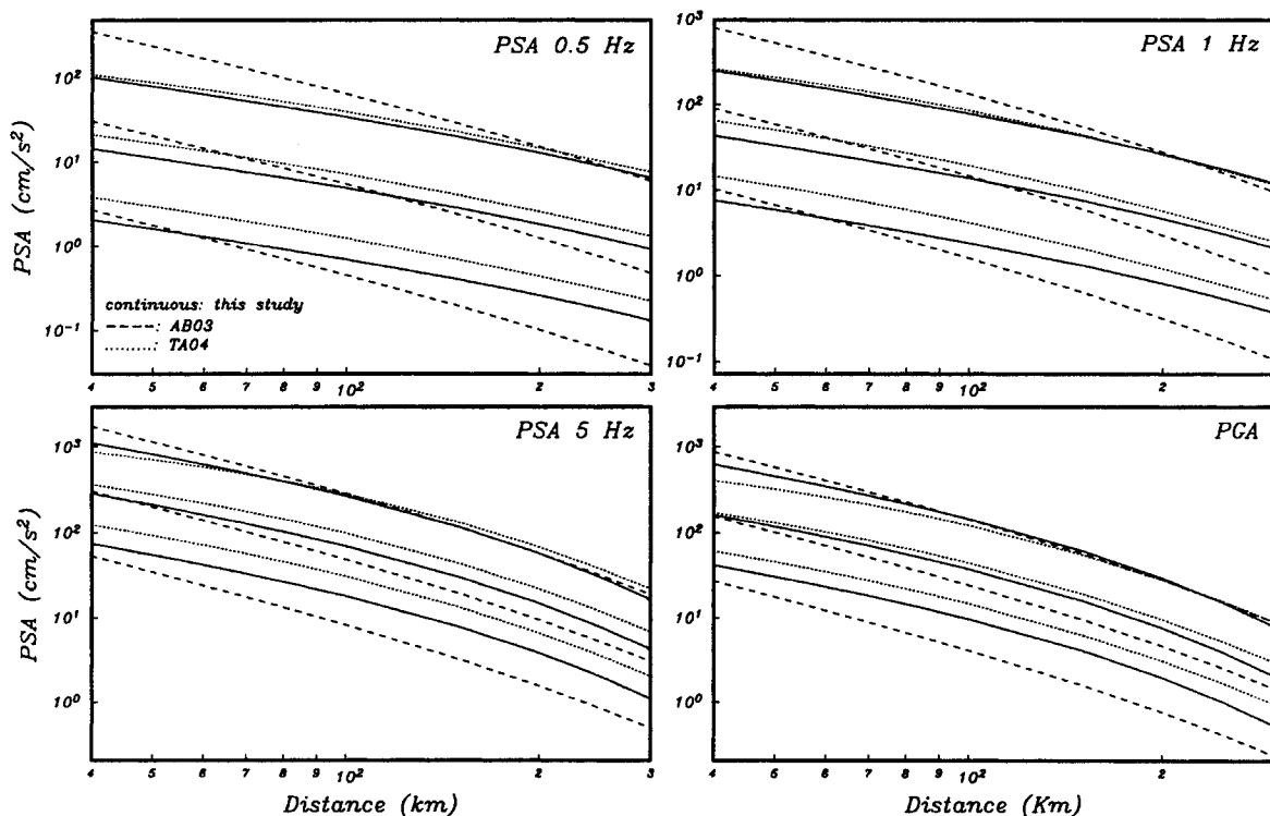
Figure 8. Regression curves of horizontal component of PSA at 0.5, 1, and 5 Hz, and PGA for earthquakes of M_w 5.5, 6.5, and 7.5, with H = 50 km, for different strong-motion models. Continuous curves, this study (quadratic mean horizontal component); dashed curves, Atkinson and Boore (2003), worldwide inslab model (random horizontal component); dotted curves, Takahashi et al. (2004), Japanese inslab model (geometric mean horizontal component).
