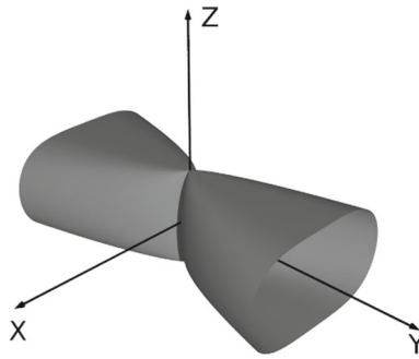
Fig. 1 A swung surface: -y^2 + x^4 + z^2y^2 = 0
