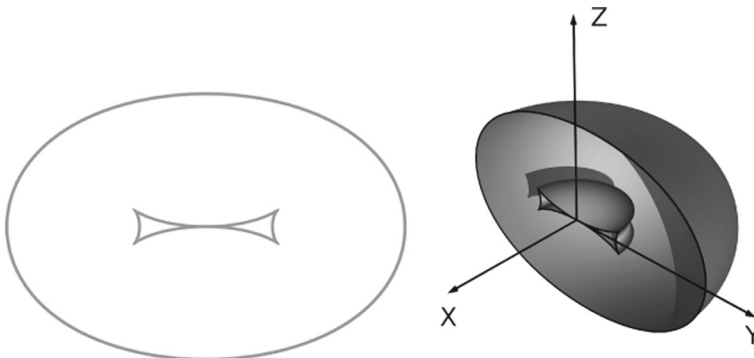
Fig. 3 A rational revolution surface, not generated by a rational curve. Left offset of the ellipse (profile curve of genus 1); Right half offset of the ellipsoid (rational revolution surface)
