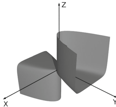
Fig. 2 Another swung surface: x^6z^2 - 8y^3z + 6x^4zy + x^6
