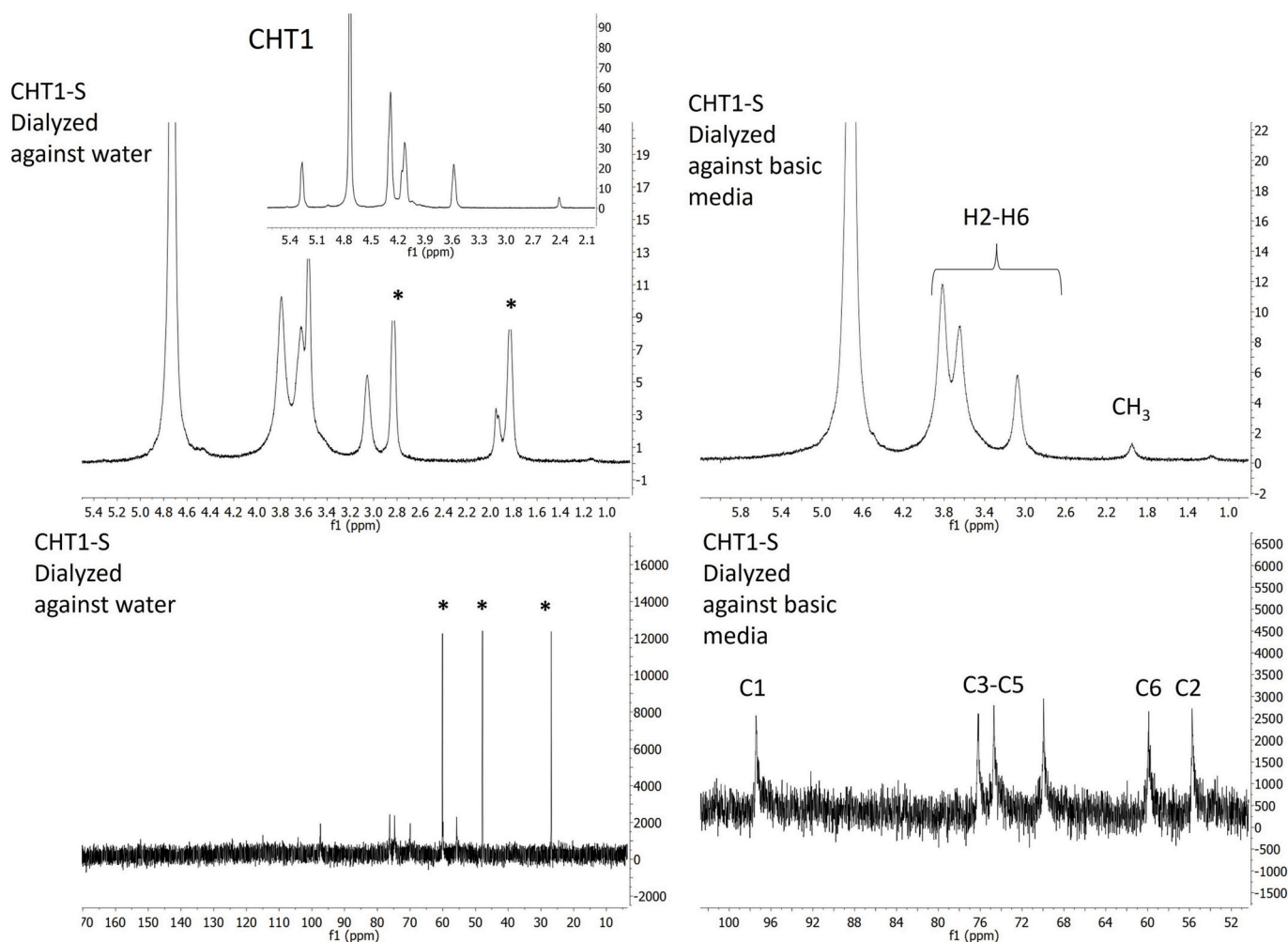
Fig. 1. Liquid 1 H NMR in D 2 O/DCl of samples CHT1-S dialyzed against water (A) and basic media (B). Liquid 13 C NMR in D 2 O/DCl of samples CHT1-S dialyzed against water (C) and basic media (D). Inset in panel A) Liquid 1 H NMR in D 2 O/DCl of sample CHT1.
