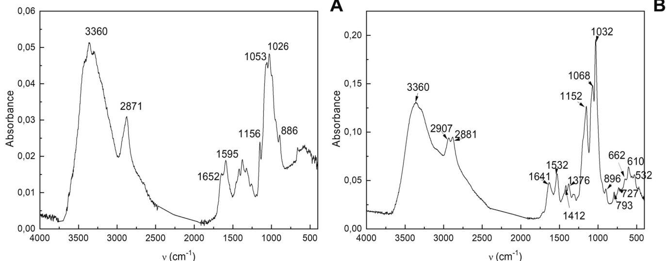
Fig. 2. ATR-FTIR Spectra of chitosan (A) and chitosan salt (B).
