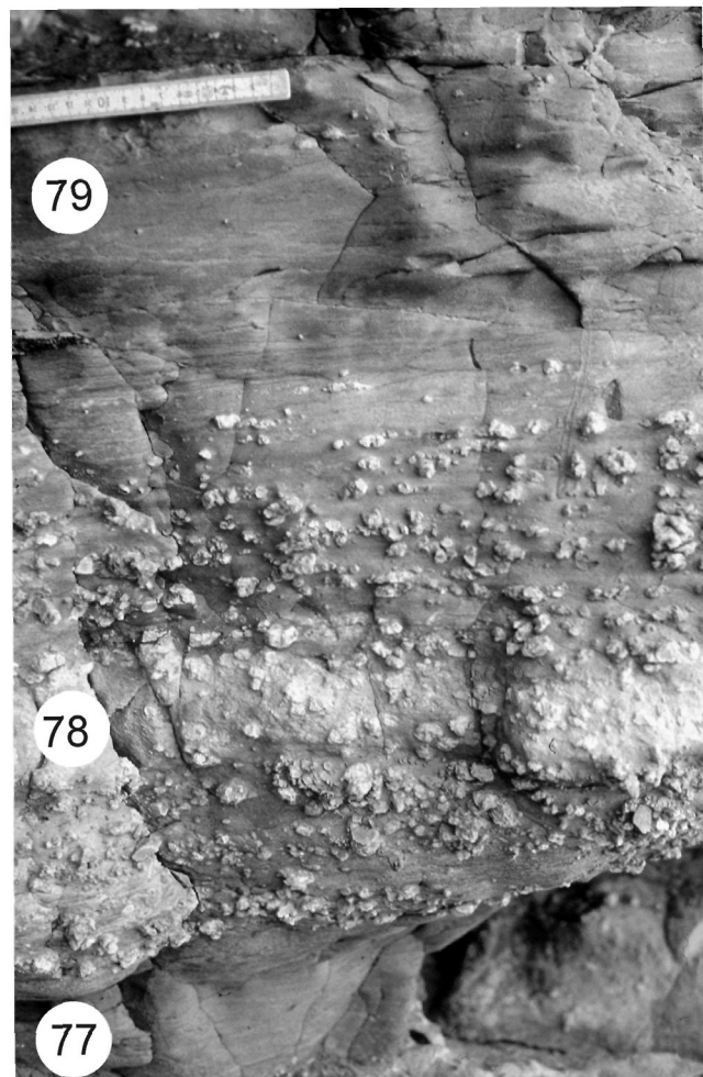
Figure 5.- Close-up view of the level 78 (taphofacies 1, lumpy limestones and marly intervals with reelaborated ammonites), showing gradational boundaries. Bar for scale is 17 cm long.
