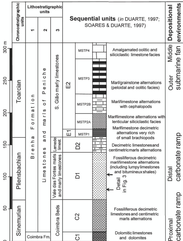
Figure 2.- Diagrammatic section of the Lower Jurassic in the Peniche Peninsula: lithostratigraphic units (1 and 3 for all the Lusitanian Basin (in Duarte 1997); 2 - sector of Peniche in Carta Geológica de Portugal, 1992), facies and depositional environments.
