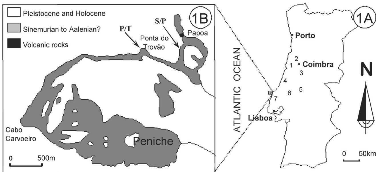
Figure 1- A) Location map of the main sections of Vale das Fontes marls and marly limestones (Quiaios Fm.) in the Lusitanian Basin (1 - Brenha, 2 - Coimbra, 3 - Rabaçal, 4 - S. Pedro de Moel, 5 - Tomar, 6 - Porto de Mós, 7 - Peniche). B) Geological map of the Lower Jurassic in the Peniche Peninsula (S/P - Sinemurian/Pliensbachian boundary; P/T - Pliensbachian/Toarcian boundary).
