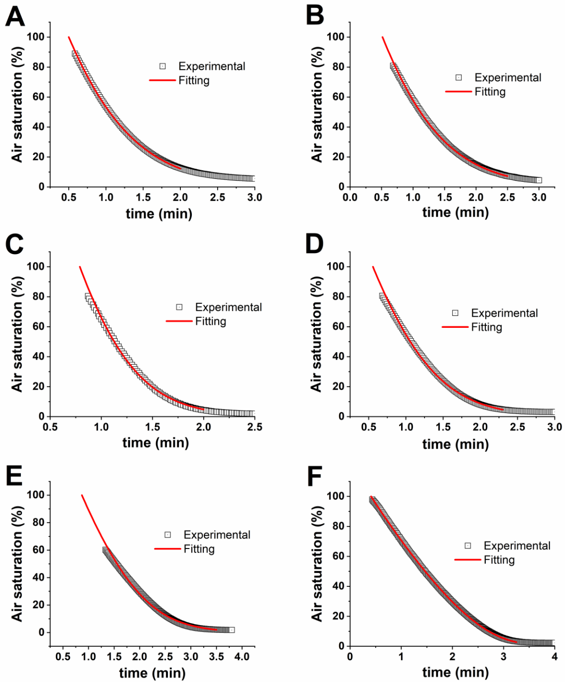
Figure S10. Single response integral analysis with BM for GOX. Panel A: 40 mM of glucose, Panel B: 30 mM of glucose, Panel C: 20 mM of glucose, Panel D: 10 mM of glucose, Panel E: 5 mM of glucose, Panel F: 1 mM of glucose. Experimental data (square dots), simulated data (red line).
