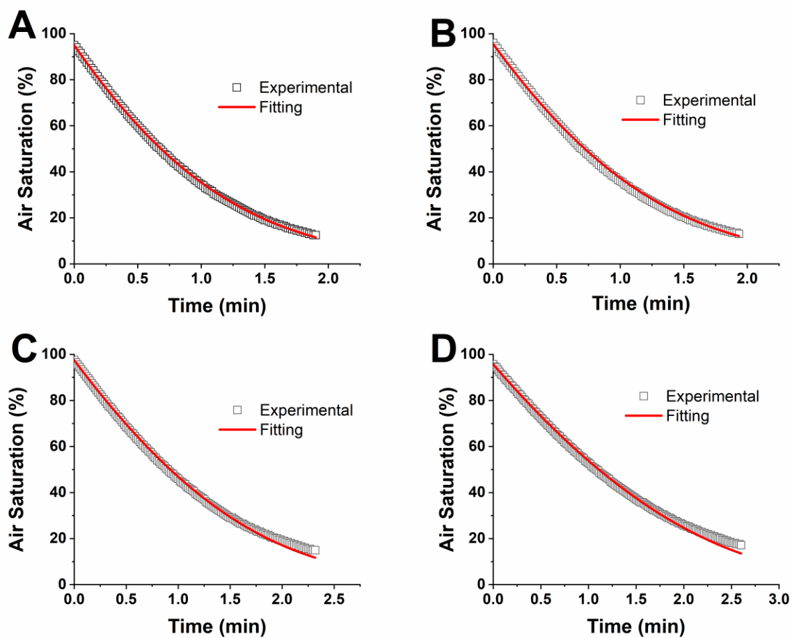
Figure S17. Multiple response integral analysis with Aspen for laccase. Panel A: 5.0 mM of catechol, Panel B: 3.0 mM of catechol, Panel C: 1.0 mM of catechol, Panel D: 0.6 mM of catechol. Experimental data (square dots), simulated data (red line).
