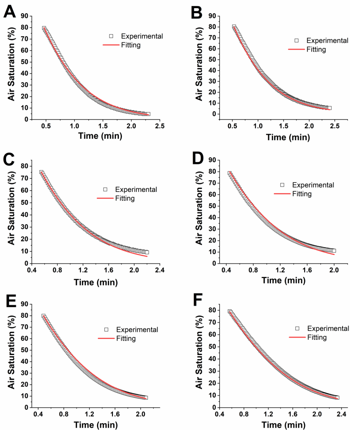
Figure S15. Multiple response integral analysis with Aspen for GOX. Panel A: 2000 mM of glucose, Panel B: 400 mM of glucose, Panel C: 100 mM of glucose, Panel D: 75 mM of glucose, Panel E: 50 mM of glucose, Panel F: 25 mM of glucose. Experimental data (square dots), simulated data (red line).
