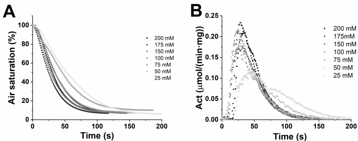
Figure S5. Representative set of oxygen time courses upon variation of main substrate concentration for GalOx with K_3Fe(CN)_6 as activator. Panel A: Air saturation time course, Panel B: Specific reaction rate (enzyme activity) time course. Data in Panel B are obtained by finite incremental differentiation of Panel A data. Concentration of enzyme, E, was adjusted to have a suitable number of data points (E was increased at low activities and E was decreased at high activities; [E]=0.5-0.75 mg/mL). [O_2] = 0.25 mM at 100 % air saturation conditions and 25 °C.
