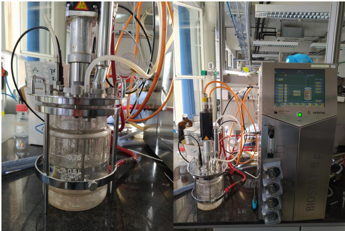
Figure S2. Stirred tank reactor of 1 L (Biostat B Plus) from Sartorius AG where the experiments at medium-scale were performed. The reactor was equipped with a sintered metal sparger and a Rushton turbine for mixing. Oxygen and pH were measured with probes from Hamilton Company.
