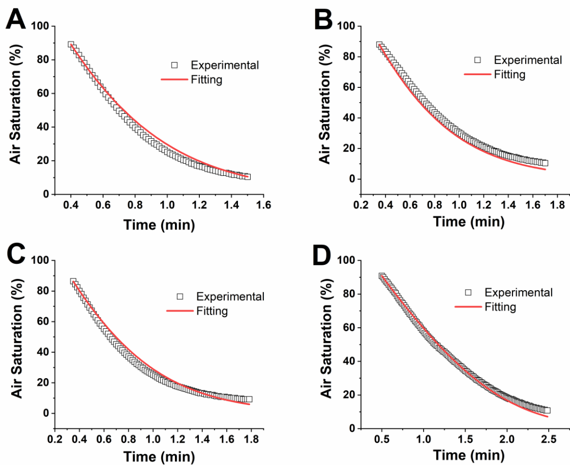
Figure S16. Multiple response integral analysis with Aspen for GalOx with K_3Fe(CN)_6 . Panel A: 175 mM of galactose, Panel B: 150 mM of galactose, Panel C: 100 mM of galactose, Panel D: 25 mM of galactose. Experimental data (square dots), simulated data (red line).
