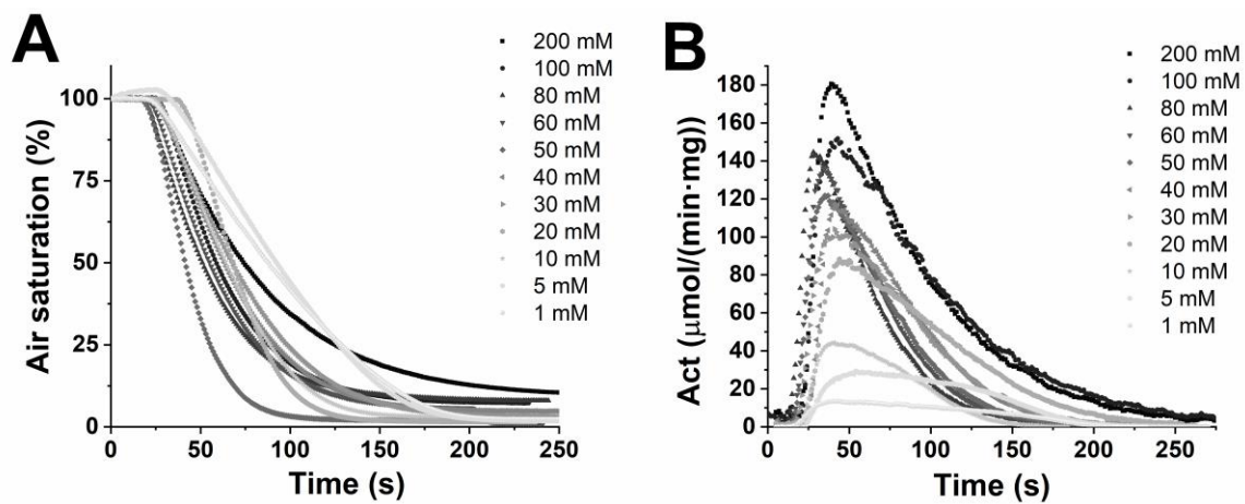
Figure S3. Representative set of oxygen time courses upon variation of main substrate concentration for GOX. Panel A: Air saturation time course, Panel B: Specific reaction rate (enzyme activity) time course. Data in Panel B are obtained by finite incremental differentiation of Panel A data. Concentration of enzyme, E, was adjusted to have a suitable number of data points (E was increased at low activities and E was decreased at high activities; [E]=0.0015\text{-}0.003 mg/mL). [\text{O}_2] = 0.25 mM at 100 % air saturation conditions and 25 °C.
