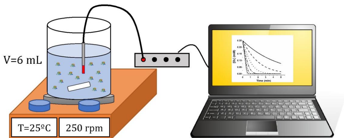
Figure S1. Oxygen consumption time course performed with a fiber-optic oxygen sensor FireSting®-PRO (FSPRO-4) from PyroScience. The experiments were performed in a 6 mL flask controlling the temperature at 25^{\circ}\text{C} and with magnetically stirring at 250 rpm.
