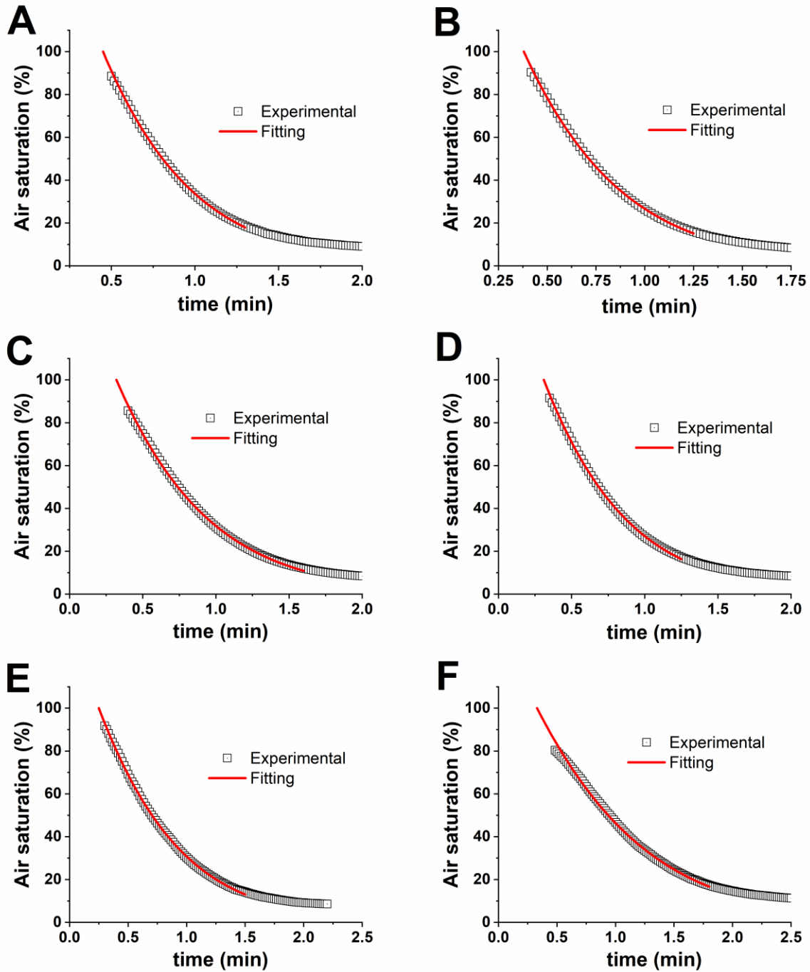
Figure S12. Single response integral analysis with BM for GalOx with K_3Fe(CN)_6 as activator. Panel A: 200 mM of galactose, Panel B: 175 mM of galactose, Panel C: 150 mM of galactose, Panel D: 100 mM of galactose, Panel E: 75 mM of galactose, Panel F: 50 mM of galactose. Experimental data (square dots), simulated data (red line).
