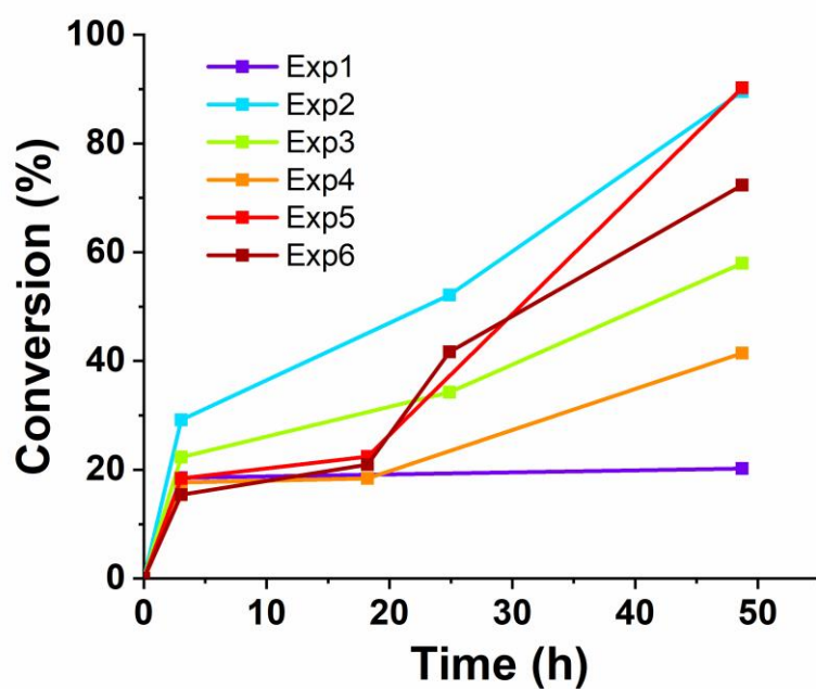
Figure S20. Conversion of galactose vs time experiments for GalOx with surface aeration. Exp1: 4.6 mg/mL enzyme, 0.09 mg/mL HRP, no catalase. Exp2: 4.6 mg/mL enzyme, 0.18 mg/mL HRP, 0.09 mg/mL catalase. Exp3: 4.2 mg/mL enzyme, 0.17 mg/mL HRP, 0.84 mg/mL catalase. Exp4: 4.5 mg/mL enzyme, 0.18 mg/mL K_3Fe(CN)_6 , no catalase. Exp5: 4.5 mg/mL enzyme, 0.18 mg/mL K_3Fe(CN)_6 , 0.09 mg/mL catalase. Exp6: 2.5 mg/mL enzyme, 0.17 mg/mL K_3Fe(CN)_6 , 0.17 mg/mL catalase. [Galactose]_0 = 20 mM.
