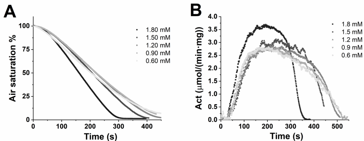
Figure S7. Representative set of oxygen time courses upon variation of main substrate concentration for Tyrosinase. Panel A: Air saturation time course, Panel B: Specific reaction rate (enzyme activity) time course. Data in Panel B are obtained by finite incremental differentiation of Panel A data. Concentration of enzyme, E, was adjusted to have a suitable number of data points (E was increased at low activities and E was decreased at high activities; [E]=0.10\text{-}0.16\text{ mg/mL} ). [\text{O}_2] = 0.25\text{ mM} at 100 % air saturation conditions and 25 °C.
