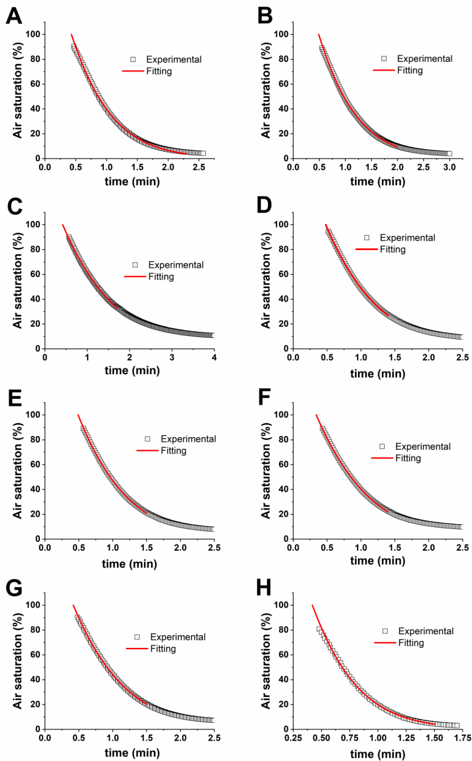
Figure S9. Single response integral analysis with BM for GOX. Panel A: 2000 mM of glucose, Panel B: 400 mM of glucose, Panel C: 200 mM of glucose, Panel D: 100 mM of glucose, Panel E: 90 mM of glucose, Panel F: 80 mM of glucose, Panel G: 60 mM of glucose, Panel H: 50 mM of glucose. Experimental data (square dots), simulated data (red line).
