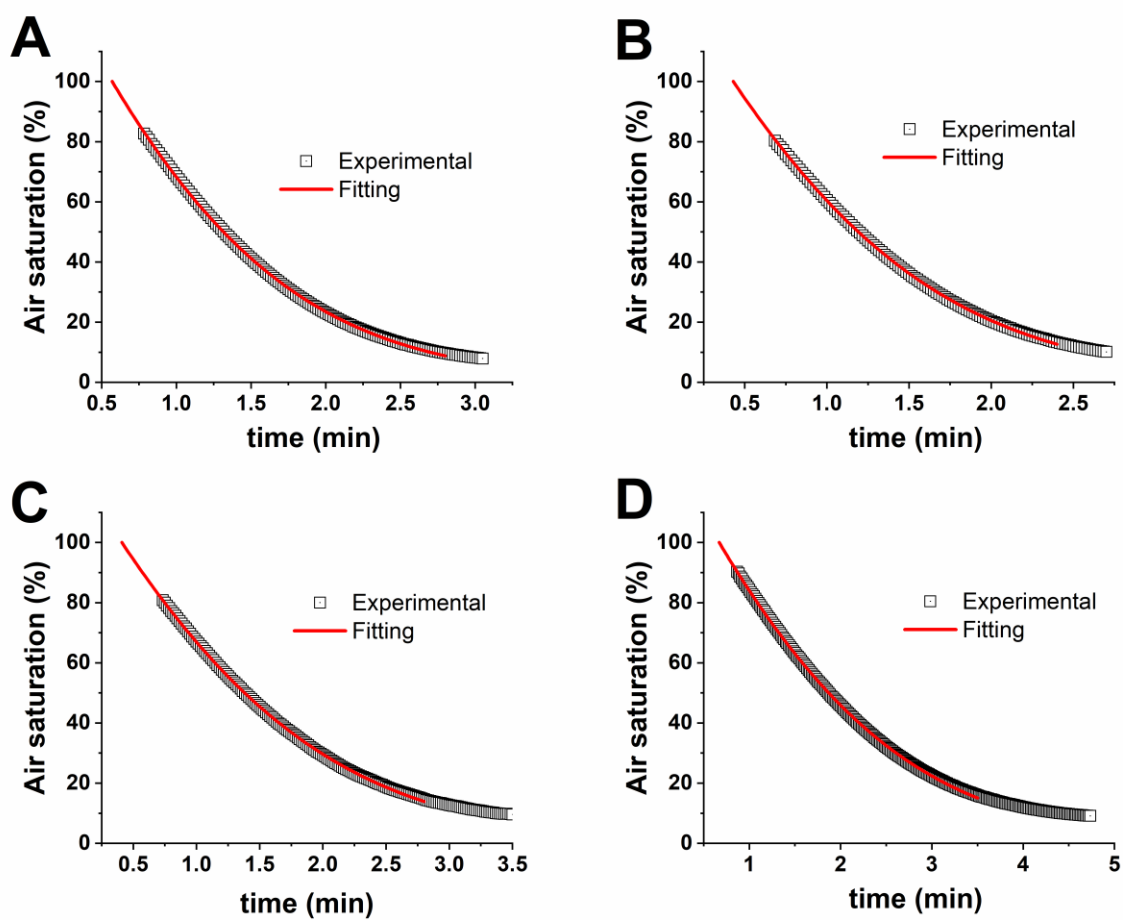
Figure S13. Single response integral analysis with BM for laccase. Panel A: 5 mM of catechol, Panel B: 3 mM of catechol, Panel C: 1 mM of catechol, Panel D: 0.6 mM of catechol. Experimental data (square dots), simulated data (red line).
