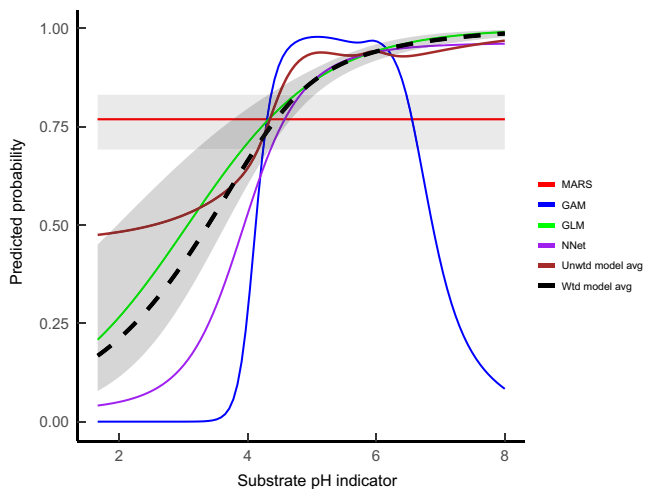
FIGURE 4 Modeled response of Coeloglossum viride to an indirect indicator of substrate pH. The modeled response was assessed by both experts as moderate (expert 1) and poor (expert 2). Their assessment would have been based solely on inspection of the unweighted model average (brown line). Raw probabilities have been rescaled to between 0 and 1. Gray ribbons indicate the 95% confidence region for the relevant modeled response
