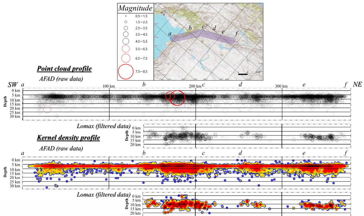
Figure 9. Seismicity profiles along the Main Strand of the EAFZ oriented approximately N60°E. Upper image: The location of the profile and the buffer used to select the seismic foci. Center of the figure: Point cloud of earthquakes at different depths, differentiated by magnitude. Upper: Raw data (AFAD); Lower: filtered data (Lomax, 2023 [35]). At the bottom of the figure: Kernel density profiles. Upper: Raw data; Lower: filtered data. Different points are marked with letters both on the profiles and on the map to accurately locate the black loci.
