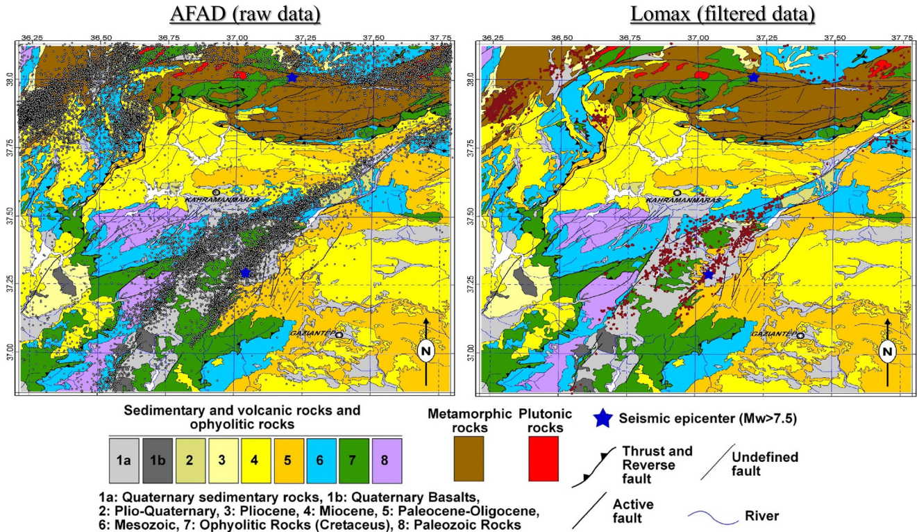
Figure 10. Detailed geological map of the surroundings of the major earthquakes, with epicenters from both datasets: AFAD (raw dataset, black dots) on the left and Lomax (2023) [35] (relocated-filtered, red dots) on the right.
