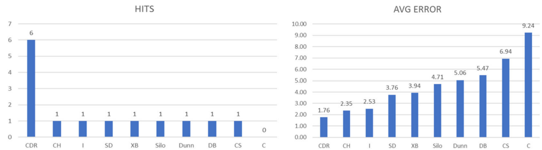
FIGURE 9 Average error rate (right); success rate (left) of the internal indices [Color figure can be viewed at wileyonlinelibrary.com ]
