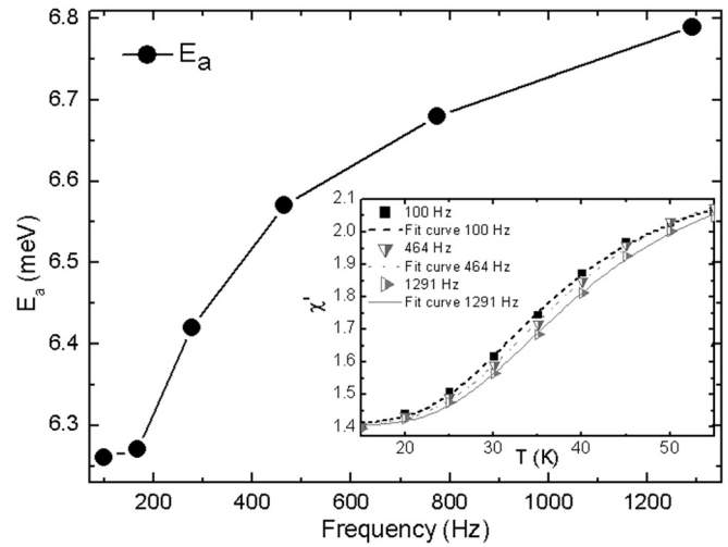
FIG. 3. Activation energy, E_a , dependence on frequency. The inset shows the in-phase susceptibility curves with their corresponding fittings.
