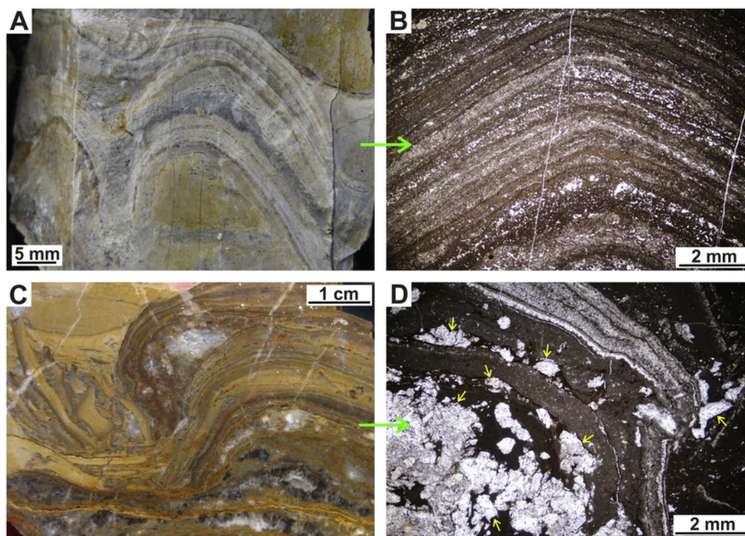
Fig. 13. Micritic-evaporitic stromatolites of the Leza Fm. A, C: Polished hand specimens. B, D: Photomicrographs of the same specimens. Note abundant pseudomorphs after evaporites disrupting lamination both at meso- and micro-scale in C (crystalline white and gray areas) and D (yellow arrows), respectively. (For interpretation of the references to colour in this figure legend, the reader is referred to the web version of this article.)
