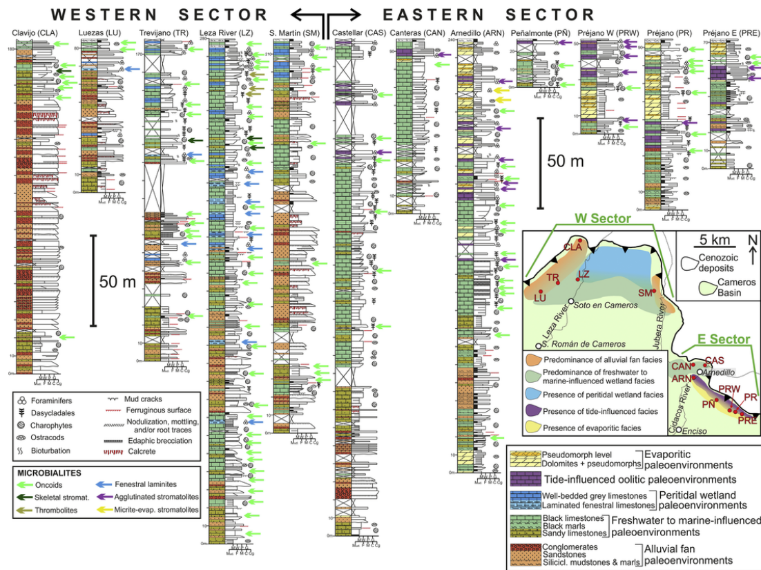
Fig. 4. Stratigraphic sections logged in the Leza Fm with their geographical location (red dots) shown in the map at the right side (see location in Fig. 3B). Modified after Suarez-Gonzalez et al. (2015). Colors in the sections and in the inset map (equivalent to the colour-code of Figs. 2, 5 and 15) are related to the different paleoenvironments interpreted for the unit, as described in the text. Colored arrows mark the stratigraphic location of the studied microbialites. Note that some paleoenvironments and some microbialites have a widespread distribution throughout the unit, whereas others only occur in particular geographical sectors (as highlighted in the inset map). (For interpretation of the references to colour in this figure legend, the reader is referred to the web version of this article.)
