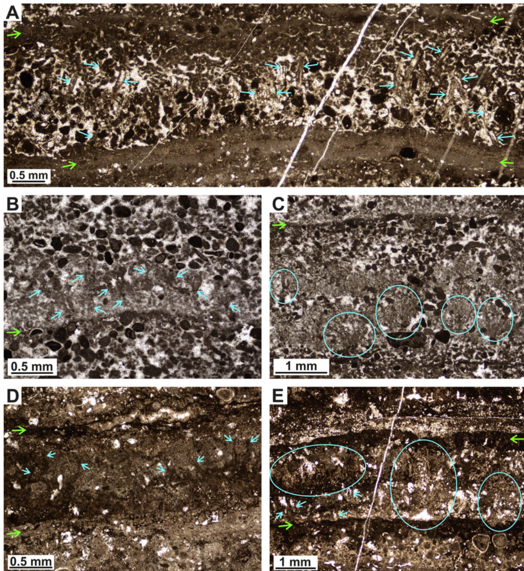
Fig. 11. A-E Photomicrographs of the rare filament remains observed in the agglutinated stromatolites of the Leza Fm. Note that filament remains (blue arrows and ellipses) are poorly preserved, mostly as individual elongated clusters of clotted-peloidal micrite, being only locally associated in tufts (ellipses of C and E). Compare the preservation of filaments with that of modern agglutinated microbialites (Fig. 1F–G). Green arrows point to thin micritic crusts between successive laminae, strongly similar to those of modern analogues (Fig. 1H–I). (For interpretation of the references to colour in this figure legend, the reader is referred to the web version of this article.)
