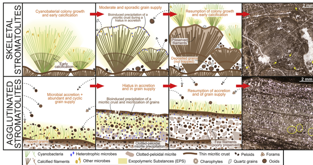
Fig. 9. Contrasting accretion processes that generate skeletal and agglutinated stromatolites. Skeletal stromatolites accrete through the growth of colonies of filamentous microbes (probably cyanobacteria) and the early and pervasive precipitation of carbonate in the EPS sheaths of their filaments. Thus, filaments are well-preserved, whereas grains supplied on the stromatolite surface are not trapped and bound in the microbial EPS, but only deposited between the filament fans (yellow arrows in photomicrograph). In contrast, agglutinated stromatolites accrete through the development of benthic microbial communities simultaneous with abundant and cyclic grain supply. Filamentous microbes are not early calcified (and thus only locally and poorly preserved, yellow areas in photomicrograph, see Fig. 11), whereas grains are profusely trapped and bound in the uncalcified EPS. Lithification of the biofilms may occur subsequently, through precipitation of clotted-peloidal micrite probably influenced by the degradation of EPS by heterotrophic microbes. Thin micritic crusts separating successive laminae (see Figs. 10E, 11) form during interruptions in accretion and in grain supply (cf. Fig. 1H–I). (For interpretation of the references to colour in this figure legend, the reader is referred to the web version of this article.)
