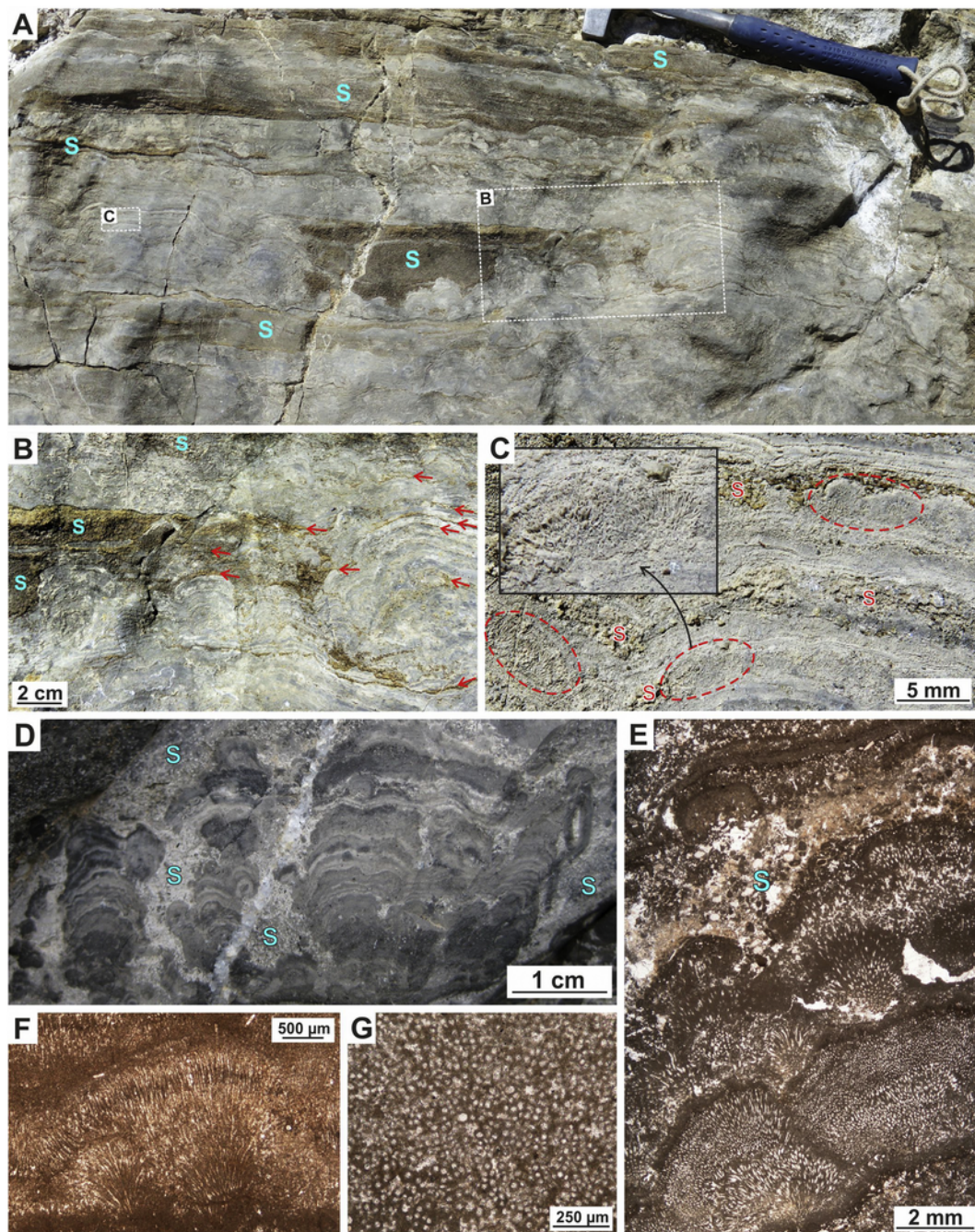
Fig. 8. Skeletal stromatolites of the Leza Fm. An 'S' marks each sandy intercalation between stromatolite levels, domes, columns or laminae. A: Field image of the stromatolite-bearing facies deposited in freshwater bodies with alluvial influence (Fig. 5B). White rectangles mark the location of B and C. B: Detail of A showing domal stromatolites adjacent to sandy levels (S) and including thin sandy intervals between some of their laminae (red arrows). C: Field detail of the stromatolite lamination. Red ovals mark fan-like filamentous colonies easily visible (the black square shows a close-up of one of the colonies). Note that sandy intercalations (S) occur infilling cavities and irregularities within or over the stromatolite laminae (see E). D: Detailed field image of skeletal stromatolites with columnar macrostructure. Note how sandy material (S) fills the space between columns. E: Photomicrograph of the skeletal stromatolites showing the predominant microfabric formed by filamentous fans. Note that sandy intercalations (S) are filling the irregularities over one of the stromatolite laminae. F: Detail of one of the filamentous fan-like colonies that form the skeletal stromatolites. G: Photomicrograph of a thin section cut parallel to stromatolite lamination, showing a transverse section of the filaments. (For interpretation of the references to colour in this figure legend, the reader is referred to the web version of this article.)
