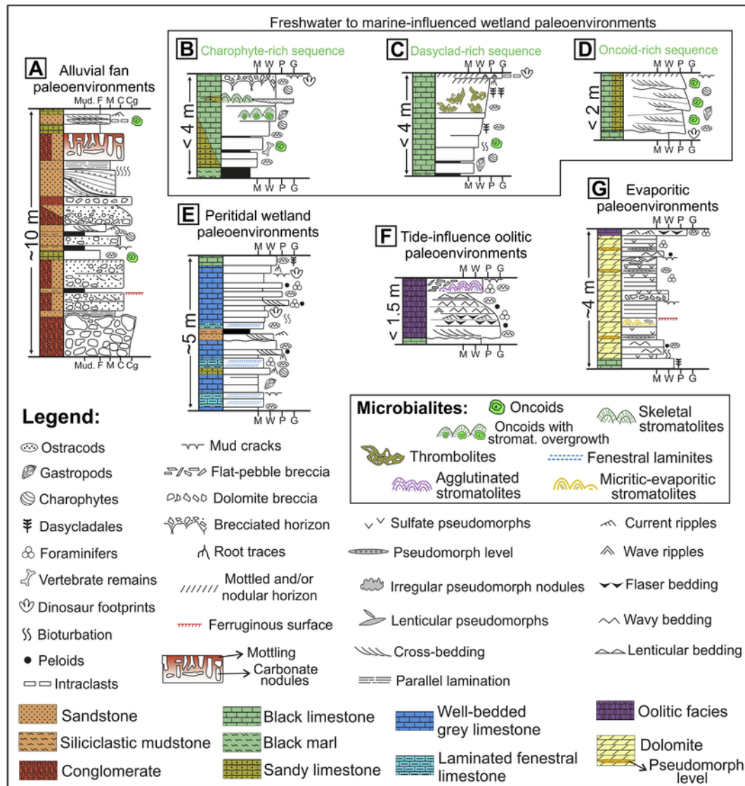
Fig. 5. Schematic logs of the different facies associations of the Leza Fm, with the interpretation of their general paleoenvironments. Modified after Suarez-Gonzalez et al. (2015). The colour-code is equivalent to that of Figs. 2, 4, 5 and 15. A: Facies deposited in alluvial fan paleoenvironments, where oncoids occur. B-D: Facies deposited in freshwater to marine-influenced wetland paleoenvironments. B: Example of a charophyte-rich (i.e. freshwater-dominated) sequence where oncoids and skeletal stromatolites occur. C: Example of a dasyclad-rich (i.e. marine-influenced) sequence where thrombolites occur. D: Oncoid-rich facies deposited in freshwater-dominated creeks. E: Facies deposited in the peritidal wetland paleoenvironments, where fenestral laminites occur. F: Facies deposited in the tide-influenced oolitic paleoenvironments, where agglutinated stromatolites occur. G: Facies deposited in the evaporitic paleoenvironments, where micritic-evaporitic stromatolites occur.
