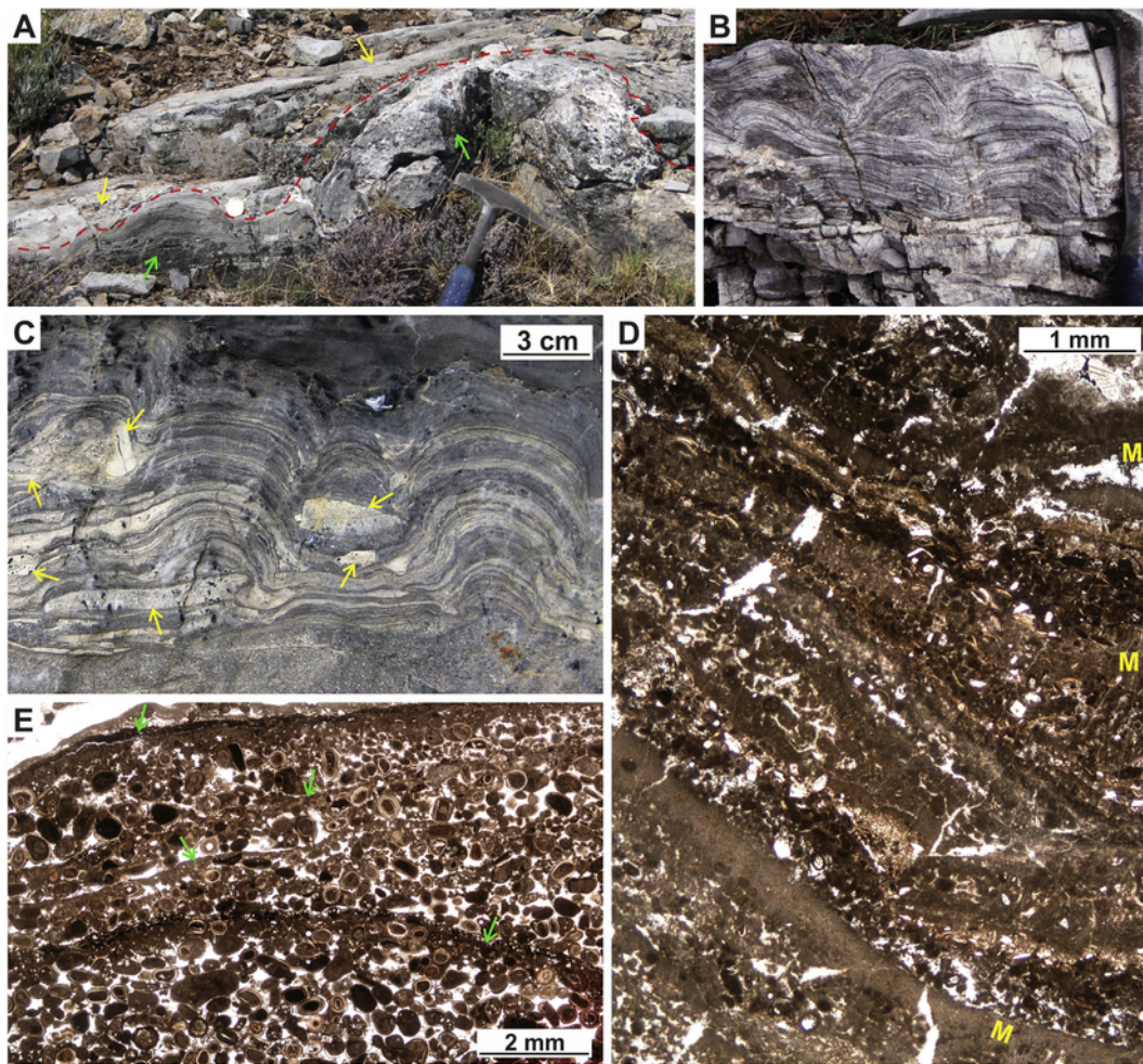
Fig. 10. Agglutinated stromatolites of the Leza Fm. See further images in Suarez-Gonzalez et al. (2014). A: Field view of a stromatolite level (green arrows) with a large dome (right), overlapped by thinly bedded oolitic deposits (yellow arrows). B: Close-up of a stromatolite bed showing stratiform to domal structures and clear thin bedding. C: Domal stromatolite level developed over oolitic deposits and showing clear lamination formed by alternating dark and light laminae. Note large intraclasts included within the stromatolite (yellow arrows). D: Photomicrograph of the side of a stromatolite dome, showing very abundant grains included within the stromatolite laminae, even at steep angles. Laminae dominated by micrite are marked with a yellow M. Note that most laminae have an intermediate composition with both grains and micrite. E: Photomicrograph showing grainy stromatolite laminae separated by thin micritic crusts (green arrows). Note that the crusts are associated to micritization of the grains of the underlying laminae. Compare with micritic crusts of modern agglutinated microbialites (Fig. 1H–I). (For interpretation of the references to colour in this figure legend, the reader is referred to the web version of this article.)
