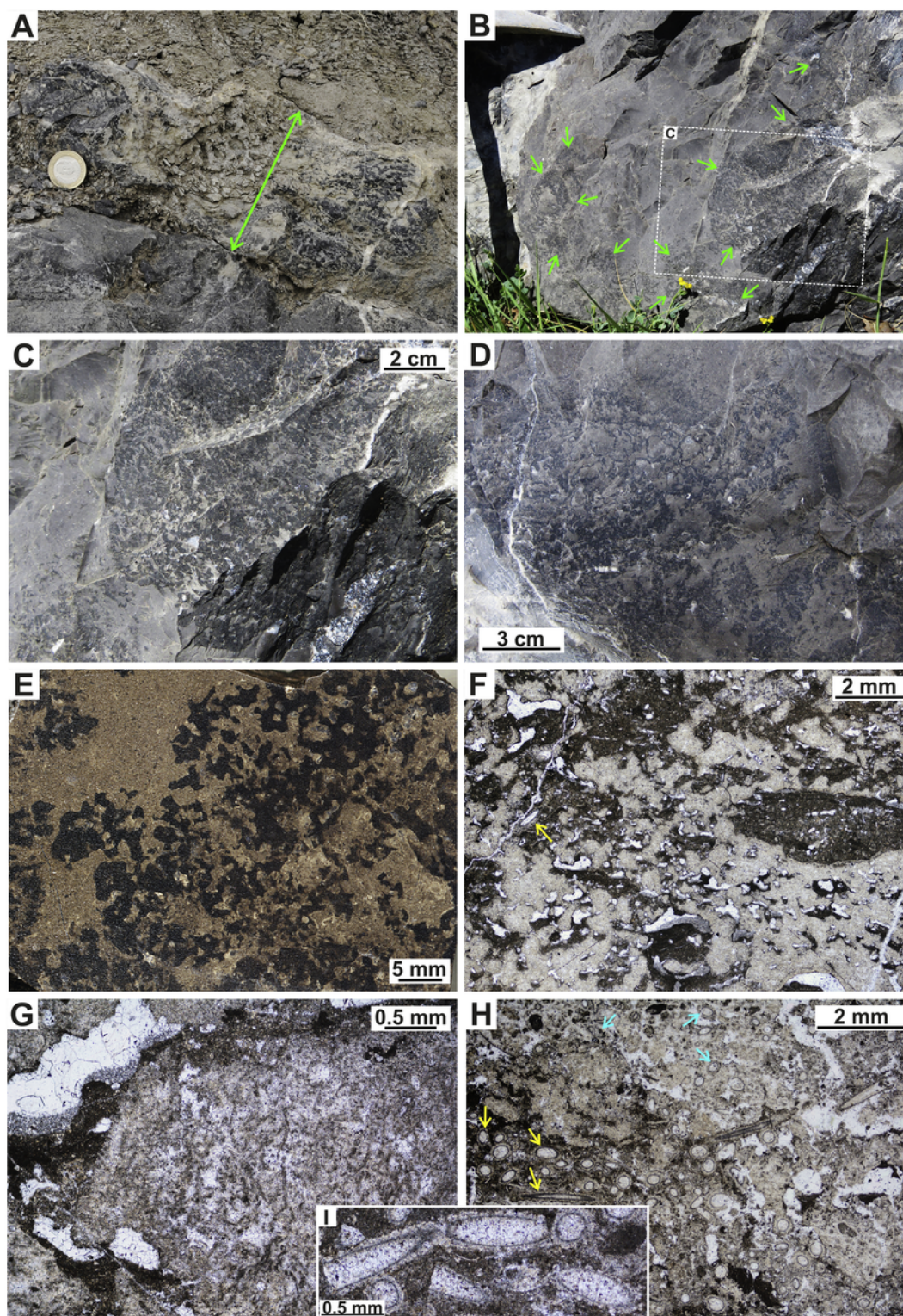
Fig. 7. Thrombolites of the Leza Fm. A: Field image of a thrombolite occurring as a laterally-continuous bed (biostrome). Green arrow marks bed thickness. Coin diameter is 23 mm. B: Field image of thrombolites (green arrows point to their margins) occurring as irregular masses (bioherms) within thicker beds (Fig. 5C). White rectangle marks the location of C. Tip of hammer at the top left for scale. C: Field image of the macroscopic features of thrombolites, showing the characteristic mesoclots (dark colour) and large irregular fenestrae (light colour). D: Field image of the macroscopic features of thrombolites. Note the upwards-elongated distribution of mesoclots suggesting vertical growth. E: Polished hand specimen showing the mesostructure of thrombolites and the characteristic irregular interconnected mesoclots (black) and the surrounding sediment (brown) filling fenestrae between the mesoclots. F: Photomicrograph showing a detail of the thrombolite mesostructure with irregular mesoclots (light brown) and fenestrae filled with sediment (dark brown) and/or cement (white). Note many fenestrae with geopetal fillings. Yellow arrow points to a dasycladal. G: Detail photomicrograph of a mesoclot, showing clotted-peloidal microfabric with poorly-preserved filamentous structures. Note geopetal cavities to the left. H: Photomicrograph of a thrombolite sample very rich in dasyclads, both in the sediment-filled fenestrae (dark colors, dasycladales pointed by yellow arrows) and within the mesoclots (light colors, dasycladales pointed by red arrows). I: Detail photomicrograph of the dasycladales. (For interpretation of the references to colour in this figure legend, the reader is referred to the web version of this article.)
