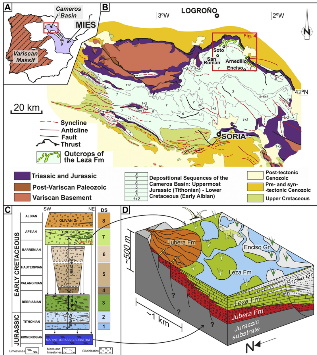
Fig. 3. Geological setting of the case study presented in this work. A: Simplified geological map of the Iberian Peninsula, highlighting the location of the Cameros Basin within the Mesozoic Iberian Extensional System (MIES). B: Geological map of the Cameros Basin (modified after Mas et al., 2011) highlighting in green the outcrops of the Leza Fm, at the northern margin of the basin. Red square marks the location of the map included in D and in Fig. 4. C: Litho-chronostratigraphic chart of the eastern area of the Cameros Basin, modified after Mas et al. (2011). DS: depositional sequences. D: Reconstruction of the stratigraphic and paleogeographic relationships of the case study presented here (Leza Fm) with its adjacent units (see Fig. 3C), showing that the Jubera and Leza Fms are associated with the faulting and erosion of the Jurassic substrate of the basin. Modified after Suarez-Gonzalez et al. (2013). (For interpretation of the references to colour in this figure legend, the reader is referred to the web version of this article.)
