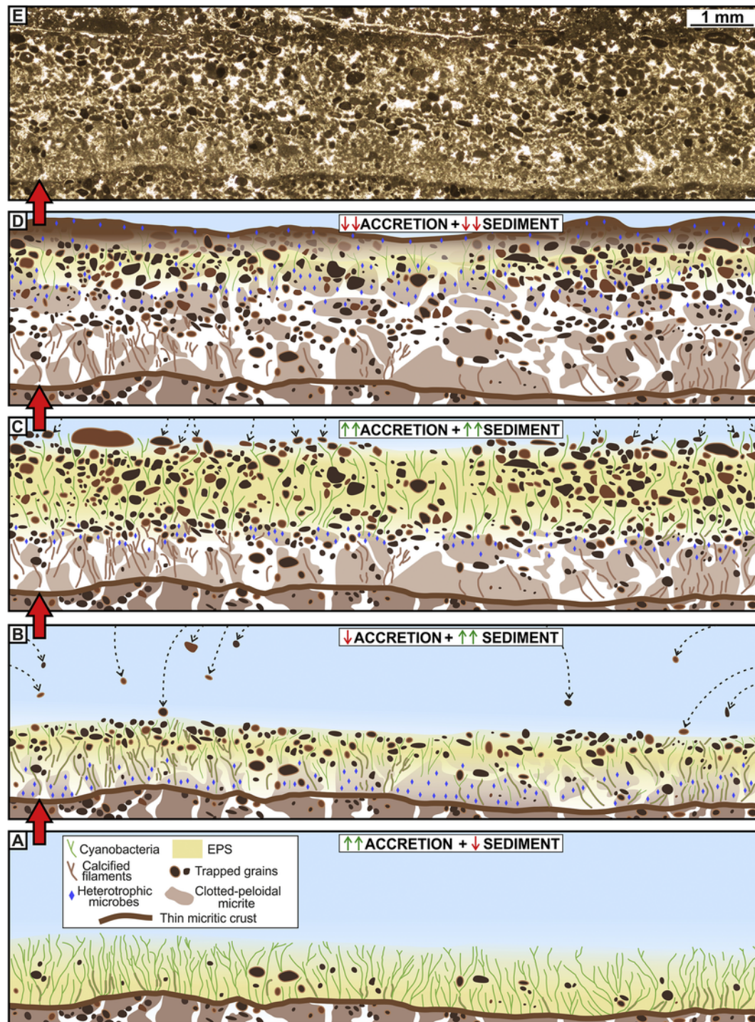
Fig. 12. The detailed analysis of stromatolite laminae reveals, even at the small temporal and spatial scale of a single lamina, the complex interplay between microbial accretion and sediment supply that produces the microfabrics of the Leza Fm agglutinated stromatolites, which are strikingly similar to those of modern analogues (Fig. 1F–I). A: During some periods, a benthic microbial community could accrete on the stromatolite surface even with relatively low sediment supply. If early calcification occurred locally, some filament remains would eventually be preserved. B: During periods of low microbial accretion relative to the sediment supply, thin levels especially rich in grains developed. C: When the rates of microbial accretion and grain supply were balanced, grainy levels were recorded. Meanwhile, precipitation of clotted-peloidal micrite could start in underlying parts of the microbial community, probably induced by the degradation of EPS by heterotrophic microbes. D: Interruption periods of both microbial accretion and grain supply are recorded by thin micritic crusts caused by intense microbial activity at the top of the microbial community, which induced micritization and truncation of underlying grains and micrite precipitation. E: Photomicrograph of the final result in the fossil record.
