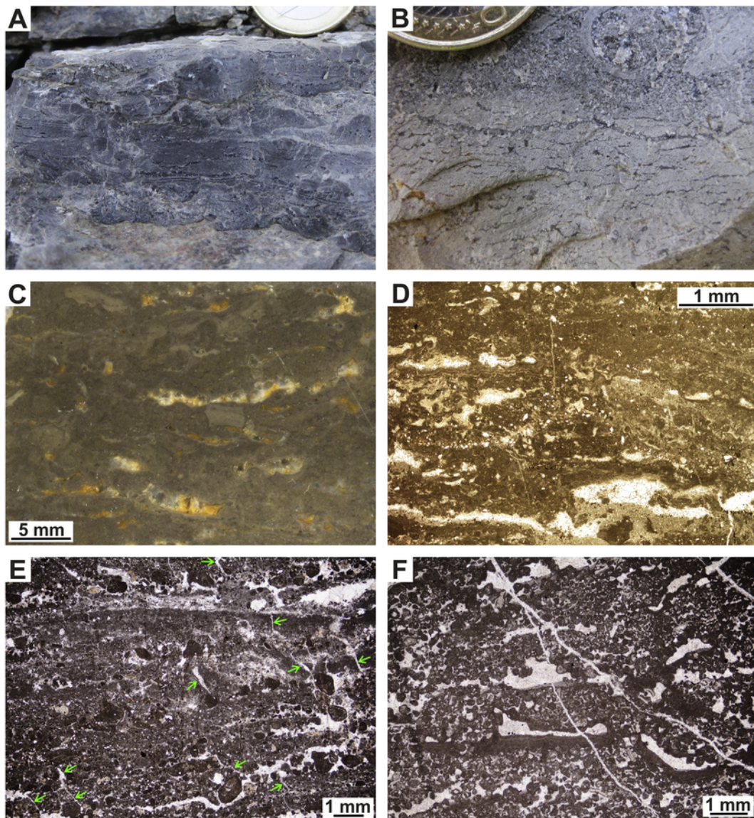
Fig. 14. Fenestral laminites of the Leza Fm. A: Field view of a thin level of fenestral laminites. B: Close-up view of fenestral lamintes, showing the thin lamination formed by horizontally elongated fenestrae (darker colors). C: Polished slab of fenestral laminites showing the irregular, horizontal, cement-filled fenestrae (white, gray and yellow colors). D: Photomicrograph showing fenestrae (light colors, some of them with darker geopetal fillings) and the micritic texture of the laminae, some of them including grains (mainly quartz). E: Photomicrograph of grain-rich microfabrics of the fenestral laminites. Green arrows point to subvertical cracks (some of them V-shaped) in many laminae. F: Photomicrograph showing stromatolite-like fenestrae, some of them with geopetal fillings. (For interpretation of the references to colour in this figure legend, the reader is referred to the web version of this article.)
