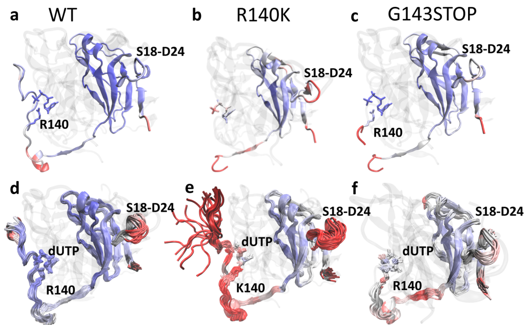
Figure 2. Flexibility and disorder of mtDUT and its mutants affecting the Arg finger and the P-loop-like elements from crystallographic structures (top) and MD simulations (bottom). Cartoon representation is shown of the (a) wild type mtDUT (PDB: 2PY4), (b) mtDUT R140K,H145W , and (c) mtDUT G143STOP structures. The local thermal motions defined by B factors in crystal structures (upper row, a–c) are compared with the observed flexibility in MD simulations (lower row, d–f). The superposition of MD simulation snapshots collected at uniform intervals is shown. The disordered C-terminal region and the loop S18–D24 are highlighted; the dUTP and the R/K140 are shown as licorice. Color code: blue, more rigid; red, more flexible. Only one dUTPase protomer is highlighted with the other two protomers shown as transparent.
