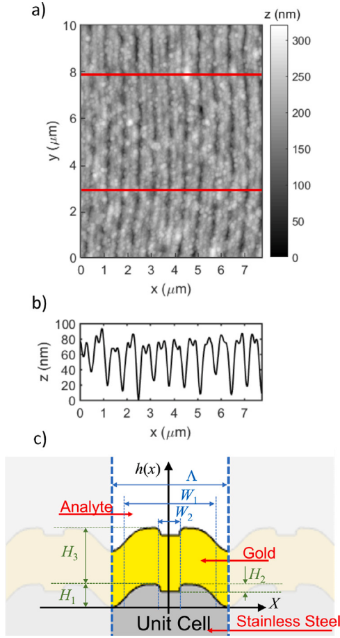
Fig. 3. (a) AFM scanning of a region of the fabricated sample. (b) Average profile of the LIPSS between the red lines in (a). (c) Profile used in the simulations.
