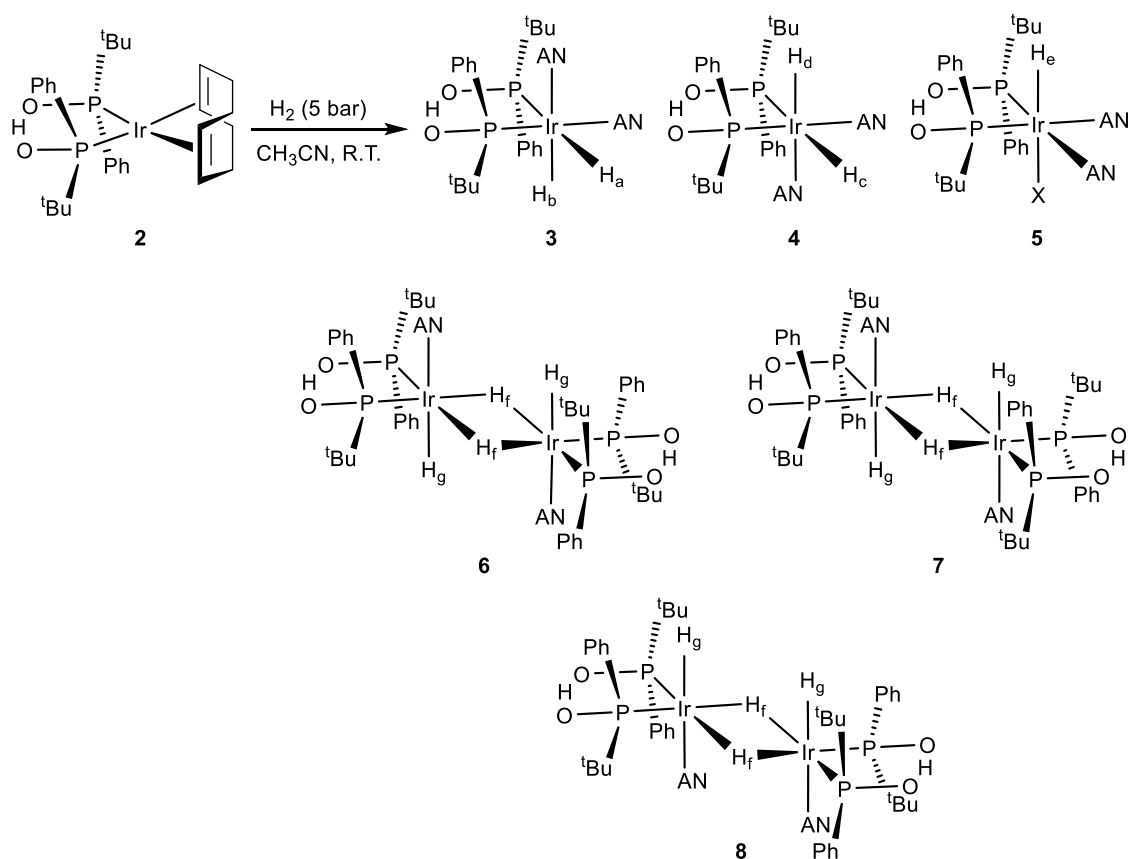
Scheme 2. Formation of Iridium (III) hydride species under substrate-free hydrogenation conditions.
