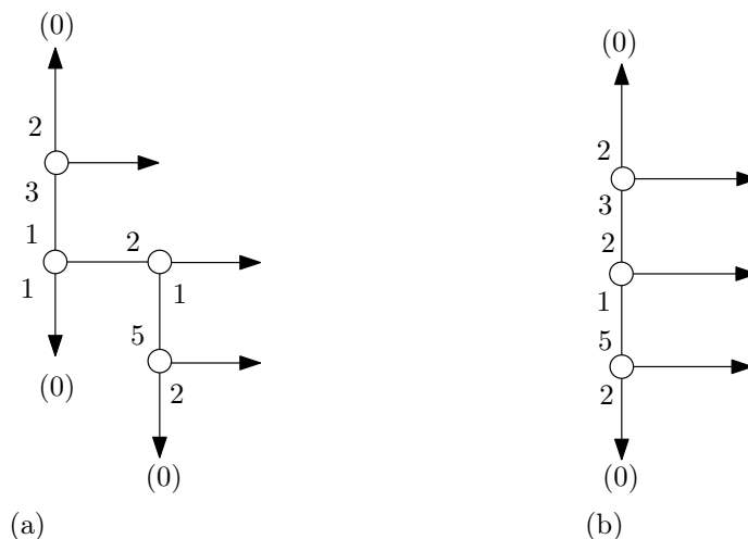
FIGURE 4. Newton tree in suitable coordinates and not P-good
