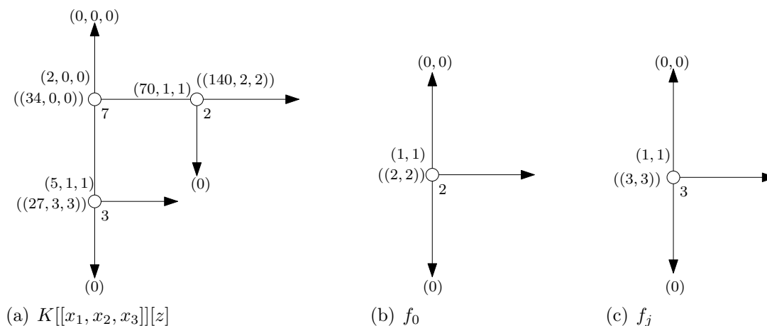
FIGURE 7. Newton trees of Example 5.5.
