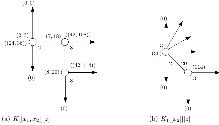
FIGURE 9. Newton trees of Example 5.7.
