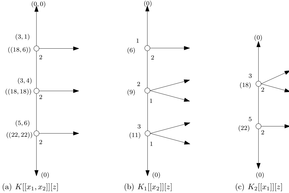
FIGURE 6. Newton trees of Example 5.2
