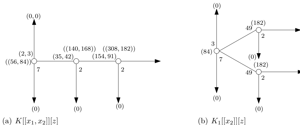
FIGURE 8. Newton trees of Example 5.6.
