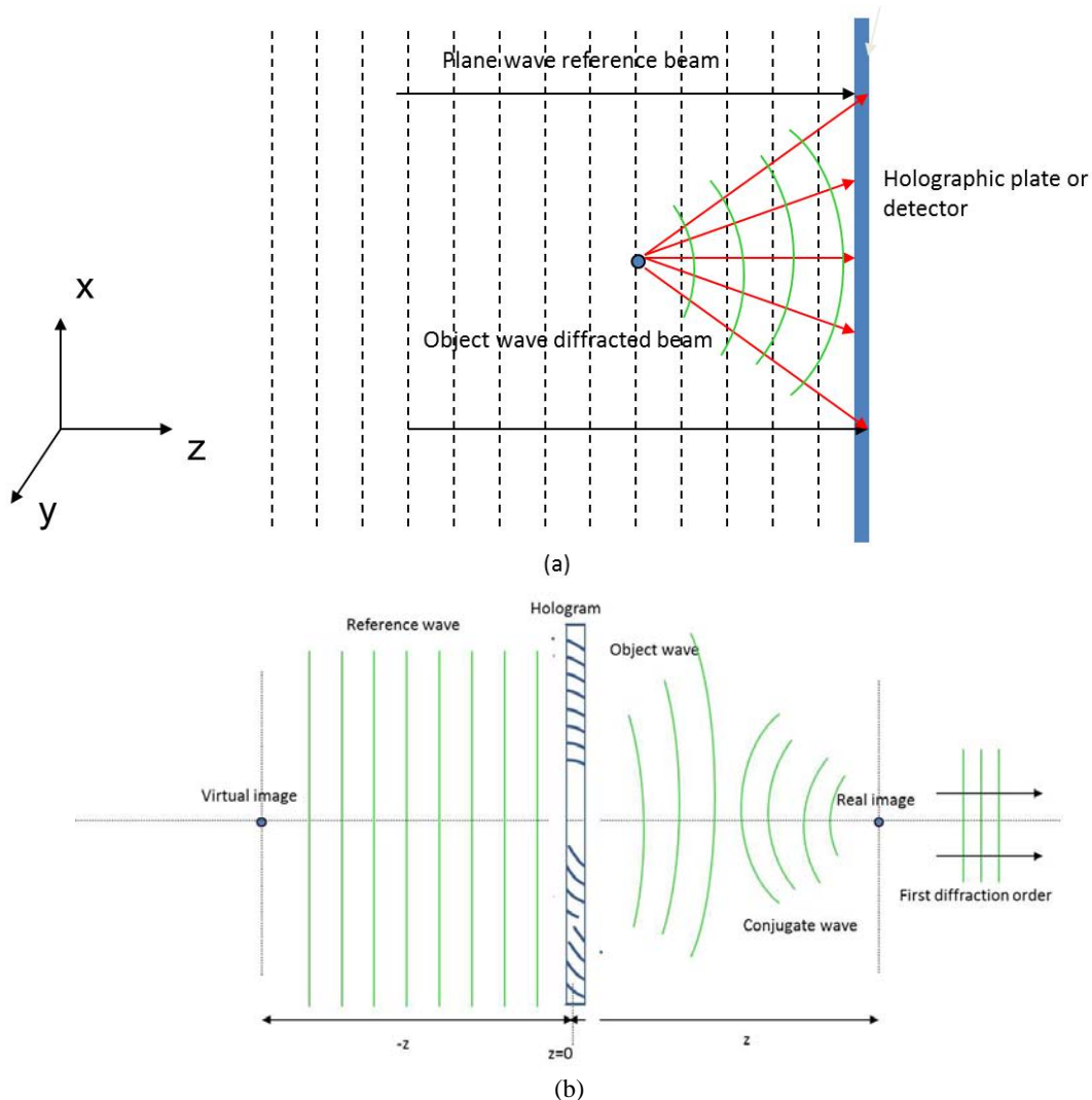
Figure 1.- (a) Recording of the hologram of an ideal point source. (b) Reconstruction, two twin point source images are formed. See text for details
