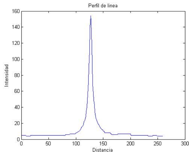
Figure 4 .- (a) Pattern of the projected laser beam onto the white screen, captured by the mobile phone (NOKIA X3-02, see text for details), propagation distance 3m. (b) Line profile of the corresponding image. Abscissa horizontal line indicates the selected location for obtaining the line profile. Distance is measured in number of pixels.
