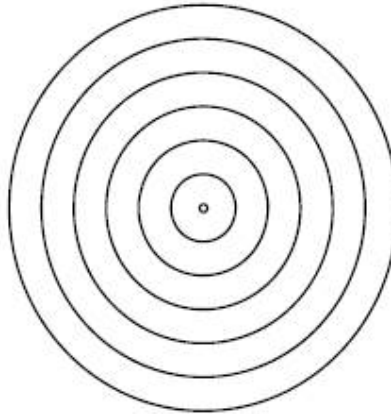
Figure 2.- Structure of the recorded hologram whose transmittance amplitude is represented in ec. (8). This is the so named Fresnel Zone Plate (FZP) and gives the ideal structure as recorded by the camera phone.
