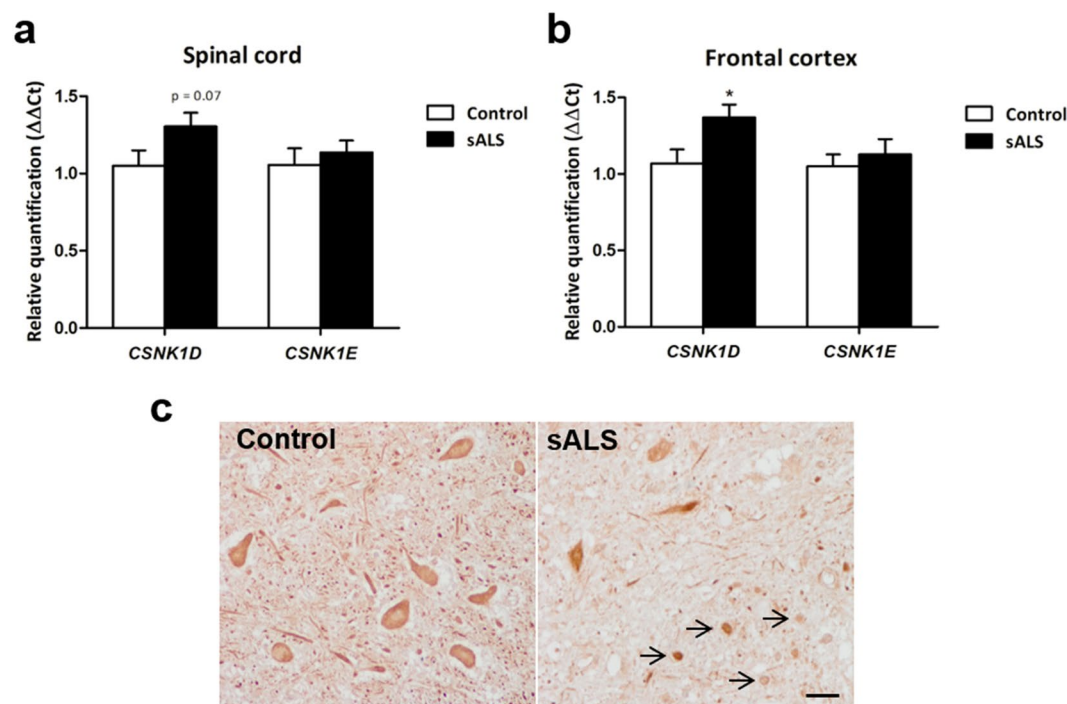
Figure 6. Relative expression of CSNK1D and CSNK1E mRNA levels in post-mortem samples from control and ALS subjects and immunohistochemical analysis. (a) CSNK1D and CSNK1E mRNA levels in the anterior horn of the spinal cord and (b) frontal cortex area 8 of sALS cases and controls, *p < 0.05 . (c) CK-18 immunoreactivity in the anterior horn of the spinal cord at lumbar level in control and ALS cases showing CK-18 immunoreactivity in the cytoplasm of neurons and neuronal processes in control. Similar reaction is found in the remaining motor neurons in devastated anterior horn in the ALS case together with increased CK-18 immunoreactivity in reactive glial cells (arrows). Paraffin sections, slightly counterstained with haematoxylin; scale bar = 25 \mu m.
