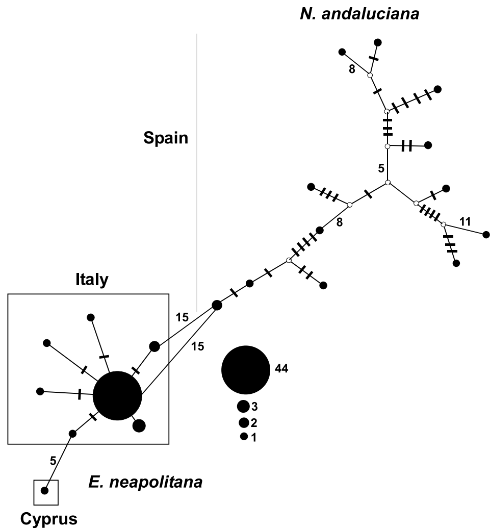
Fig. 5 Haplotype network based on 28S. Each black circle represents a different haplotype; their size is proportional to the number of samples belonging to that haplotype. Each perpendicular line indicates a mutational step, if there were more than four it is shown with the number of mutational steps. White circles are hypothetical intermediate haplotypes. Branch length does not contain any information
