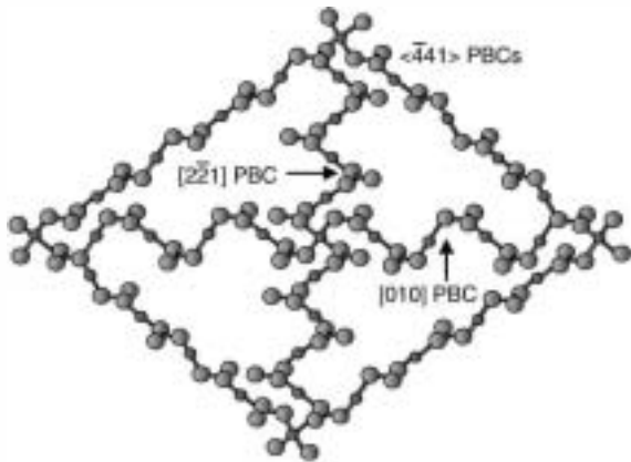
Fig. 1. Schematic illustration showing the three non-equivalent PBCs contained in the calcite \{10\bar{1}4\} face: two non-parallel \langle 441 \rangle PBCs, which define the edge of the rhombohedron, and the PBCs \langle 221 \rangle and \langle 010 \rangle parallel to the short and long diagonals. The straight PBCs parallel to \langle 441 \rangle are the most stable, while the undulated PBCs parallel to \langle 221 \rangle and \langle 010 \rangle have a higher energy and are less stable. The growth layers will be bounded by the most stable steps, i.e. those parallel to \langle 441 \rangle . (After Paquette and Reeder, 1995).
