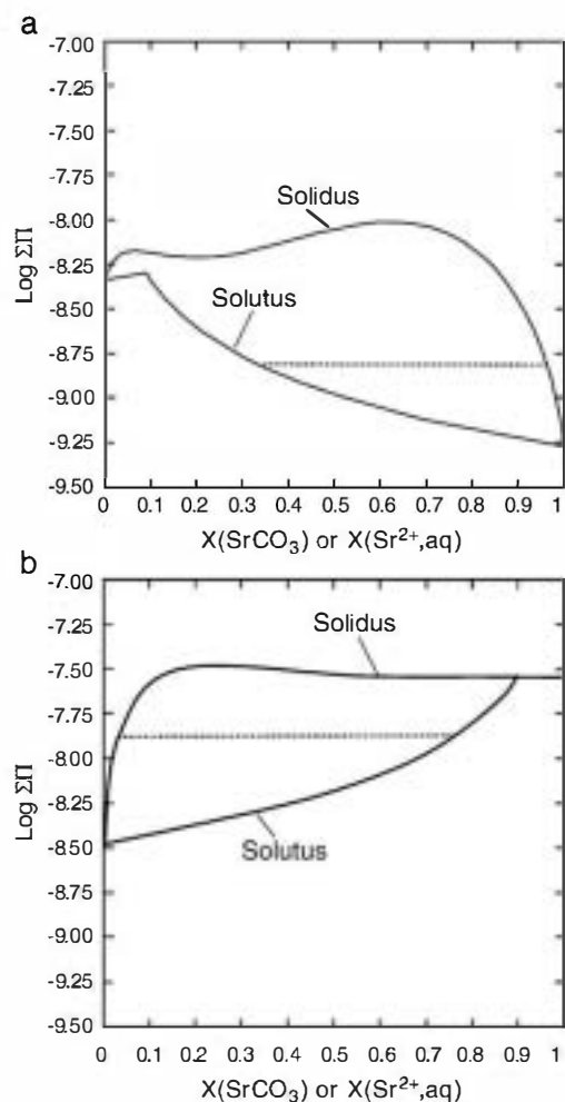
Fig. 3. Lippmann phase diagrams for the (\text{Ca,Sr})\text{CO}_3 solid solution-aqueous solution systems at 25 °C: (a) (\text{Ca,Sr})\text{CO}_3\text{-H}_2\text{O} system. The diagram was constructed assuming a subregular solid solution model with Redlich-Kister coefficients \alpha_0=3.43 and \alpha_1=-1.82 ; (b) (\text{Ca,Sr})\text{CO}_3\text{-H}_2\text{O} system (Plummer and Busenberg, 1987). Diagram constructed considering a hypothetical regular solid solution model ( \alpha_0=2.6 ; Böttcher, 1997). In both diagrams, dotted tie lines connect solid-solution equilibrium pairs.
