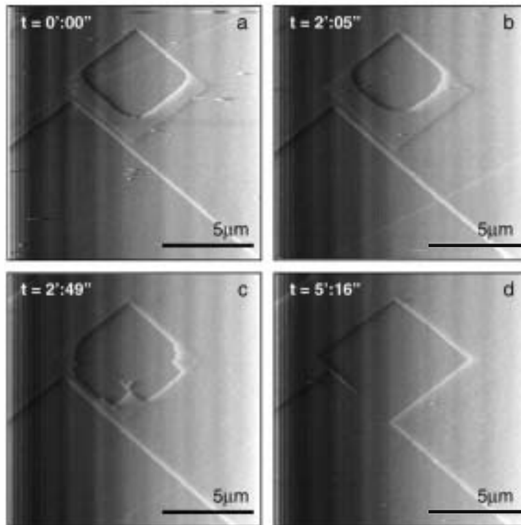
Fig. 7. AFM growth sequence on a calcite \{10\bar{1}4\} surface in contact with a solution supersaturated with respect to calcite ( \beta_{\text{calcite}}=5 ); [\text{Sr}]=4.0 mmol/l (without flow). (a–b) The incorporation of Sr into the structure causes the thickening of advancing steps. (c–d) After some minutes, dissolution starts and the retreat of both the newly and the original steps can be observed. The time of the sequence is 316 s.
