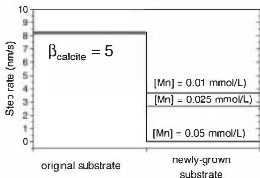
Fig. 14. Step advancement rates in contact with solutions supersaturated with respect to calcite ( \beta_{\text{calcite}} ) and different concentrations of Mn. The higher the Mn in solution the more effective is the effect of the newly formed substrate in inhibiting the subsequent step advancement, and the more exact is the reproduction of the pre-existing topography.
