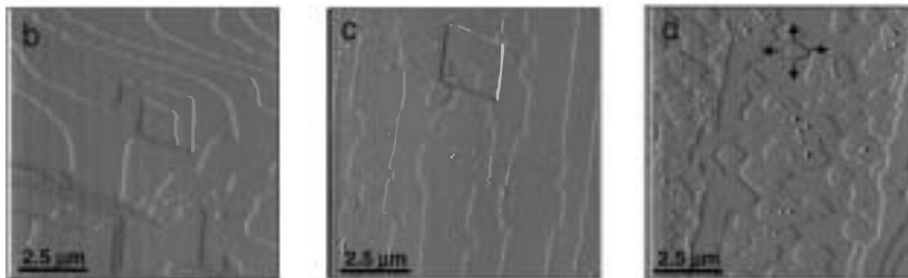
Fig. 10. (a) Supersaturation functions, \beta(X_{\text{MnCO}_3}) , for the solutions 1, 2 and 3 calculated using Eq. (4) for the system (\text{Ca},\text{Mn})\text{CO}_3\text{-H}_2\text{O} . (b-d) Microtopography of the \{10\bar{1}4\} surfaces growing from solutions 1, 2 and 3, observed by AFM. The observation of step advancement for solution 1 and 2 and two-dimensional nucleation only for solution 3 allows to draw the \beta^* line i.e., the variation of the transitional supersaturation between step advancement and two-dimensional nucleation as a function of the solid composition.
