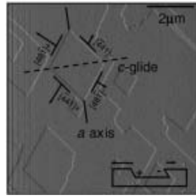
Fig. 2. AFM image of a calcite \{10\bar{1}4\} surface in water. On the dissolution pits, four non-equivalent steps parallel to \langle 441 \rangle_+ and \langle 441 \rangle_- , as well as the a -axis and the c -glide trace are indicated. Steps parallel to [\bar{4}41]_- and [48\bar{1}]_- , i.e. those steps with constrained kink sites, exhibit a slow retreating speed, while those parallel to [\bar{4}41]_+ and [48\bar{1}]_+ retreat rapidly. The growth of this surface shows similar characteristics to dissolution, also occurring by a layer-by-layer mechanism with a clearly anisotropic advancement of monomolecular steps. Those steps parallel to [\bar{4}41]_- and [48\bar{1}]_- advance slowly while [\bar{4}41]_+ and [48\bar{1}]_+ advance rapidly. Such a coincidence reflects the crystallographic control of both processes.
