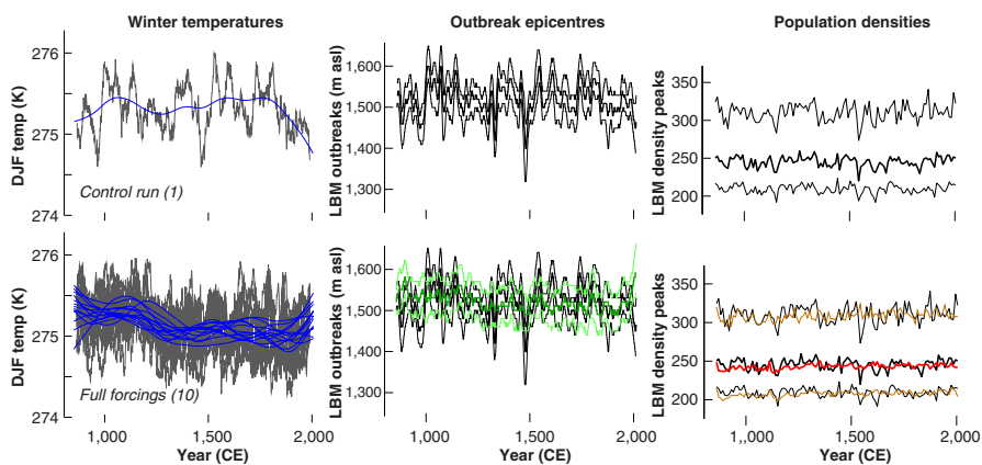
FIGURE 2 Control run and the fully forced simulations of December–February temperature means over the European Alps (blue lines are 30-year splines; left). Elevational changes in larch budmoth (LBM) outbreak epicentres (mean \pm 1 SD) under the different climate simulations (middle), and the corresponding LBM population densities at cycle peaks (mean \pm 1 SD; right). Outbreak epicentre and density peaks for full forcing simulations (green) are overlaid on those from control simulations (black) for comparison (bottom row, middle and right)
