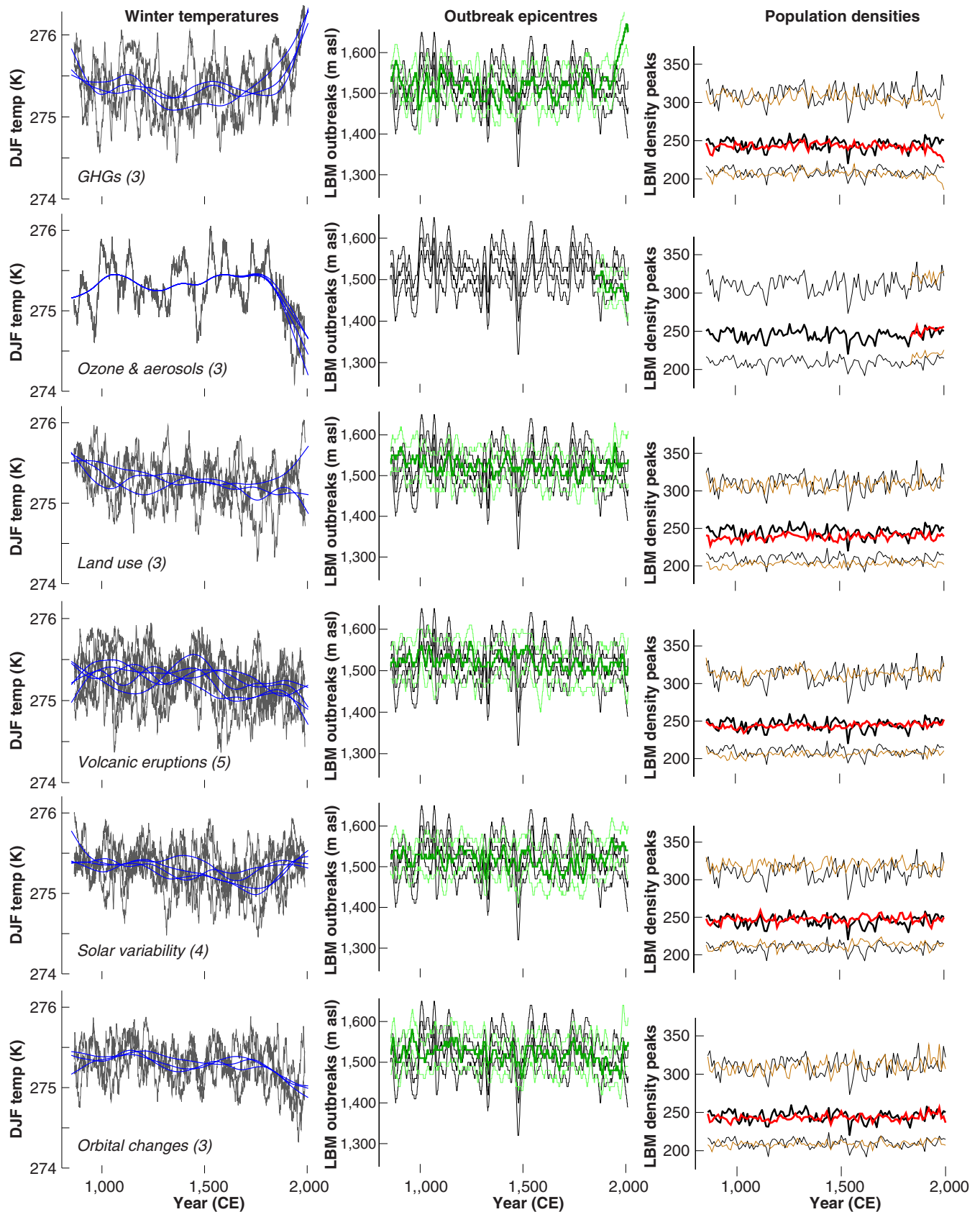
FIGURE 3 Single forcing simulations of Alpine winter temperatures (blue lines are 30-year splines; left). Elevational changes in larch budmoth (LBM) outbreak epicentres under different climate simulations (mean \pm 1 SD; middle), and corresponding LBM population densities at cycle peaks (mean \pm 1 SD; right). Outbreak density peaks for single forcing simulations (green, red) are overlaid on control simulations (black). Ozone and aerosol runs are reliable after 1850 CE
