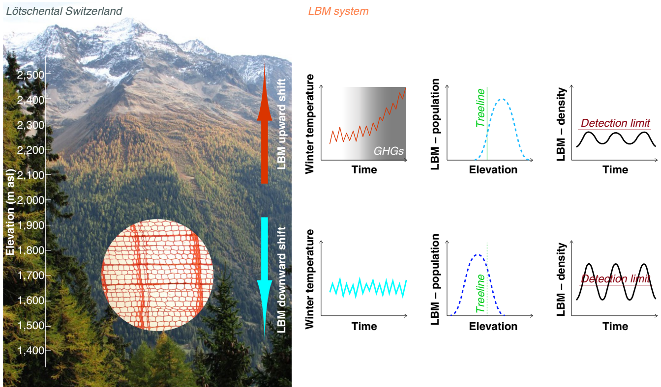
FIGURE 1 South-exposed slope of the Lötschental (c. 46^\circ 29'N and 8^\circ 17'E ), the largest northern side valley of the Rhone valley in the western Swiss Alps (Büntgen, Frank, Nievergelt, & Esper, 2006), where cyclic population outbreaks of the larch budmoth (LBM; Zeiraphera diniana or griseana Gn.) defoliate the subalpine larch forest every 8–9 years (Esper et al., 2007), and leave distinct growth depressions in the host's tree rings (inset circle; Büntgen et al., 2009). Anthropogenic winter warming causes substantial upward elevational range shifts in LBM outbreak epicentres that suppress the insect's population peak density below a certain detection threshold (upper sketch line). No such effects occur under stable temperatures without greenhouse gas or other external forcing, because the LBM system is best known for its persistent regular behaviour (lower sketch line)
