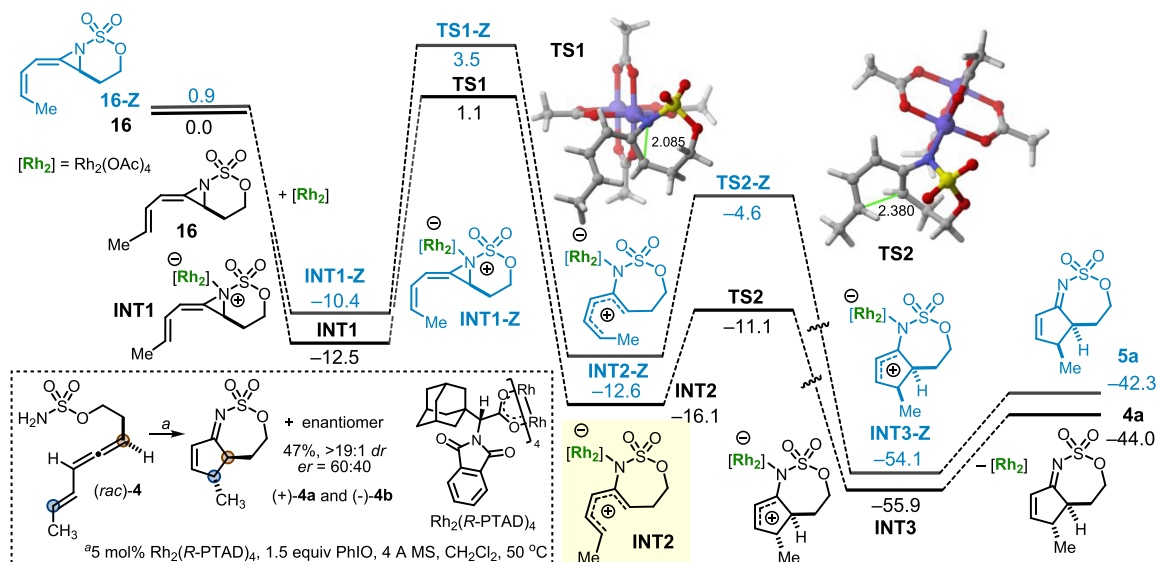
Figure 1. Computed reaction profile for the 2-imino-Nazarov reaction of aziridine 16 . Relative energies and bond distances are given in kcal/mol and angstroms, respectively. All of the data were computed at the SMD(CH 2 Cl 2 )-B3LYP-D3/def2-TZVPP//SMD(CH 2 Cl 2 )-B3LYP-D3/def2-SVP level.
