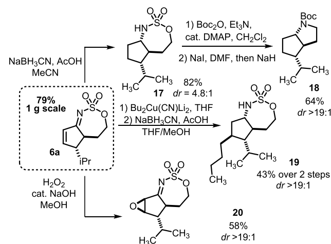
Scheme 2. Flexible Transformations of 6a
