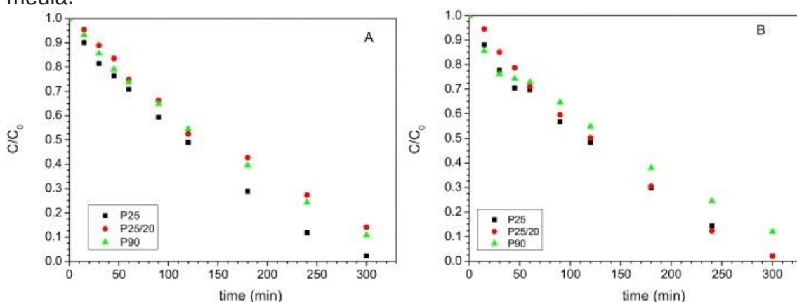
Fig. 8. Evolution of relative phenol concentrations without (A) and after sonication pre-treatment (B).
