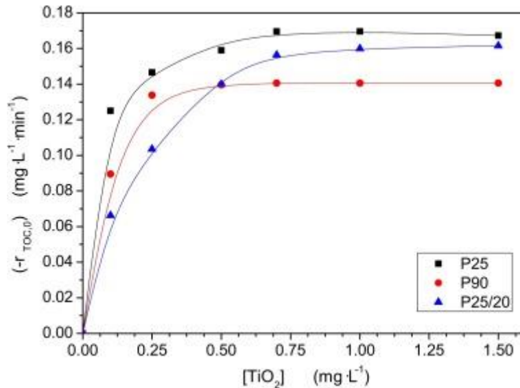
Fig. 3. Influence of TiO 2 catalyst concentration on initial TOC photodegradation rate. Operating conditions: [phenol] 0 = 50 mg L -1 , pH 0 = 6.0, irradiance = 38.4 W m -2 , Q aire = 75 mL N min -1 .
