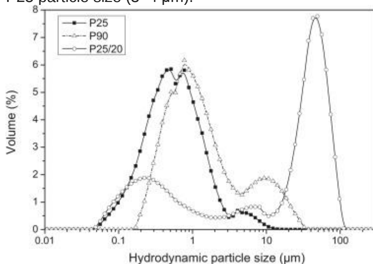
Fig. 7. Hydrodynamic particle size distributions of sonicated \text{TiO}_2 photocatalysts in aqueous suspensions.
