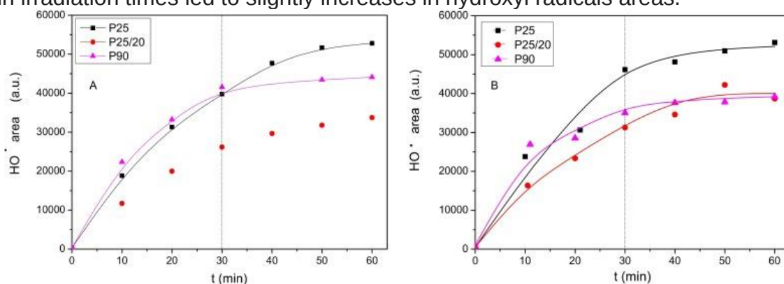
Fig. 9. Evolution of \text{HO}\cdot radical generation without (A) and after sonication pre-treatment (B).
