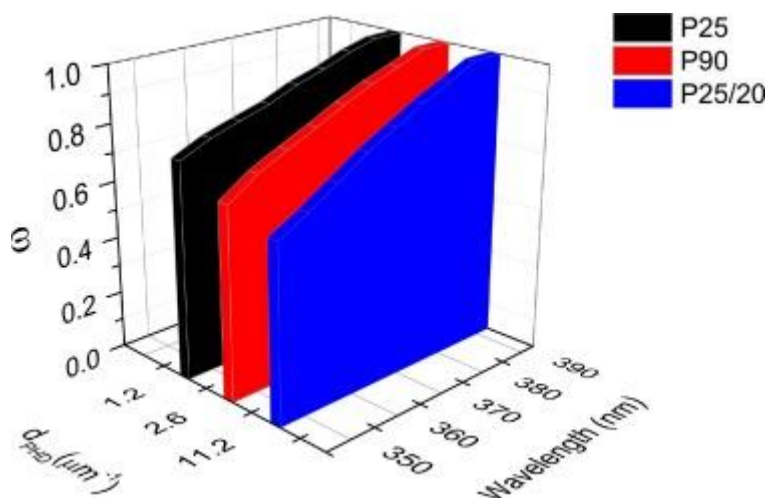
Fig. 4. Albedo coefficient at \lambda = (345\text{--}390) nm, with mean diameter of hydrodynamic particle in aqueous suspensions ( d_{\text{PHD}} ).
