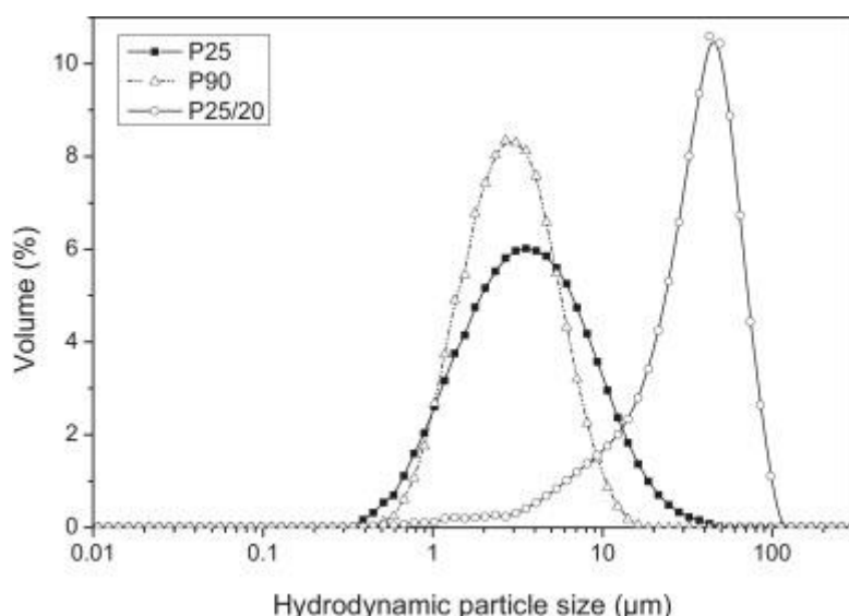
Fig. 2. Hydrodynamic particle size distributions of original \text{TiO}_2 photocatalysts in aqueous suspensions.
