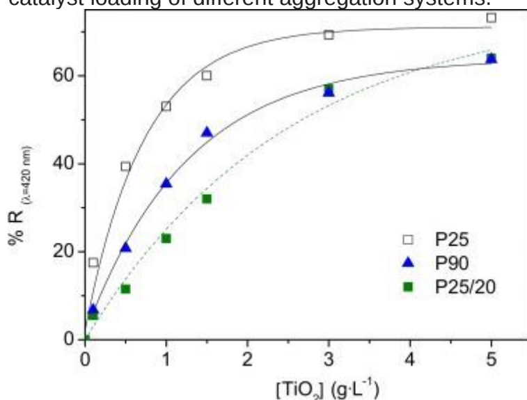
Fig. 5. Extinction of the light in function of the concentration of \text{TiO}_2 catalysts in aqueous suspension.
