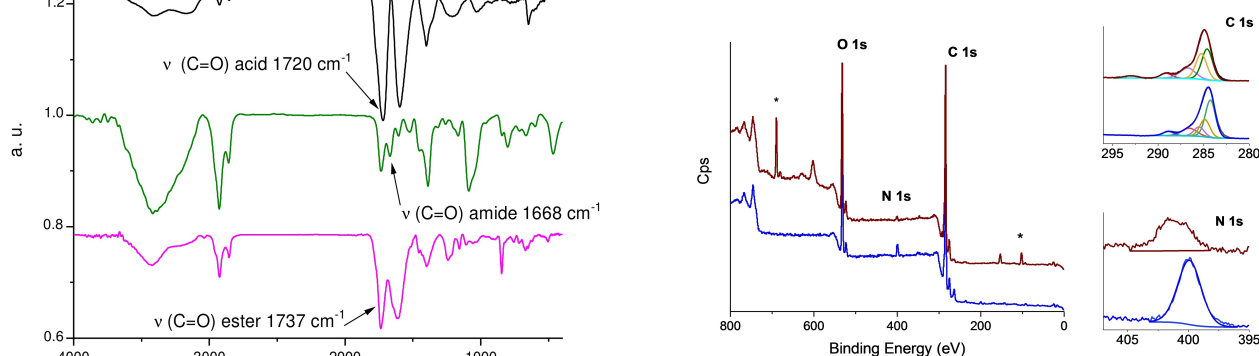
Figure 3. XPS survey spectra of GQDs-1(R) (blue) and GQDs-sup 1(R) (brown). The insets detail the C 1s and N 1s peaks deconvolutions. Highlighted with an asterisk are the XPS peaks of Si 2p (102.5 eV) and F 1s (690.5 eV) from the sample holder.
