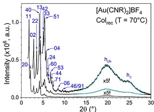
Fig. 4 S/WAXS pattern of [\text{Au}(\text{CNR})_2]\text{BF}_4 ( 4 ), recorded at 70^{\circ}\text{C} , chosen as a representative example. S/WAXS patterns of the other compounds and the complete indexation table can be found in the SI (Table S1 and Fig. S32).
