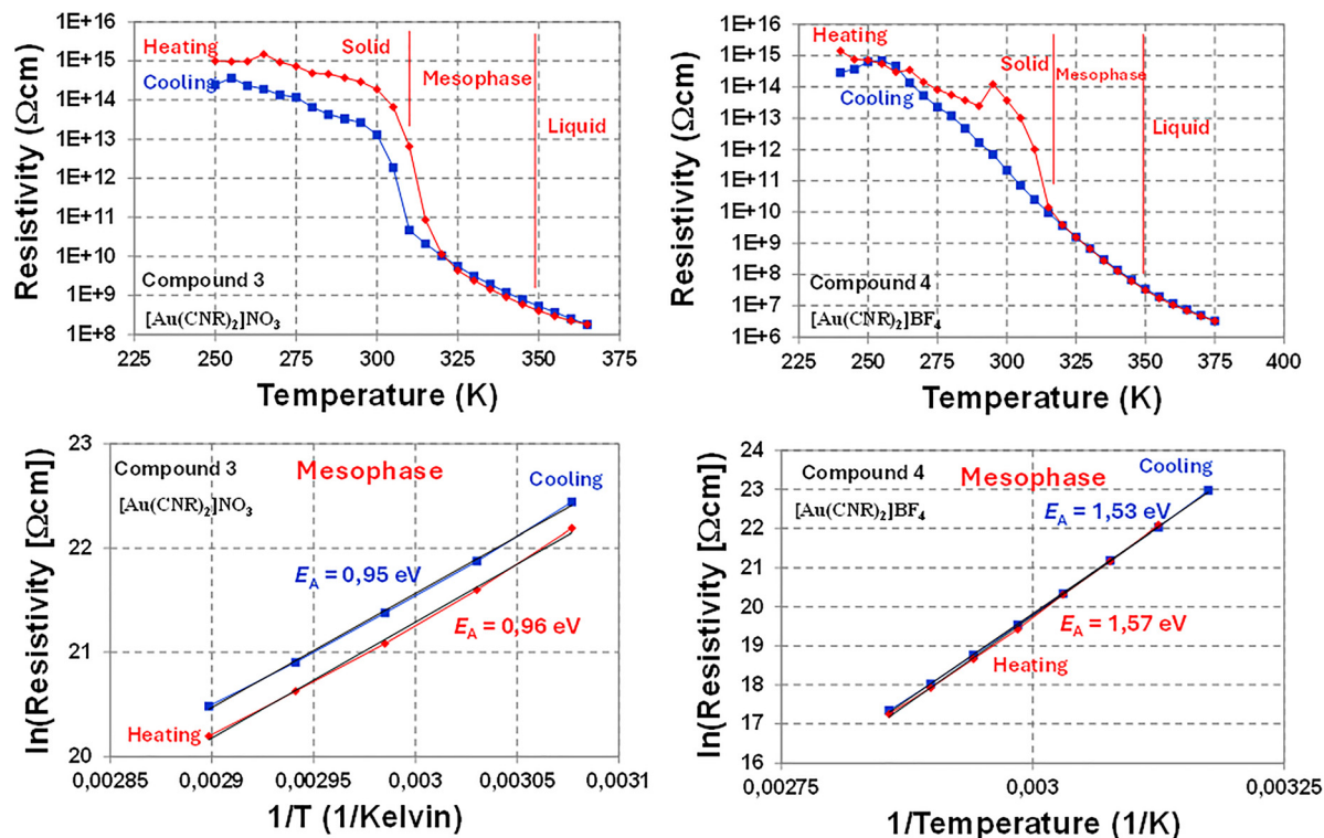
Fig. 8 Resistivity ( \Omega\text{ cm} ) vs. temperature ( T ) plots upon heating (red symbols and lines) and upon cooling (blue symbols and lines) for compounds 3 and 4 . In the lower panels, the data are plotted on Arrhenius axes for the temperature ranges only where the compound is in the mesophase.
