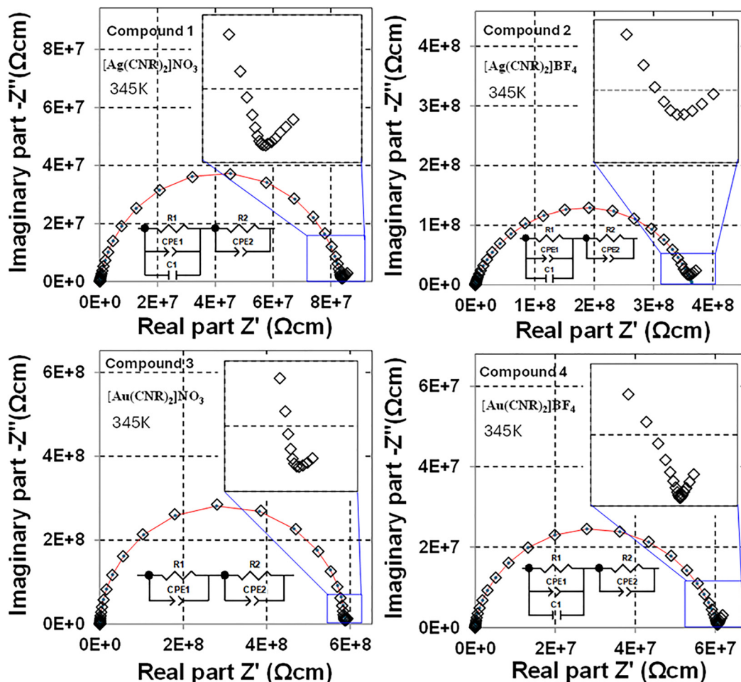
Fig. 6 Complex impedance plane plots of imaginary vs. the real part of the impedance Z'' vs. Z' at 345 K in the mesophase for all compounds 1–4, expressed in specific units of resistivity \rho ( \Omega cm). Open diamond symbols correspond to the data, small blue dots and red lines represent equivalent circuit fits using the circuit models displayed below each semicircle.
