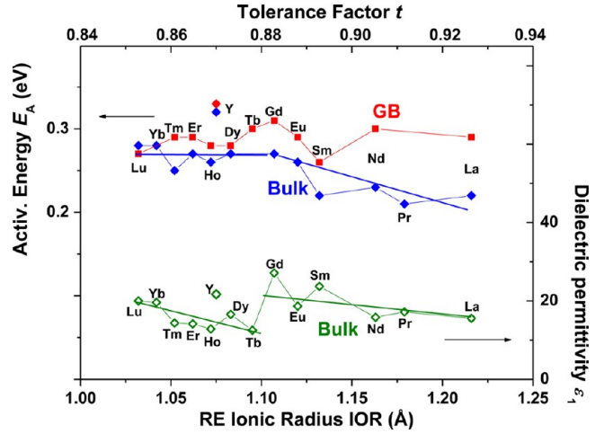
Figure 11. B and GB charge-transport activation energies E_A and bulk dielectric permittivity \epsilon_1 plotted versus IOR and the perovskite tolerance factor.
