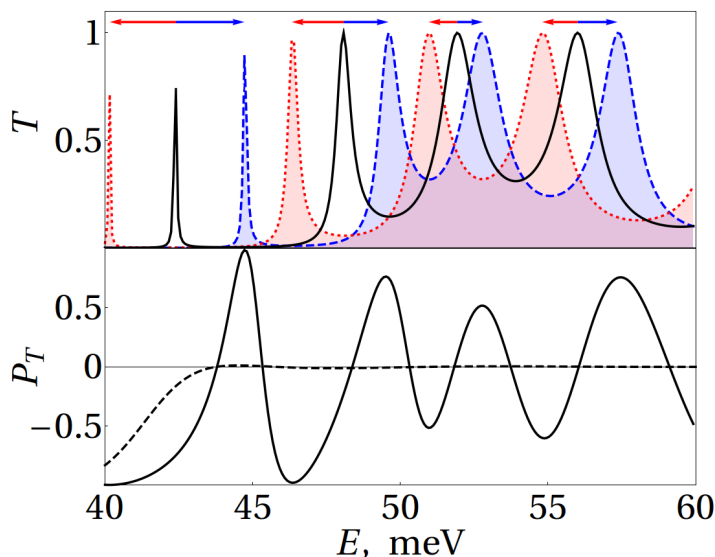
Figure 3. Upper panel shows the transmission coefficient calculated without the exchange splitting (solid black line) and with it (dotted red and dashed blue lines correspond to T_+ and T_- , respectively). Lower panel shows the degree of the transmission polarization P_T of the nanoring (solid line) and that of a single nanoribbon (dashed line). All quantities are calculated at U_G = 0 .
