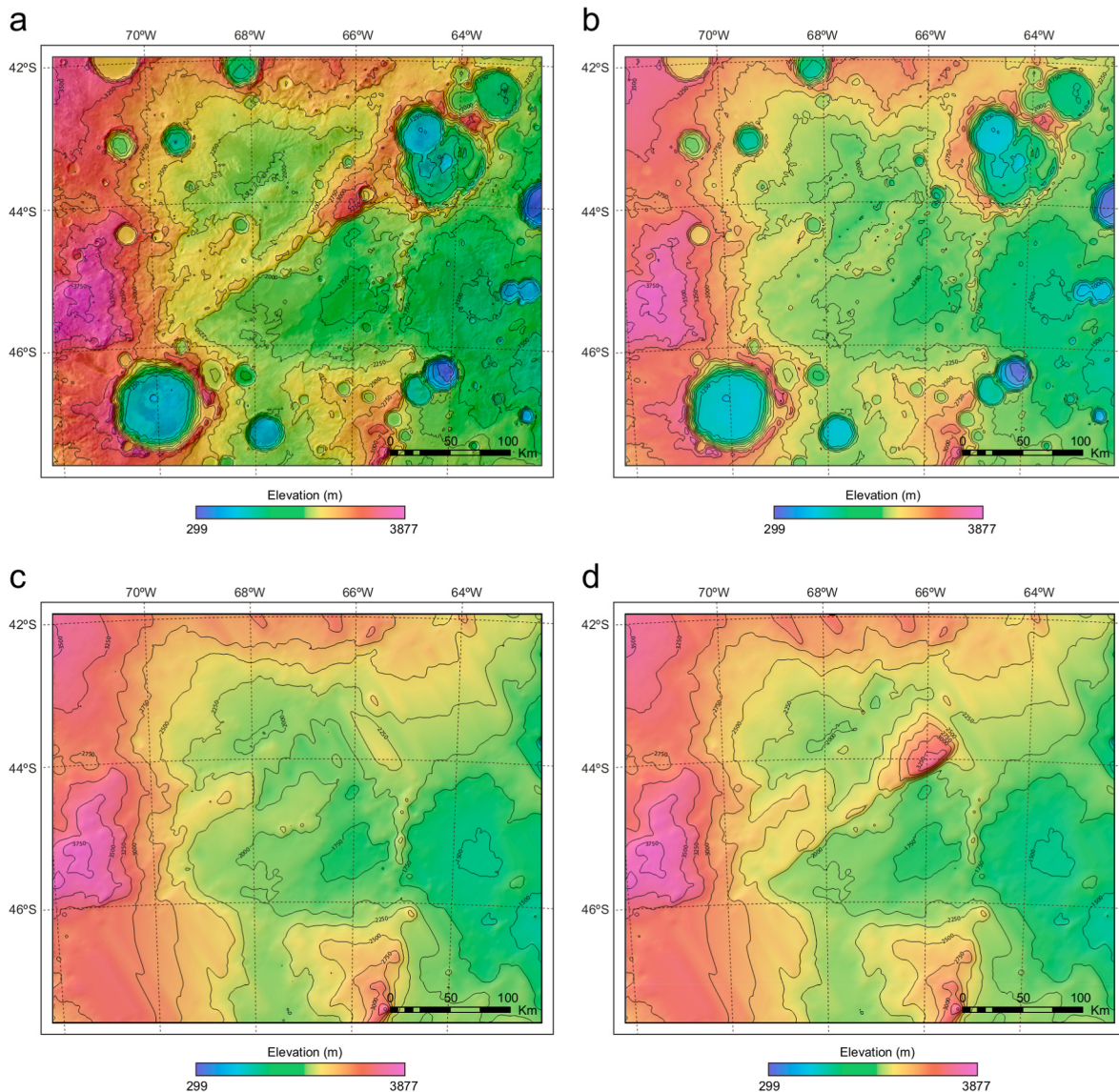
Fig. 8. Digital elevation models used and obtained during the modeling of Phraxi Rupes. a) Observed MOLA topography. b) Restored digital elevation model after the retrodeformation of the two modeled faults. c) Smooth digital elevation model where the relief caused by faults and impact craters has been removed (this topography was used as the starting stage for the 3D forward modeling). d) Digital elevation model obtained at the end of the forward modeling reproducing the main relief signatures associated with the faults observed in (a).
