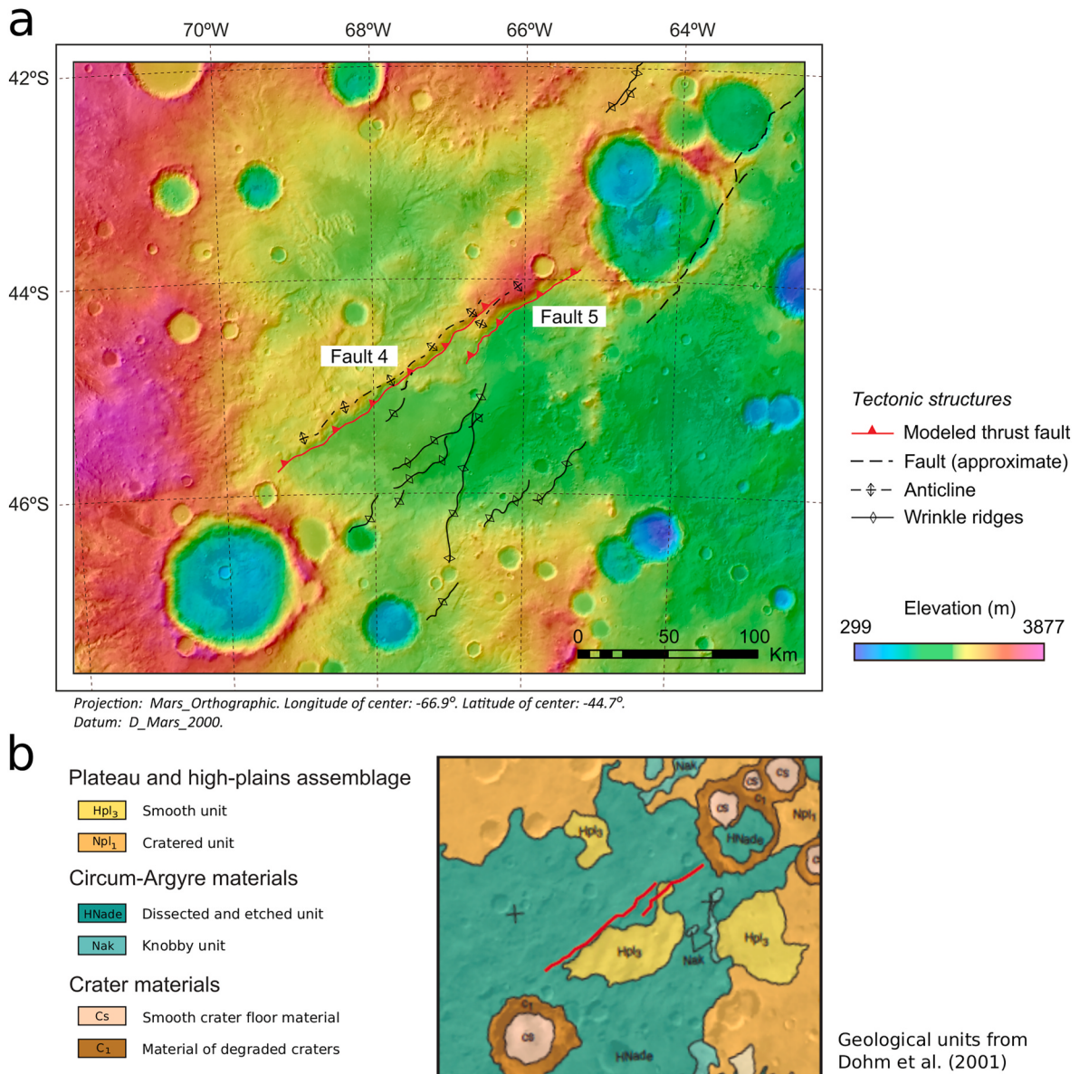
Fig. 7. (a) Structural map of the modeled thrust faults in Phrxi Rupes. The base map is made by combining a MOLA model (DEM) over a THEMIS-IR Day image. The modeled large thrust faults are labeled and marked in red. The fault-propagation anticlines generated on the hanging wall of every modeled thrust are mapped. Other minor faults and wrinkle ridges colored in black were not included in the models. (b) Geological units of the same area from Dohm et al. (2001) , the traces of the studied faults are marked in red. (For interpretation of the references to color in this figure legend, the reader is referred to the Web version of this article.)
