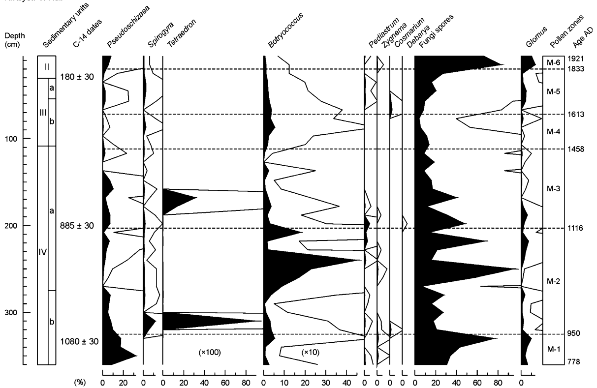
Fig. 6 Percentage diagram for non-pollen palynomorphs (NPP) with respect to the pollen sum. The scales of Tetraedron and Botryococcus have been reduced for more clarity. Solid lines indicate 10× exaggeration. Zonation as in Fig. 3
