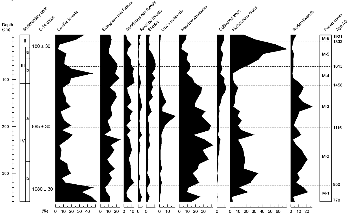
Fig. 5 Percentage pollen diagram grouped by vegetation types, according to Carreras et al. (2005–2006), with additional information from Muenscher (1980), Folch (1981), Vigo
