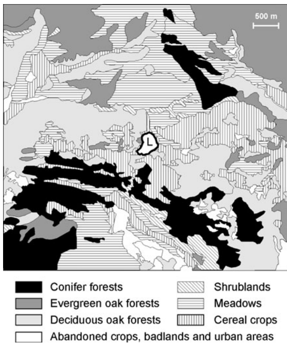
Fig. 2 Vegetation map according to the classification of Carreras et al. (2005–2006), using the CORINE system (CBM 1991). L, Lake Montcortès
