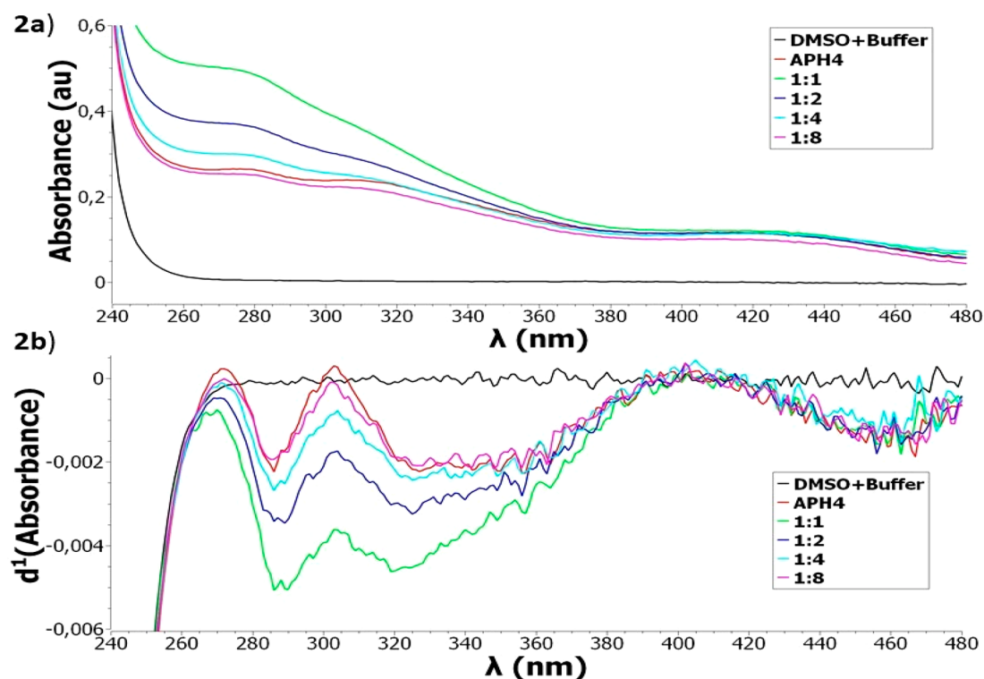
Figure 2. UV–vis spectra (a) and first-order derivative absorption spectra (b) of APH4 alone and in the presence of FeCl_2 in buffer (100 mM phosphate, pH= 7.30) at room temperature. [APH4] = 50 \mu\text{M} and [Fe^{2+}] = 50, 25, 12.5, and 6.25 \mu\text{M} , corresponding to stoichiometries 1:1, 1:2, 1:4 and 1:8, respectively.
