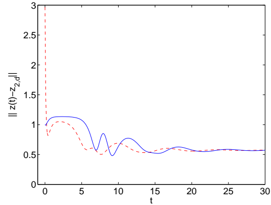
FIGURE 7. Graphic of \|z(t) - z_{2,d}\|_2 for (u_0, v_0) (—) and (u_6, v_6) (- - -).
