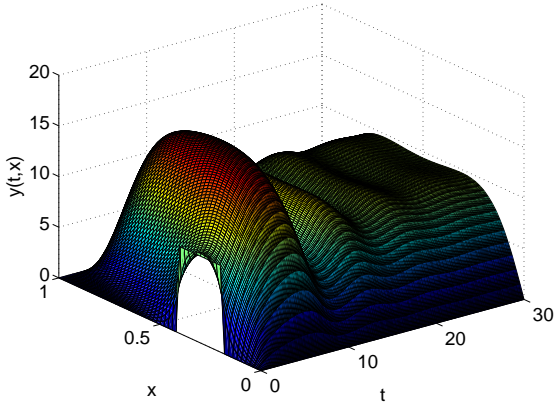
FIGURE 2. Graphic of y(t, x) when u = u_0 \equiv 8.56 on (0.2, 0.4) and v = v_0 \equiv 1.6379 on (0.6, 0.8) .
