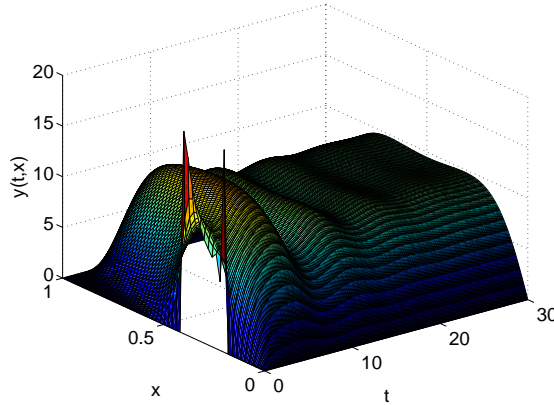
FIGURE 4. Graphic of y(t, x) when (u, v) = (u_6, v_6) are the computed Nash equilibrium on (0.2, 0.4) .
