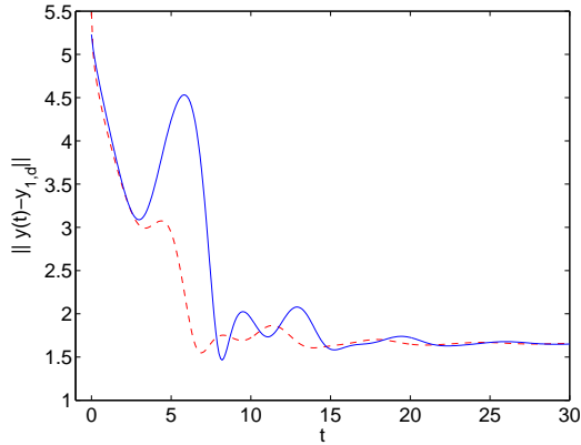
FIGURE 6. Graphic of \|y(t) - y_{1,d}\|_2 for (u_0, v_0) (—) and (u_6, v_6) (- - -).
