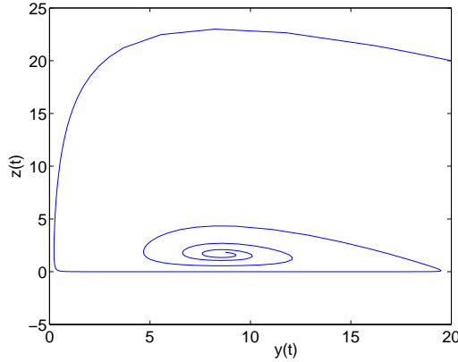
FIGURE 1. Phase diagram of the associated ODE system, for t \in [0, 30] .
