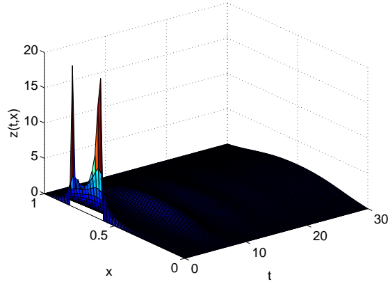
FIGURE 5. Graphic of z(t, x) when (u, v) = (u_6, v_6) are the computed Nash equilibrium on (0.6, 0.8) .
