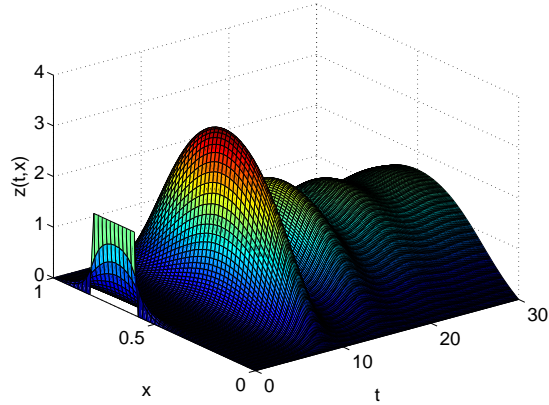
FIGURE 3. Graphic of z(t, x) when u \equiv 8.56 on (0.2, 0.4) and v \equiv 1.6379 on (0.6, 0.8) .
