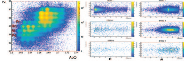
Fig. 1. – Left: particle identification plot obtained for our dataset. Middle (right): implantation profile of francium (astatine) isotopes in the three AIDA detectors.
