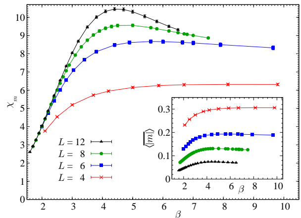
FIG. 8: As in figure 7, but p = 6 .
