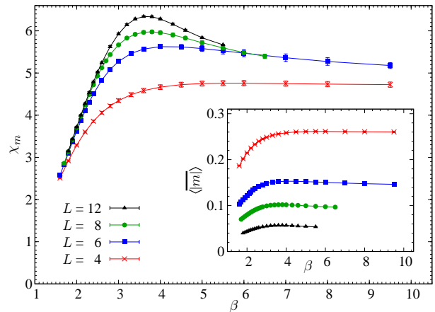
FIG. 7: Magnetic susceptibility as a function of \beta for L = 4, 6, 8 and 12 . Here p = 5 .
