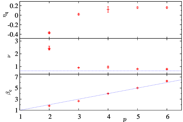
FIG. 9: In the bottom plot: \beta_c versus p , and the straight line f(p) = p . Middle plot: \nu as a function of p . We also show (dashed line) the value which marks the onset of a disordered first order phase transition ( \nu_{\text{first}} = 2/3 ). Upper plot: \eta_q as a function of p .
