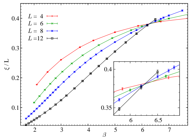
FIG. 6: As in figure 5, but p = 6 .
