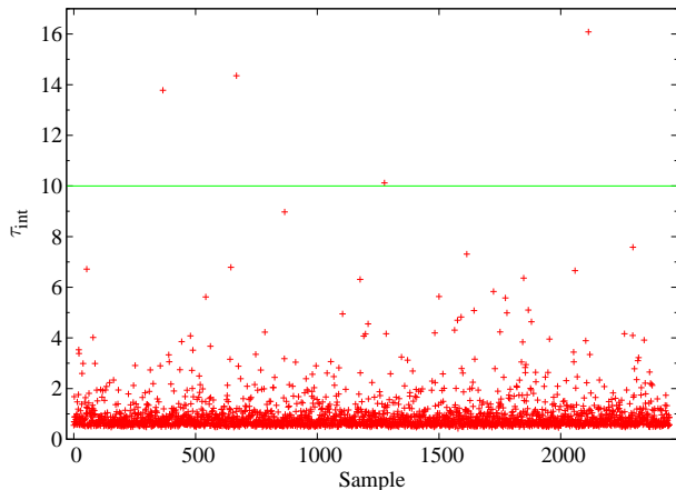
FIG. 4: Integrated autocorrelation time, \tau_{\text{int}} , for all p = 5 , L = 8 samples. \tau_{\text{int}} is in units of blocks of ten measurements, i.e. of 2010^3 MCS. Samples above the green line have been “extended” (see the text for a discussion of this issue).
