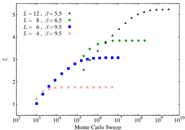
FIG. 1: Log-binning thermalization test for p = 5 . For all data points the point size is bigger than the corresponding error bar.
