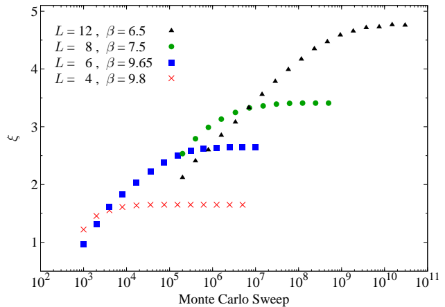
FIG. 2: As in figure 1, but p = 6 .
