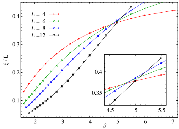
FIG. 5: Overlap correlation length in lattice size units as a function of the inverse temperature \beta for L = 4, 6, 8 and 12 . Here p = 5 .
