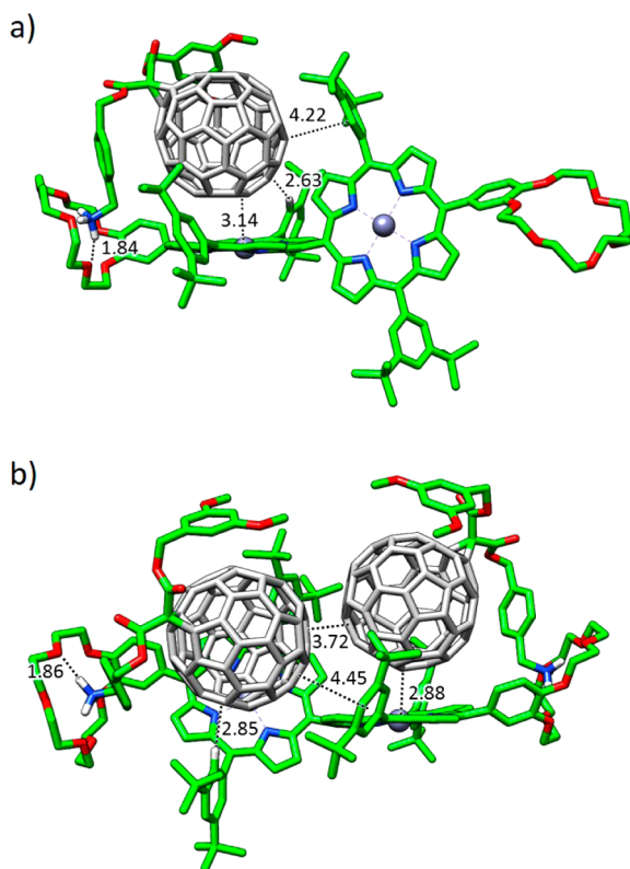
Figure 6. Minimum-energy geometry computed for supramolecular complexes [\mathbf{3}\cdot\mathbf{1}] (a) and [\mathbf{3}\cdot\mathbf{1}_2] (b) at the B97-D3/(6-31G**+LANL2DZ) level of theory. Selected intermolecular distances are given in Å. Hydrogen atoms are omitted for clarity.
