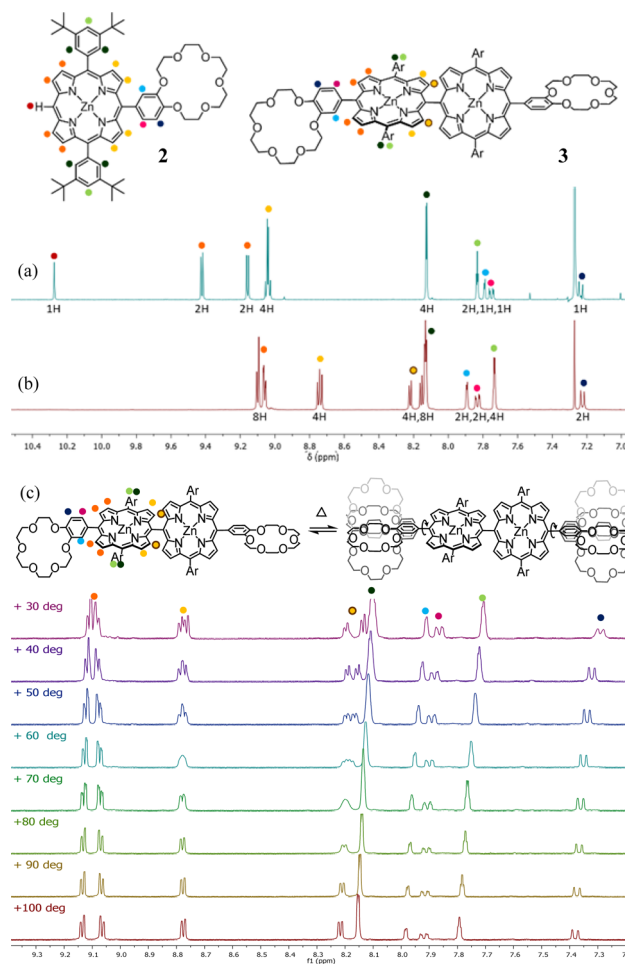
Figure 2. NMR characterization of compound 3 . ^1H NMR ( CDCl_3 , 400 MHz, 298 K) of monoporphyrin 2 (a) versus meso – meso dimer 3 (b) and (c) ^1H NMR variable temperature experiments ( ClCD_2CD_2Cl , 400 MHz, 30–100 °C).
