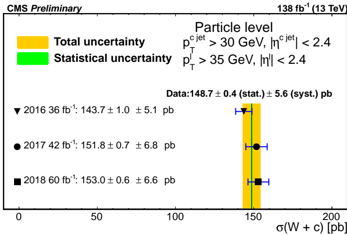
Figure 6.2: Comparison of the combined measurement of the fiducial \sigma(W + c) cross section unfolded to the particle level with the individual measurements obtained for each of the three years of data taking.
