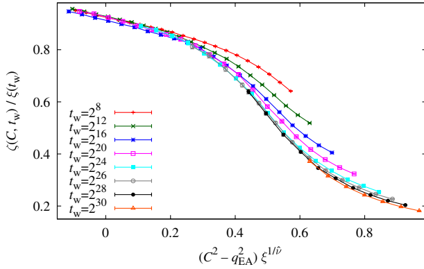
FIG. 4 (color online). Dimensionless ratio \zeta(C, t_w)/\xi(t_w) against the scaling variable (C^2 - q_{EA}^2)\xi(t_w)^{1/\nu} .
