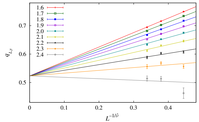
FIG. 3 (color online). Crossing points q_{L,y} for F_q/L^y computed from pairs of lattices ( L, 2L ), versus L^{-1/\hat{\nu}} , for different y values at T = 0.703 . The continuous lines are fits to Eq. (8), constrained to yield common values for q_{\text{EA}} and 1/\hat{\nu} .
