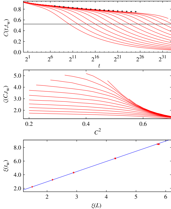
FIG. 1 (color online). Top: C(t, t_w) , Eq. (1), as a function of t for t_w = 4^i , i = 3, \dots, 16 (lines, t_w grows from bottom to top). We also plot \tilde{C}(t) (points) and our result for q_{EA} from Eq. (9) (horizontal line). Center: Correlation length \zeta(C, t_w) as a function of C^2 (same values of t_w as in the top panel). Bottom: Finite-time coherence length \xi(t_w) against the finite-size coherence length at q = 0 , \xi(L) . The results are compatible with \xi(t_w) = 1.48\xi(L) (straight line).
