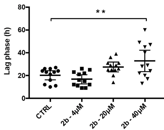
Fig. 9. Amyloid seeding assay. Prion protein fibril formation inhibitory activity in vitro for compound 2b. Each bar represents the average of n = 12 replicates from 4 independent experiments. Bars denote standard error and median value (** P < 0.005 ).
