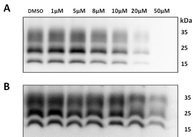
Fig. 8. Western Blot analysis of PrP Sc after 5 days of treatment with 2b in the ScN2a 22L cell line (A) or in ScGT1 22L (B). PK digested cell lysates were probed with D18 antibody. Molecular weight (in kDa) is represented on the right.
