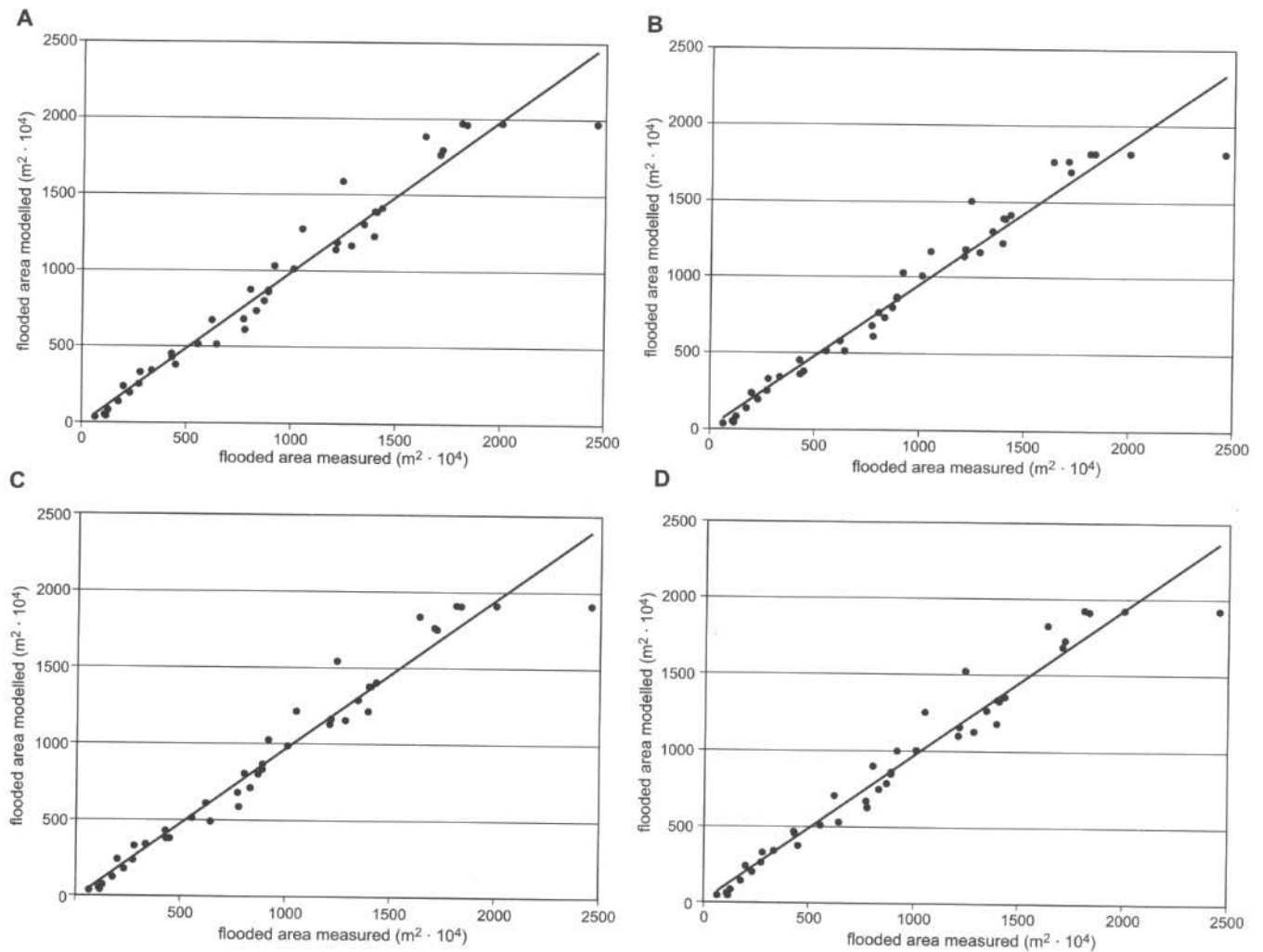
Fig. 3. Comparison between measured and calculated flooded surface values for the estimation of different parameters influencing Las Tablas de Daimiel water balance
