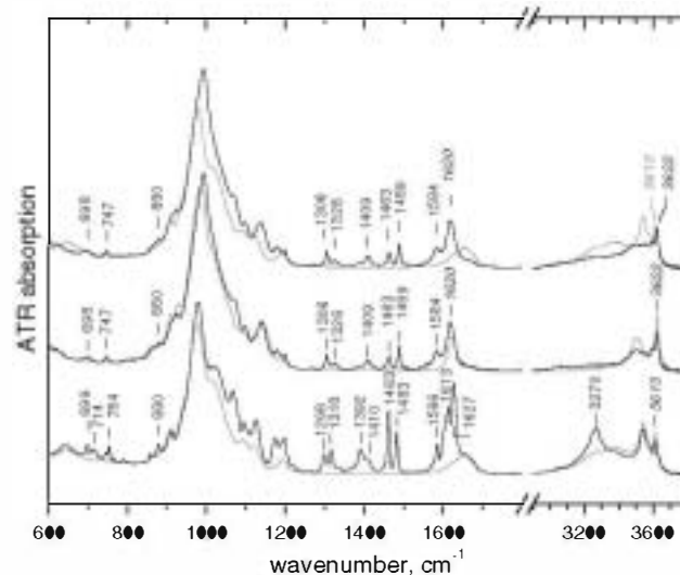
Fig. 6 ATR spectra of palygorskite (gray) and indigo-palygorskite 5 wt% mixture (black). Bottom: No thermal treatment, equilibrated to ambient conditions. Middle: Immediately after heat treatment at 130 \text{ }^\circ\text{C} overnight. Top: Heat-treated samples re-equilibrated to ambient conditions for 1 h
