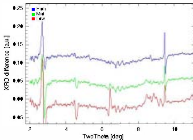
Fig. 7 Effect of possible rehydration of MB. The figure shows the differences between the averaged diffractogram during rehydration and the averaged diffractogram for low temperatures T < 90 °C (bottom), the averaged diffractogram for mid temperatures 90 < T < 130 °C (center), and the averaged diffractogram for high temperatures T > 130 °C (top)
