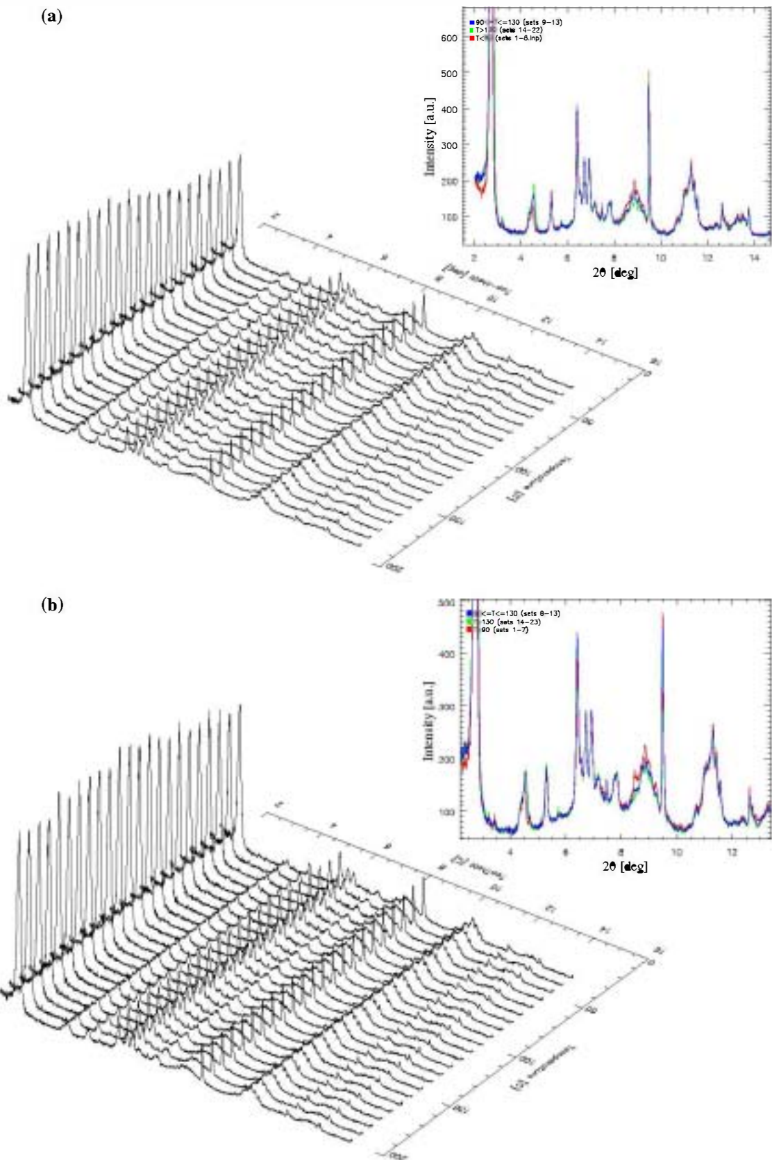
Fig. 2 X-ray diffractograms recorded as a function of the temperature for a polygorskite and b polygorskite-indigo mixture (1 wt% indigo). Insets: X-ray diffractograms averaged in three temperature ranges
