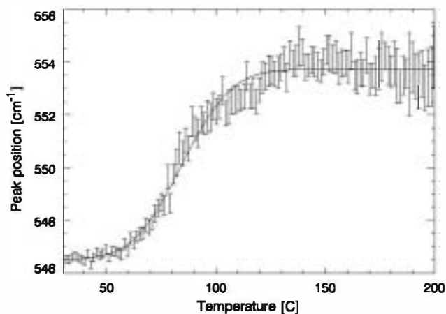
Fig. 5 Change in position versus temperature of the \delta\text{C}=\text{C}-\text{C}-\text{C} band for palygorskite and indigo (1 wt%)
