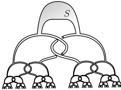
FIGURE 3. The sphere of Alexander
