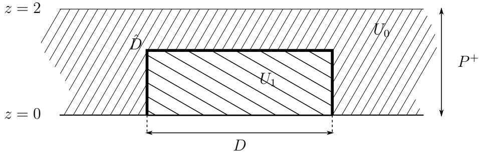
FIGURE 7. The construction of \hat{D}
