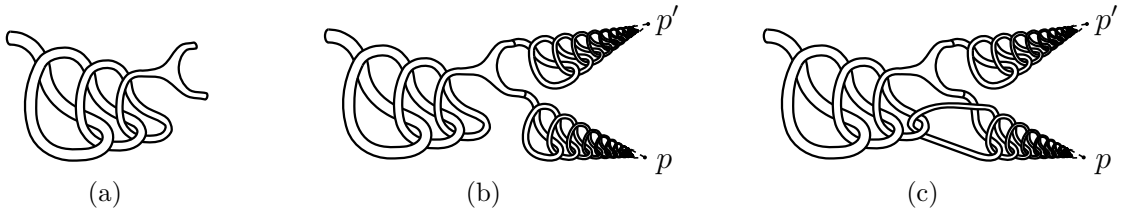
FIGURE 11. Branching a Fox–Artin feeler
