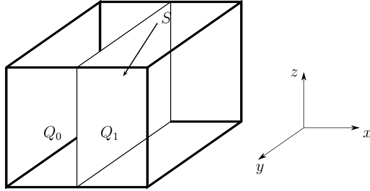
FIGURE 4. The setup for Definition 9
