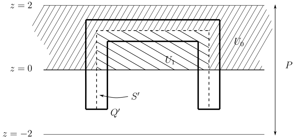
FIGURE 8. Scheme for Proposition 18
