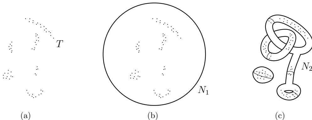
FIGURE 1. A totally disconnected set T and a couple of its neighbourhoods N_k
