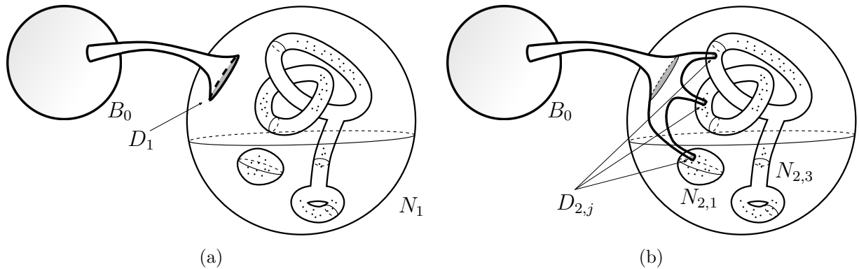
FIGURE 2. Modifying B_0 so that its boundary contains T
