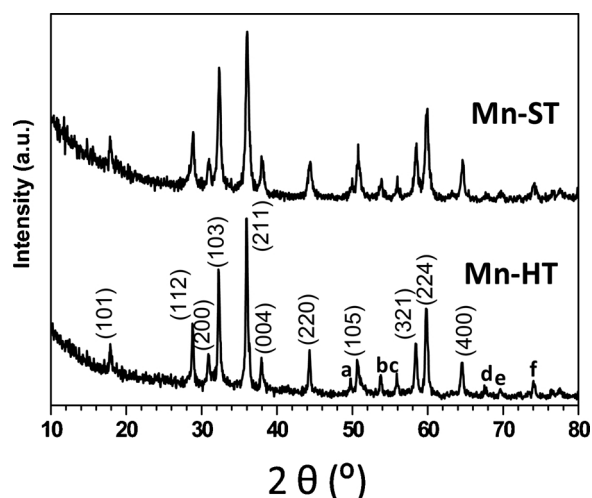
Fig. 4. XRD patterns of manganese oxide catalysts. In both cases the only phase detected is \text{Mn}_3\text{O}_4 . The small diffractions a, b, c, d, e and f correspond to (204), (312), (303), (402), (305) and (413), respectively.
