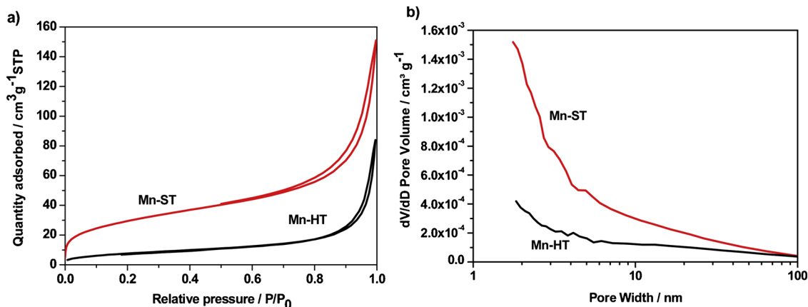
Fig. 3. a) N 2 adsorption/desorption isotherms and b) pore-size distributions for manganese catalysts.
