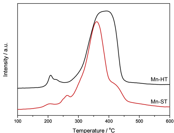
Fig. 6. H_2 -TPR for the manganese oxide catalysts.
