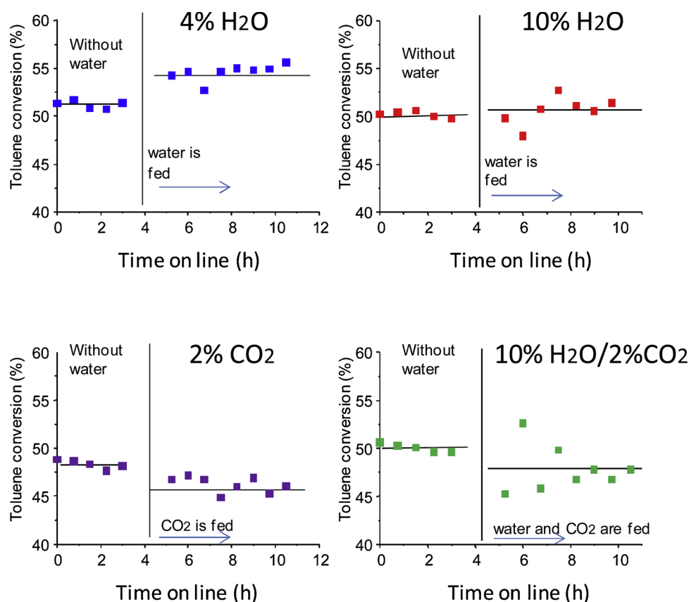
Fig. 2. Toluene conversion under different reaction feeds. Toluene concentration: 200 ppm. Reaction temperature: 125 °C. GHSV: 6000 h -1 .
