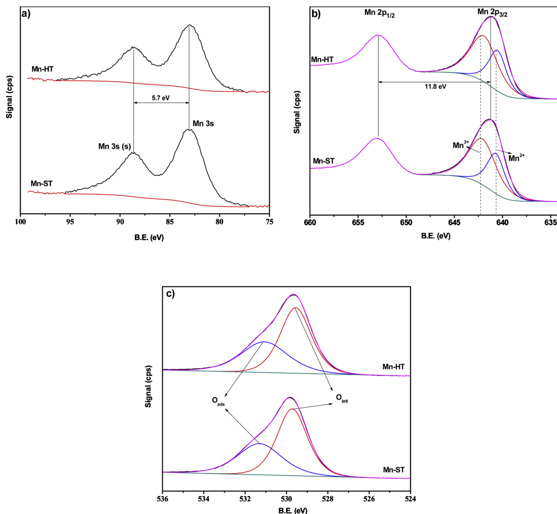
Fig. 5. XPS spectra of the (a) Mn 3s region, (b) Mn 2p region and (c) O 1s region of the manganese oxide catalysts.
