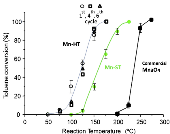
Fig. 1. Variation of the toluene conversion with the reaction temperature for manganese oxide catalysts. 200 ppm in synthetic air. GHSV = 6000 h -1 .
