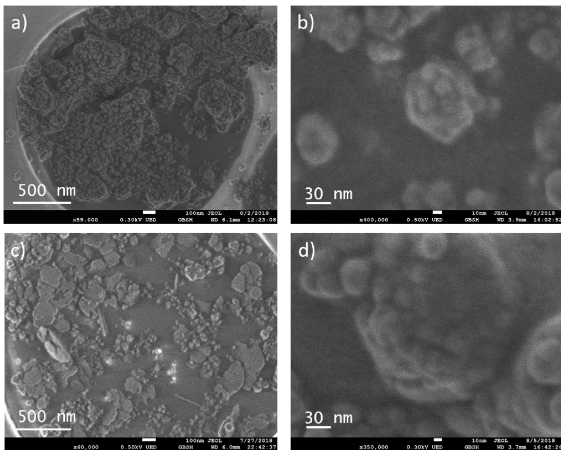
Fig. 9. SEM observations of Mn-ST, a) Low-magnification and b) High-magnification images. And Mn-HT c) Low-magnification and d) High-magnification images.
