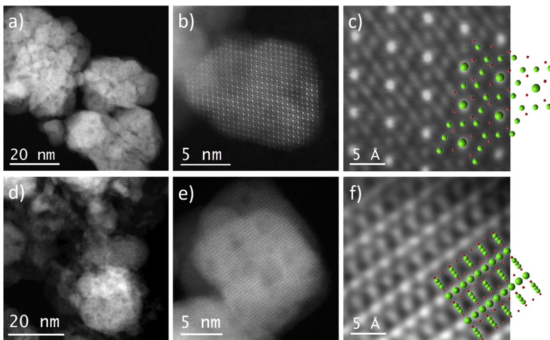
Fig. 7. C_s -corrected STEM-HAADF data. a) Low-magnification image showing several Mn-ST nanoparticles. b) High-resolution image of a Mn-ST isolated nanoparticle along the [111] zone axis. c) A closer look of the structure of the Mn-ST nanoparticle with the model superimposed. d) Low-magnification image of Mn-HT material. e) An isolated Mn_3O_4 -HT nanoparticle along the [011] orientation. f) Enlarged image of the particle shown in e) with the model superimposed. Green spheres correspond to the Mn while O atoms appear as red spheres.
