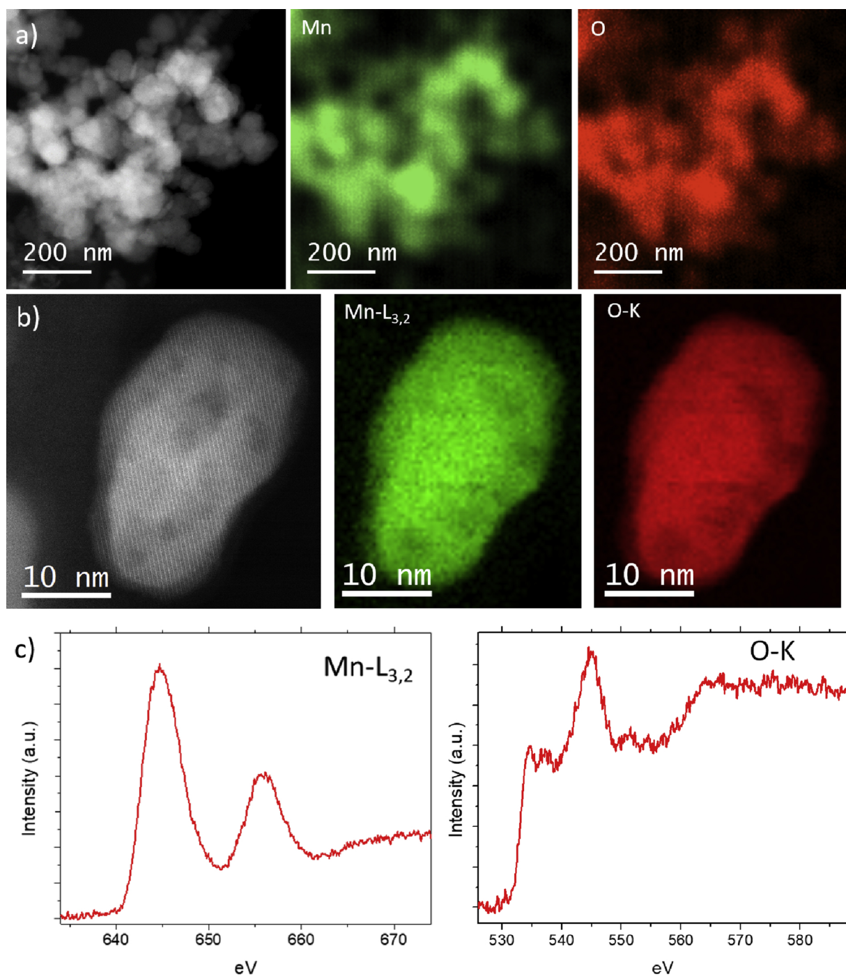
Fig. 8. Study by TEM of Mn-HT catalyst. a) EDS mapping analysis of several nanoparticles which confirms the presence of Mn (green map) and O (red map). b) EEL spectrum image of a Mn-HT nanoparticle showing the perfect concordance between the Mn and O. c) EEL spectra of the signals extracted corresponding to Mn and O edges respectively.
