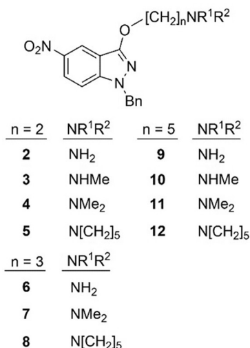
Fig. 2. Structures of 3-( \omega -aminoalkoxy)-1-benzyl-5-nitroindazoles prepared and studied in this work.
